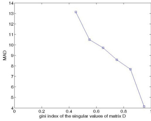
Fig. 11. MAD performance with respect to different gini values of singular values of the matrix D .
