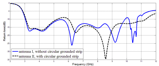
Fig. 8. Simulated reflection coefficient of the antenna I and antenna II, with L_s=18.8 .
