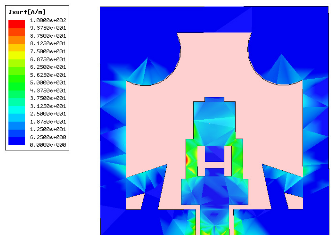
Fig. 13. Simulated current distribution of the proposed antenna at 5.45 GHz.
