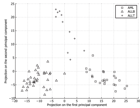
(a) K-means
