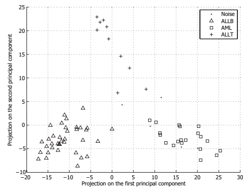
(c) QT
