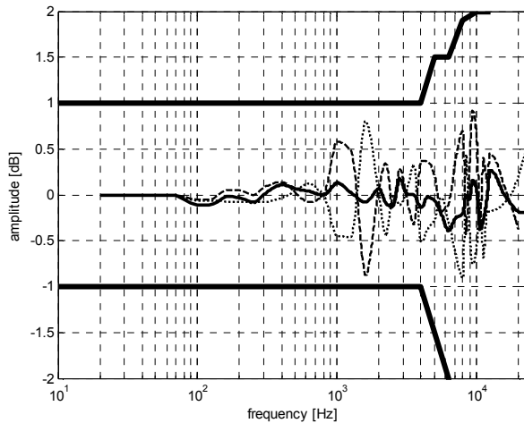
Fig. 6. The characteristics before the compensation (dashed line) and after the compensation (solid line); the characteristics of the compensation filter dotted line) and the tolerance limits (thick lines).
