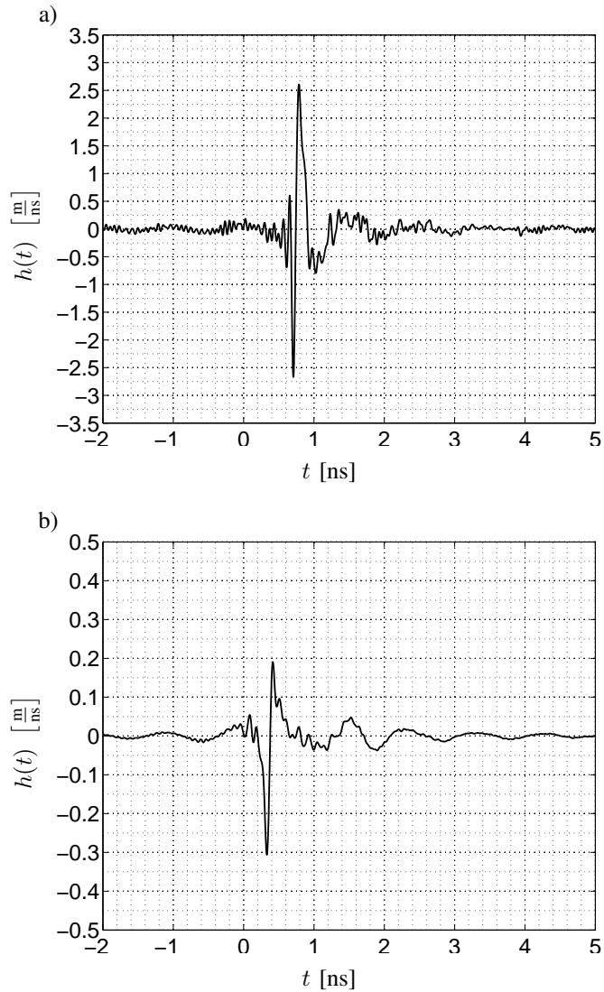
Fig. 6. Pulse response measured in frequency band: 1 ÷ 18 GHz: a) the TEM horn П16-23, b) the planar Vivaldi antenna.
