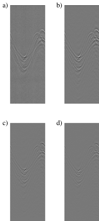
Fig. 8. Raw measurement data (echogram): a) pre-processed; b) pre-processed and bandpas filtered ;c) pre-processed after deconvolution of the receiving antenna's pulse response; d) pre-processed and after deconvolution of the waveform h_{tot}(t) .
