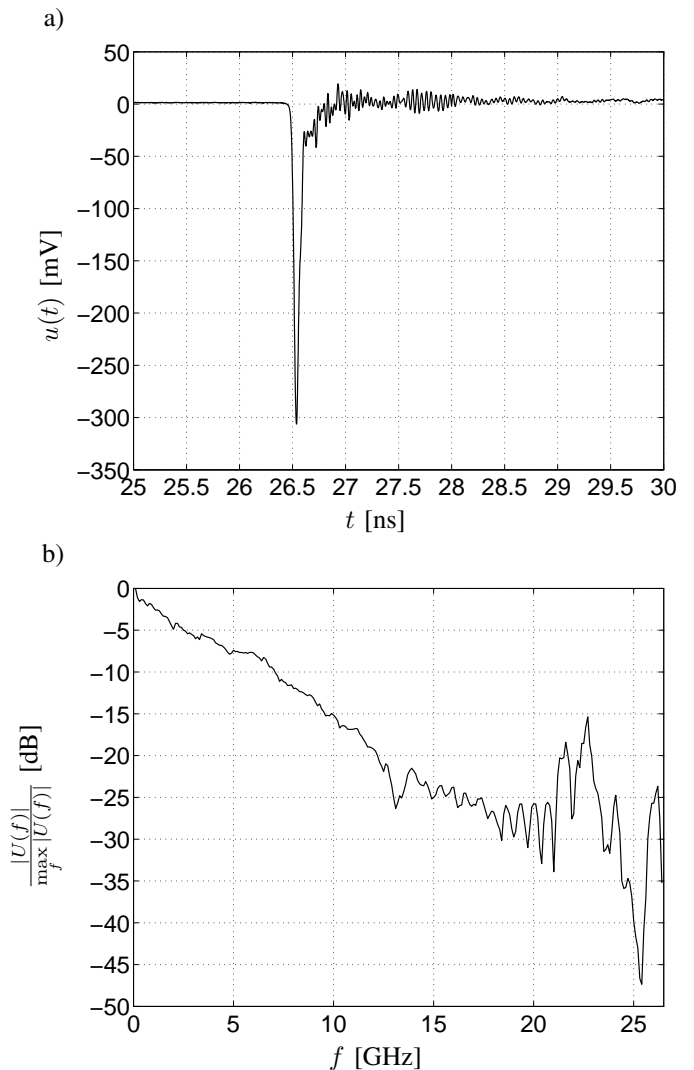
Fig. 2. Measurement pulse: a) waveform, b) amplitude spectrum.
