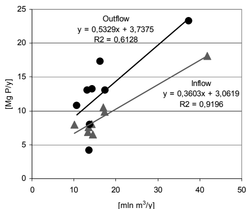
Fig. 4. Correlation between the amount of entering and leaving water and phosphorous load in the Plawniowice reservoir in the period 2004–2011
