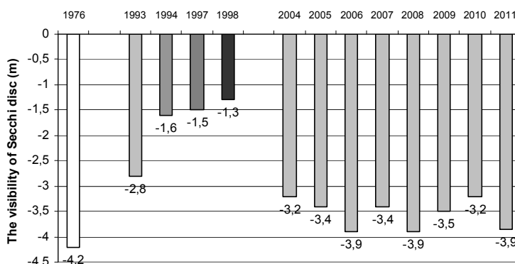
Fig. 8. The Secchi disc visibility in the summer stagnation periods in the period 1976–2011
