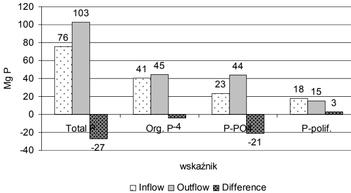
Fig. 5. The overall balance of the different forms of phosphorous, Plawniowice reservoir 2004–2011
