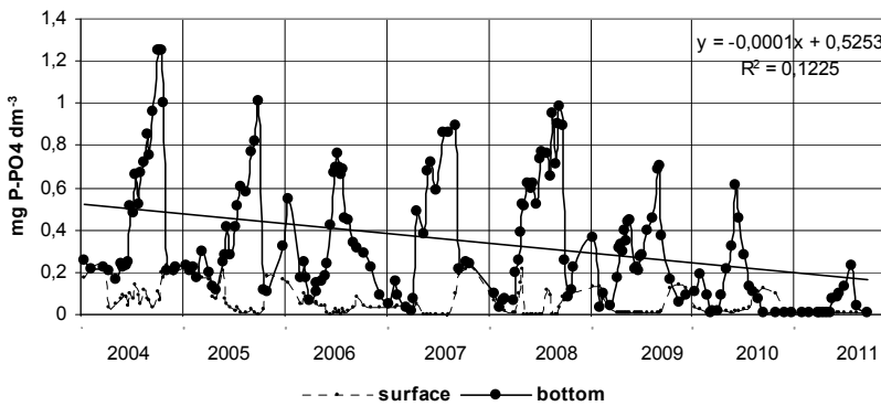
Fig. 6. Changes of phosphates concentration in the period 2004–2011
