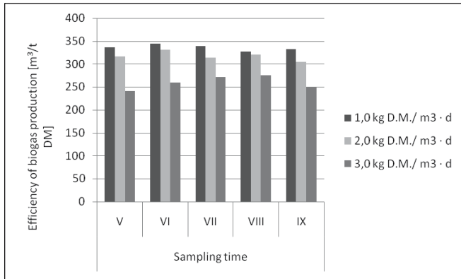
Fig. 1. Efficiency of biogas production depending on the applied load
