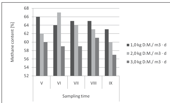
Fig. 2. Methane content in biogas depending on the applied load
