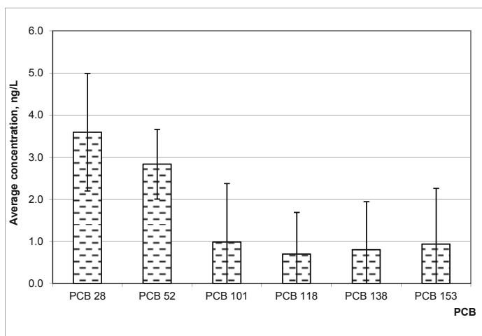
Fig. 5. The average concentration of PCBs in supernatants
