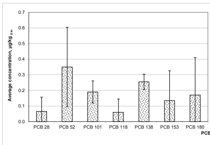
Fig. 4. The average concentration of PCBs in sewage sludge
