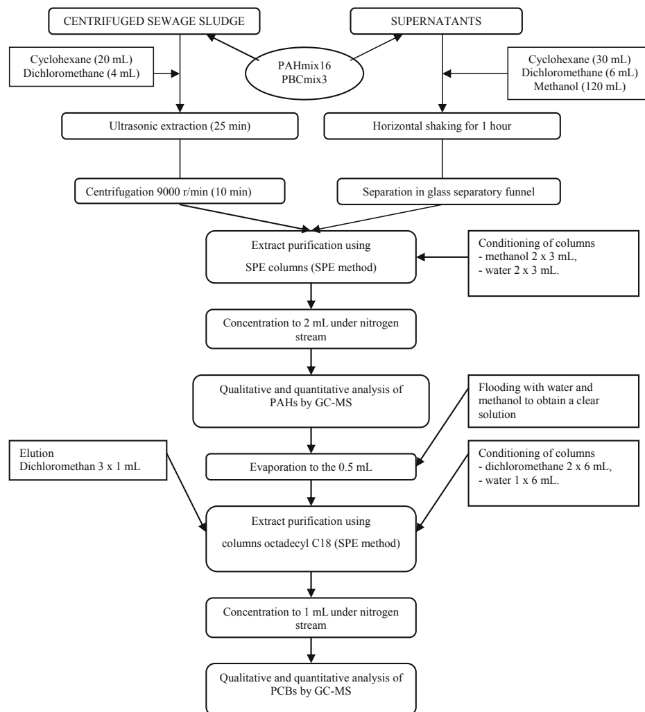
Fig. 1. Diagram of sample preparation of sewage sludge and supernatants to the common determination of PAHs and PCBs
