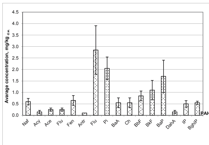
Fig. 2. PAHs concentration in coke sludge
