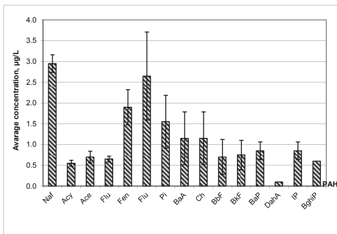
Fig. 3. PAHs concentration in supernatants
