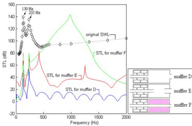
Fig. 8. Comparison of the original SWL (hybridized with two pure tone – 130 Hz and 235 Hz) with respect to the STL at various mufflers [muffler D; a two-chamber HR element and a one-chamber simple expansion element; muffler E; a two-chamber HR element and a one-chamber tube-extended element; muffler F; a two-chamber HR element and a one-chamber dissipative element].
