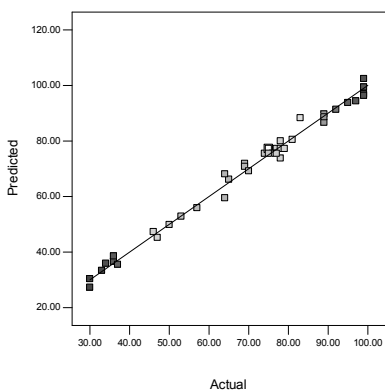
Fig. 1. a: Predicted vs. actual values of nickel extraction %, b: Normal plot of residual for nickel extraction
