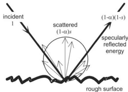
Fig. 1. Definition of the sound scattering coefficient (COX, DALENBACK, 2006).
