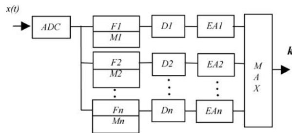
Fig. 5. Garland of n MFs with one ADC .
