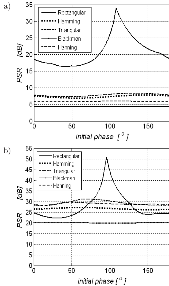
Fig. 1. PSR dependence on the initial phase for different windows when the chirp parameters are: f_1 = 0 , f_2 = 15 MHz, \tau_i = 2.5 \mu\text{s} , BT = 37.5 , optimal f_s = 30.2 MHz: a) without nonlinear operations; b) with nonlinear operations. In both cases the main lobe consists of one sample.
