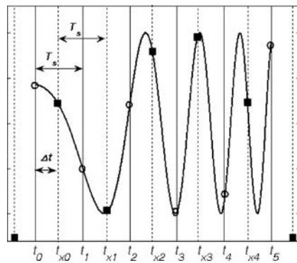
Fig. 3. Example of divergence between a signal sample and moments of MF IR weight factor determination. Here: \circ – moments of the weight factors determining; \blacksquare – signal samples.
