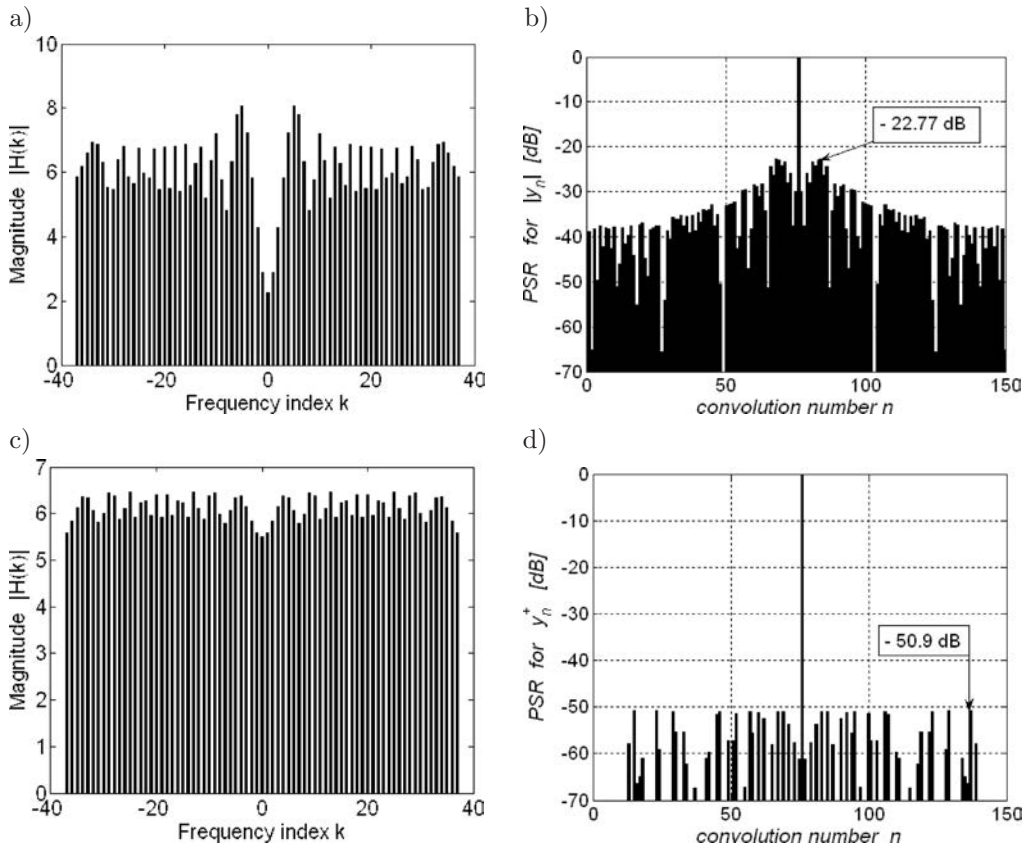
Fig. 2. a) Amplitude spectrum of unmatched IR to the rectangular window when \varphi_0 = 30^\circ , f_s = 30 MHz, D_H = 1.0765 ; b) result of the chirp compression with the use of this IR and without any nonlinear operations; c) amplitude spectrum of the matched IR to the rectangular window when \varphi_0 = 96^\circ , f_s = 30.2 MHz and minimized D_H = 0.0711 ; d) result of the chirp signal matched filtering with the use of this IR and nonlinear operations. The chirp parameters are: f_1 = 0 , f_2 = 15 MHz, \tau_i = 2.5 \mu\text{s} , BT = 37.5 .
