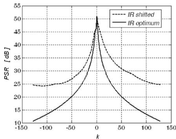
Fig. 4. Dependence of PSR on delay \Delta t = \pm kT_s/128 for the chirp parameters: f_1 = 0 , f_2 = 15 MHz, \tau_i = 2.5 \mu s, \varphi_0 = 96^\circ , f_s = 30.2 MHz. Maximal divergence: \Delta t = T_s/256 = 0.12935 ns.
