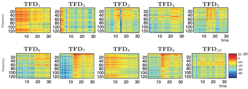
Fig. 13. \mathbf{TFD}_i components, for 80% of signal variance. The scales for all \mathbf{TFD}_i range from 0 through 129, which corresponds to the frequency range from 0 through 4 kHz. The range 0–30 in the time scale corresponds to the range 0–0.51 s. Similarities of \mathbf{TFD}_i elements with the constituent sounds of the mixed signals can be clearly seen. For example, \mathbf{TFD}_1 , \mathbf{TFD}_2 and \mathbf{TFD}_8 belong to “ringer”, \mathbf{TFD}_5 , \mathbf{TFD}_7 and \mathbf{TFD}_9 belong to “tom” and other components belong to “baby”.
