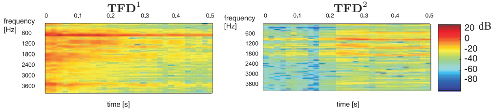
Fig. 7. \mathbf{TFD}^i components obtained with an algorithm maximising the sum of their negentropies. The variance \varphi = 90\% of the mixed signal was used. \mathbf{TFD}^1 – the spectrogram of “ringer”, \mathbf{TFD}^2 – the spectrogram of “baby” (0.51 s of the mixed signal of Fig. 1 was analysed).
