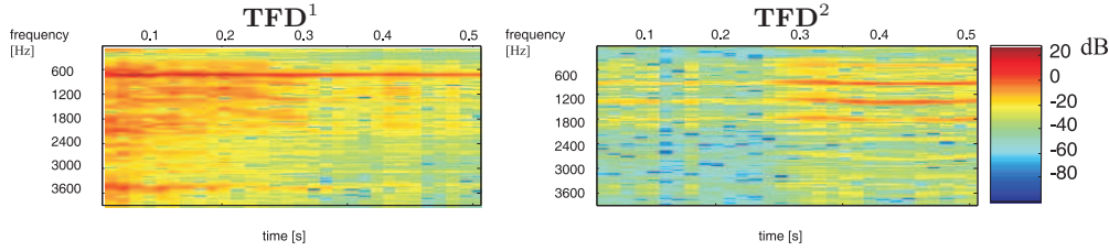
Fig. 6. Reconstructed components of the mix obtained by hierarchical clustering with the use of Euclidean distance for t-f components \mathbf{TFD}_i . \mathbf{TFD}^1 – the part of the spectrogram of S_1 (“ringer”) corresponding to the first 0.51 s of this signal, \mathbf{TFD}^2 – the spectrogram of “baby”. The harmonic structure corresponding to the original spectra of Fig. 1 can be clearly seen.
