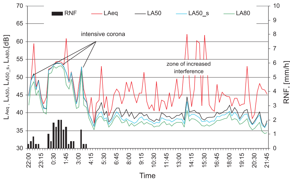
Fig. 5. Plots of the L_{Aeq} level and the statistical levels for the corona acoustic signal – L_{A80} , L_{A50} , and L_{A50_s} ( A -weighted level determined from the statistical spectrum L_{50} ) and rainfall intensity (RNF).
