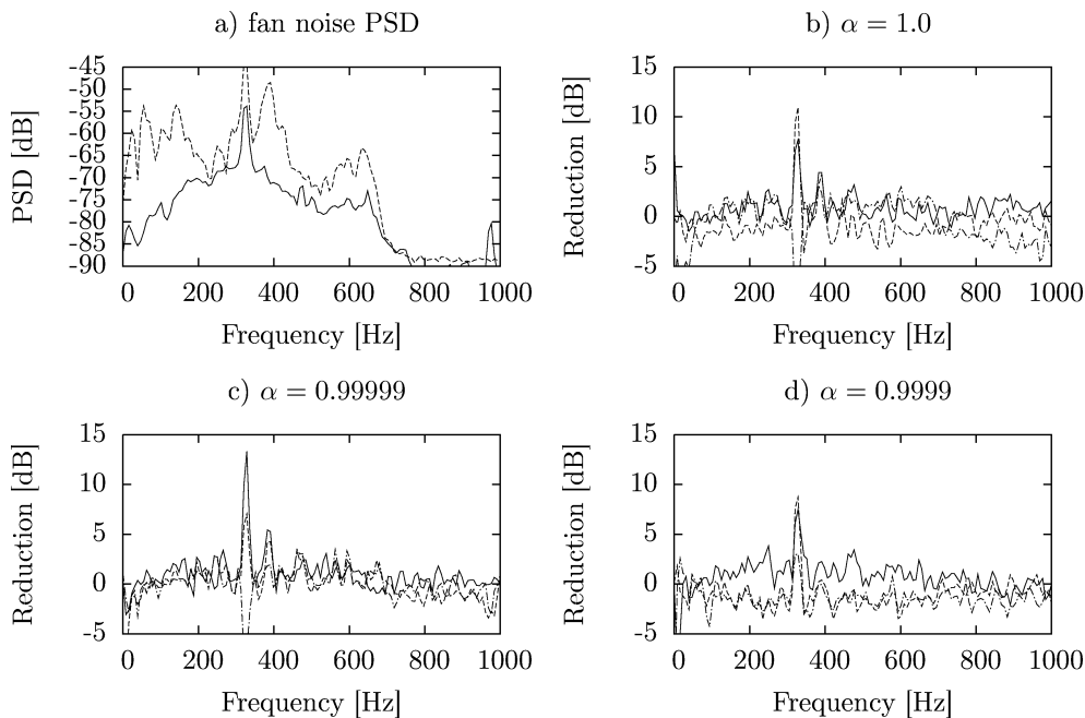
Fig. 10. a) Power Spectral Density of the signal for the primary noise loudspeaker (solid) and the primary noise at error microphone (dashed); b), c), d) The results of fan noise reduction for 28^{\circ}\text{C} for different values of parameter \alpha for a model identified just before experiment (solid line), for the same temperature before heating and cooling (hashed line), for ambient temperature 24^{\circ}\text{C} (dash-dotted).
