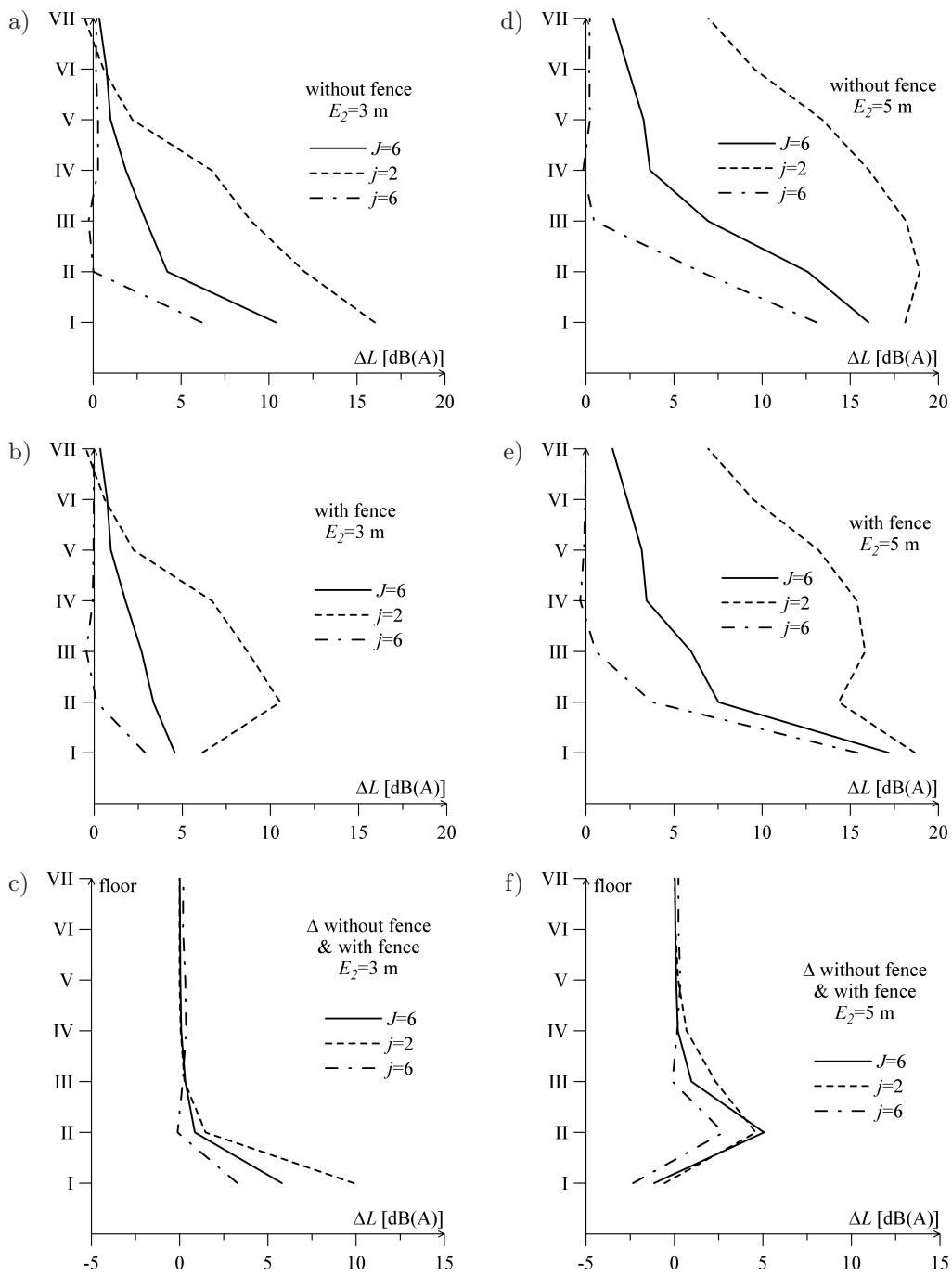
Fig. 6. The efficiency of the protecting screen E_2 = 3 m: a) without a fence, b) with a fence, c) the effect of a fence, and the efficiency of the protecting screen E_2 = 5 m: d) without a fence, e) with a fence, f) the effect of a fence.
