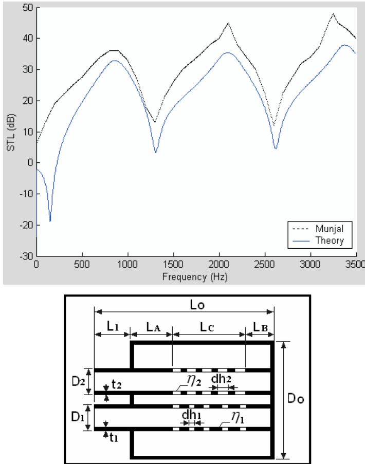
Fig. 5. Performance of a one-chamber reverse-flow perforated muffler [ D_1 = 0.0493 (m), D_2 = 0.0493 (m), D_o = 0.1481 (m), L_A = L_B = 0.0064 , L_c = 0.1286 (m), t_1 = t_2 = 0.0081 (m), dh_1 = dh_2 = 0.0035 (m), \eta_1 = \eta_2 = 0.039 , M_1 = 0.1 ] [analytical data is from MUNJAL et al. (1975)].
