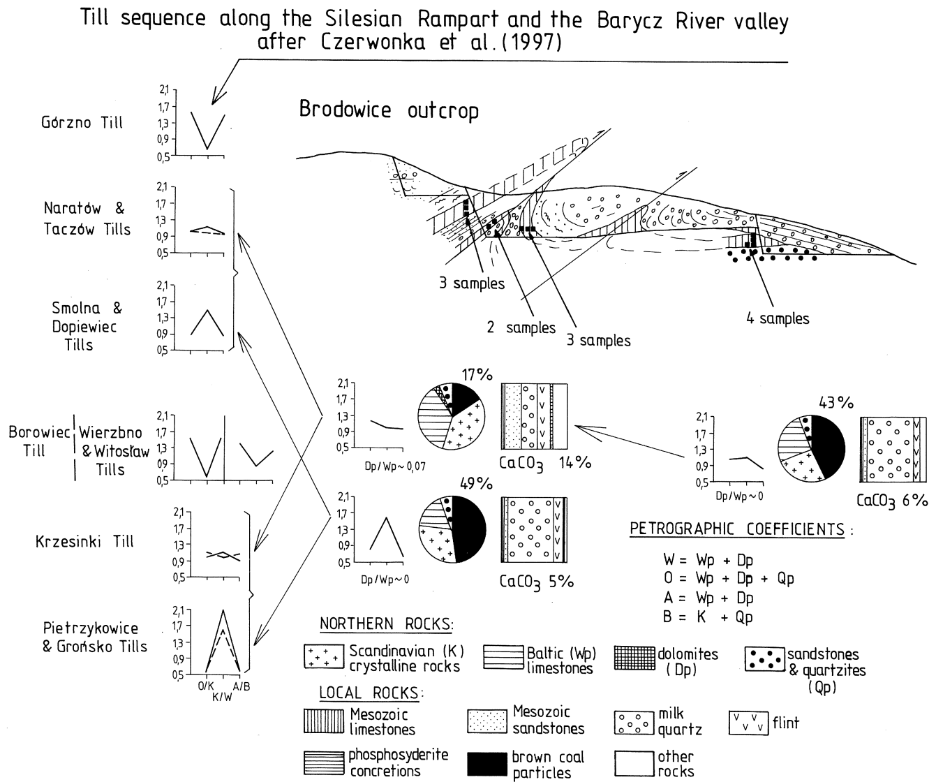
Fig. 10. Petrographic composition of tills at Brodowice outcrop and their correlation with till in the region (arrows indicate possible interpretations; detailed discussion in the text)
