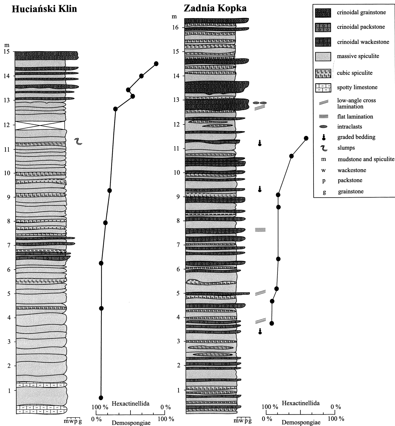
Fig. 3. Lithological sections of the spiculite series at the Huciański Klin crest and Zadnia Kopka hill, with changes in proportions of Hexactinellida and Demospongiae spicules
