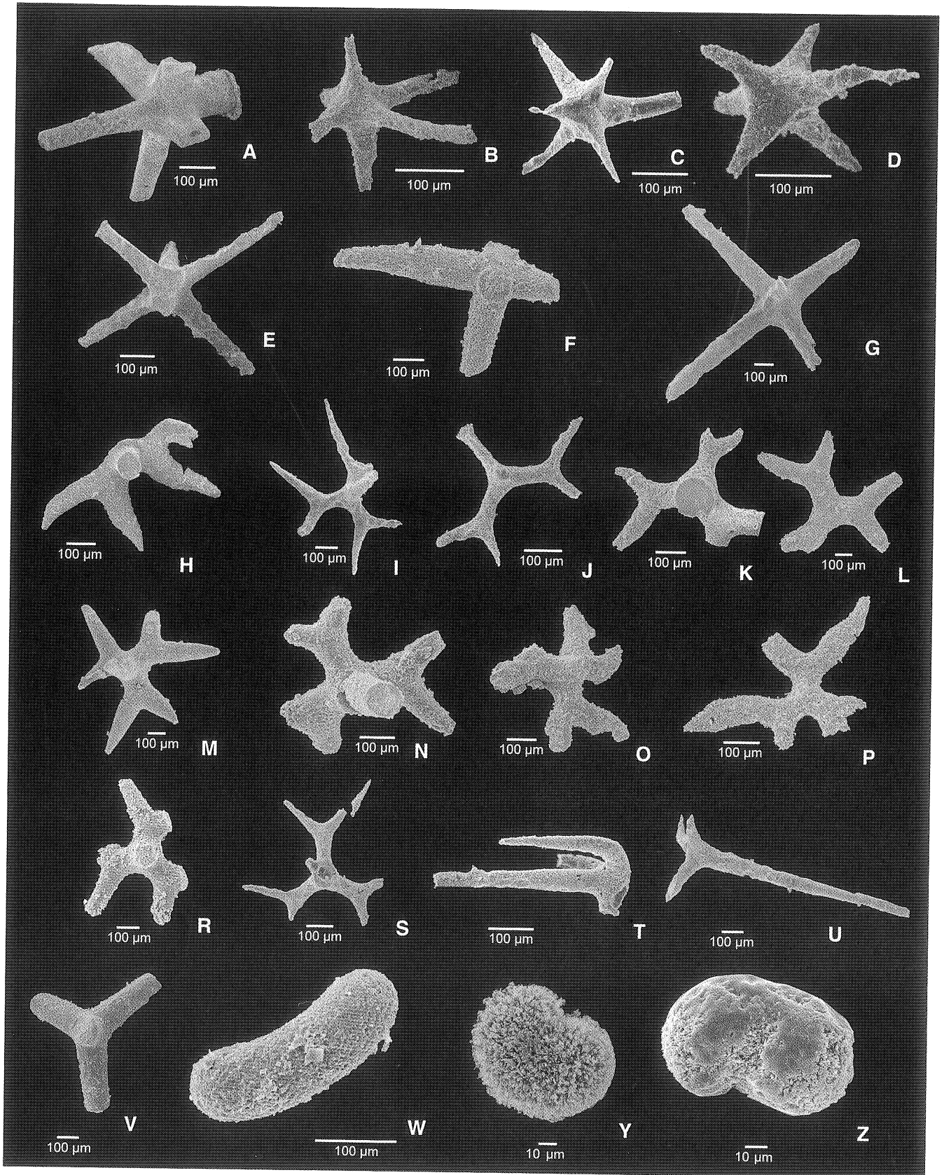
Fig. 8. Selected spicules isolated by etching in HF. Hexactinellid spicules: A–G. hexactines; Demosponge spicules: H–S. dichotriaenes; T. atriaene; U. triaene; V. tetractine; W. strongyle; Y–Z. selenasters
