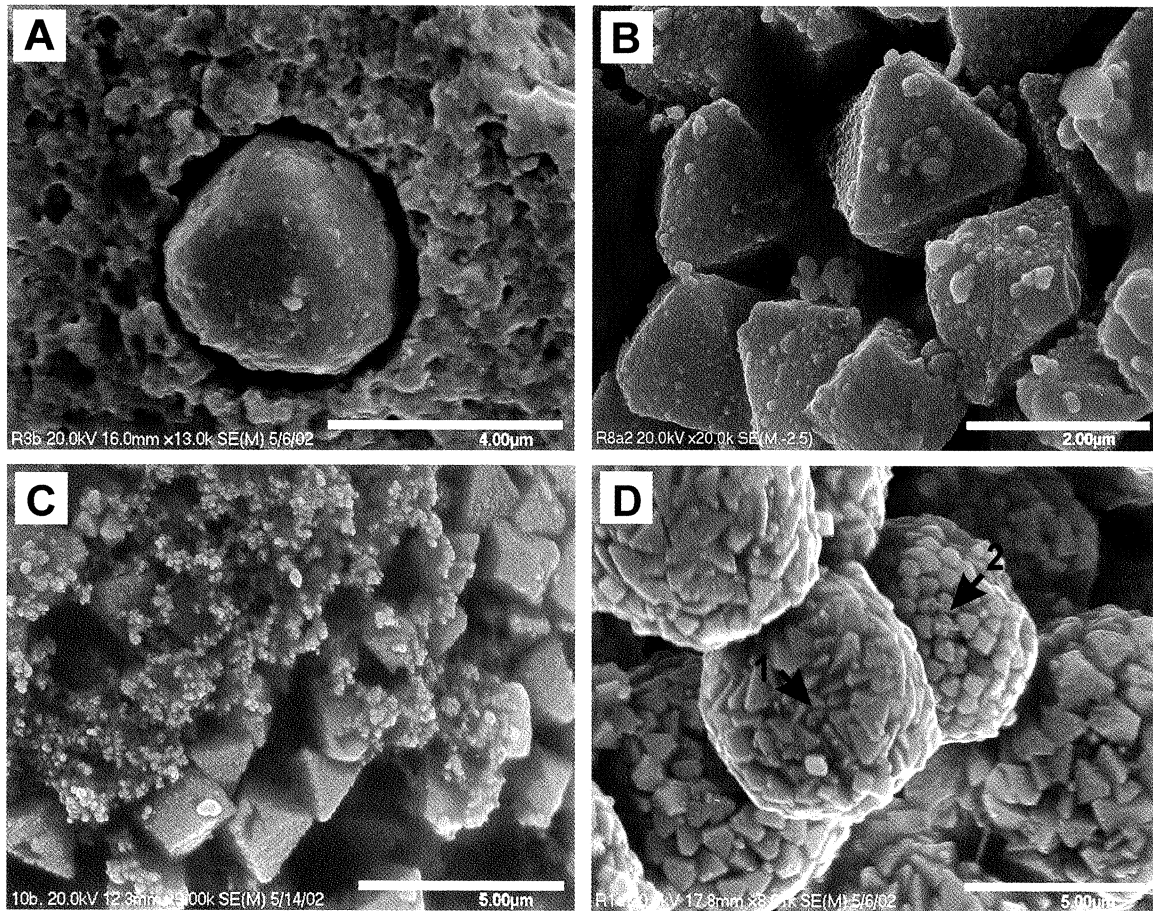
Fig. 3. Examples of pyrite from pyritized radiolaria. A – pyrite euhedra (possibly recrystallized framboid) in a pore of pyritized H. barbui (scale bar 4 \mu\text{m} ); B – octahedral microcrystals of pyrite framboid from the abdomen of pyritized H. barbui (note that microcrystals are built of smaller subunits ranging from 50 to 100 nm – crystal-like microframboid sensu Sawłowicz, 1993; scale bar 2 \mu\text{m} ); C – pyrite octahedral microcrystals (see Fig. 3B) encrusted by minute (200–300 nm) pyrite grains (abdomen of pyritized H. barbui ; scale bar 5 \mu\text{m} ); D – pyrite framboids built of closely packed (1) and strongly intergrown microcrystals (2) (pyritized H. barbui ; scale bar 5 \mu\text{m} )
