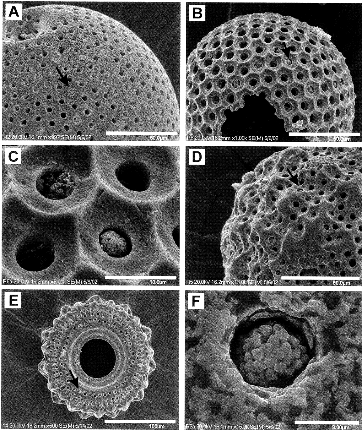
Fig. 1. Examples of frambooids from pyritized radiolaria. A – pyritized radiolarian skeleton ( Holocryptocanium barbui Dumitrica) with pyrite frambooids visible in the uppermost parts of pores (scale bar 50 \mu\text{m} ); B – pyrite frambooids visible in lower parts of pores (arrow, compare with Fig. 1A) of the uncovered by erosion outermost layer of pyritized radiolarian skeleton of H. barbui (scale bar 50 \mu\text{m} ); C – pyrite frambooid and irregular cluster of pyrite crystals in pores of pyritized H. barbui (magnified fragment of Fig. 1B; scale bar 10 \mu\text{m} ); D – pyritized radiolarian skeleton ( Holocryptocanium tuberculatum ) with pyrite frambooids visible in pores (scale bar 50 \mu\text{m} ); E – pyrite frambooids visible in the last chamber of pyritized Xitus mclaughilini Pessagno (scale bar 100 \mu\text{m} ); F – pyrite frambooid with intergrown microcrystals in a pore of pyritized skeleton of H. barbui (scale bar 3 \mu\text{m} )
