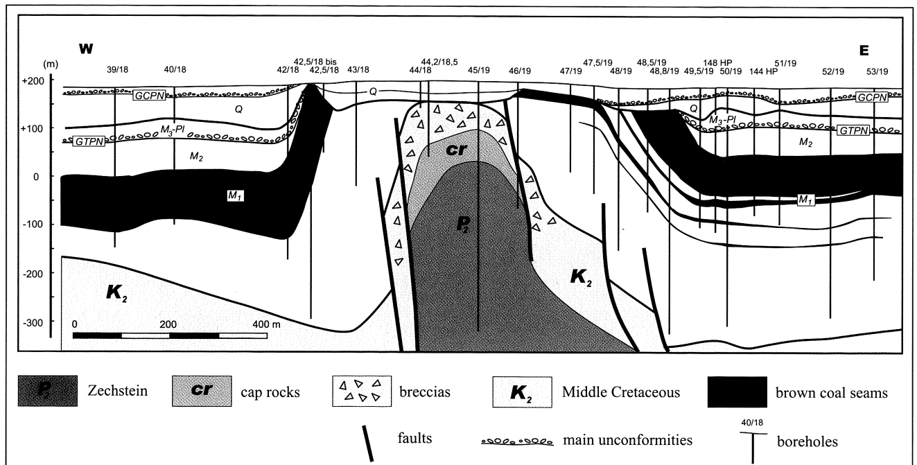
Fig. 3. Geological section across the Dębina Salt Dome area, two times exaggerated. Q – Quaternary; M 3-Pl – Late Miocene to Pliocene; M 2 – Middle Miocene; M 1 – Early Miocene; GCPN – main Quaternary unconformity; GTPN – main Tertiary unconformity
