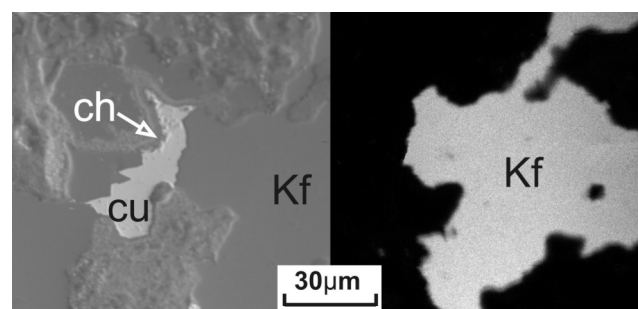
Fig. 9. Back scattered electron image of the intergrowing crystals native copper – K-feldspar (left) and K beam (Kα) image of K-feldspar (right); cu – native copper; Kf – K-feldspar, ch – chlorite
