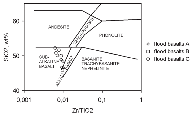
Fig. 6. Basalts of the Volhyn series of the Zhyrychi deposit and Rafalovka-Berestovets field on the \text{SiO}_2 - \text{Zr/TiO}_2 diagram (Winchester, Floyd, 1977)
