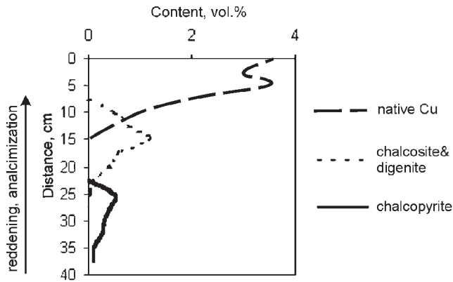
Fig. 11. Vertical profile of Cu mineral distribution in the reddened and analcimized green tuff of the Zhyrychi deposit
