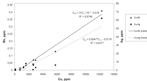
Fig. 7. Cu versus Ag and Rh in the ores of the Zhyrychi deposit
