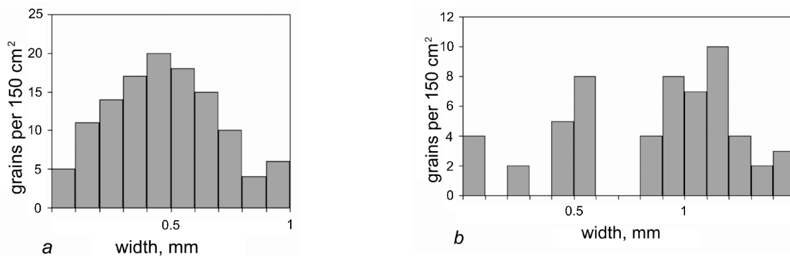
Fig. 15. Size distribution of native copper blebs in green (a) and red (b) tuffites
