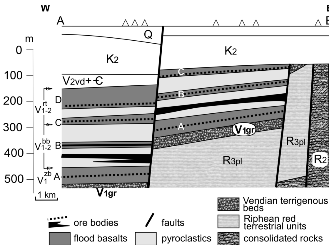
Fig. 4. Geological section of the Zhyrychi deposit. A, B, C, D – lava floods (see Fig. 5 for symbol explanation)
