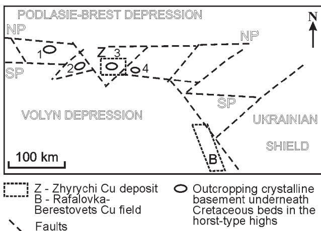
Fig. 2. Sketch of the tectonic positions of the Zhyrychi Cu deposit (Z) and Rafalovka-Berestovets Cu field (B). Fault zones: SP-SP – South-Prypyat; NP-NP – North-Prypyat. Horst-type highs of the Łuków-Ratne swell: 1 – Wishnice; 2 – Hoteshov, 3 – Ratne, 4 – Hotyslav
