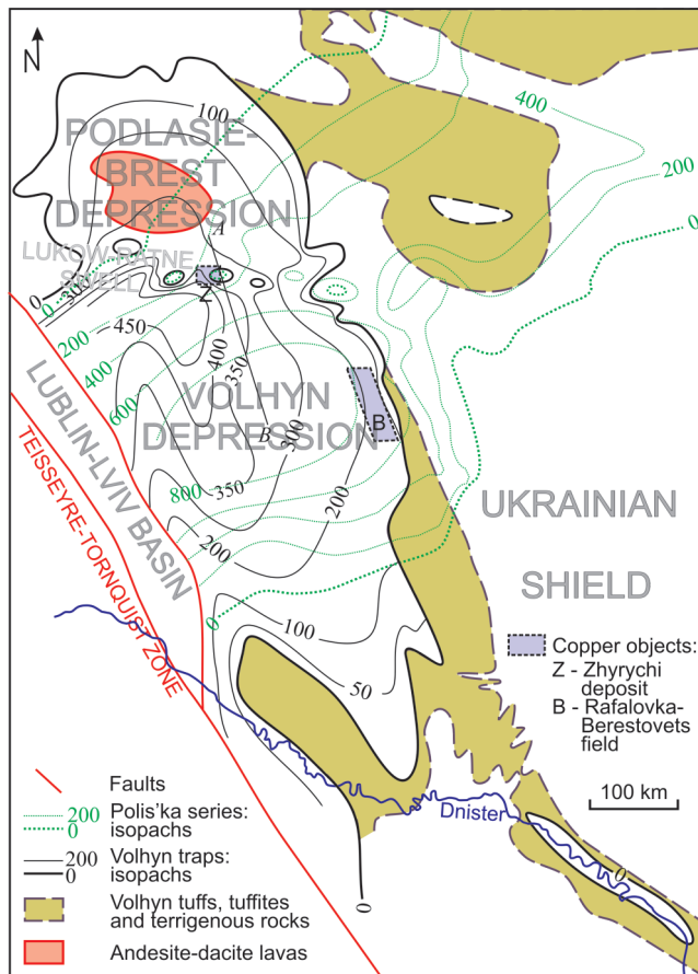
Fig. 1. Sketch map of the Western Ukraine (after Emetz et al. , 2004)
