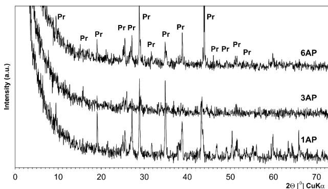
Fig. 10. X-Ray diffraction pattern of prehnite from the Zhyrychi deposit
