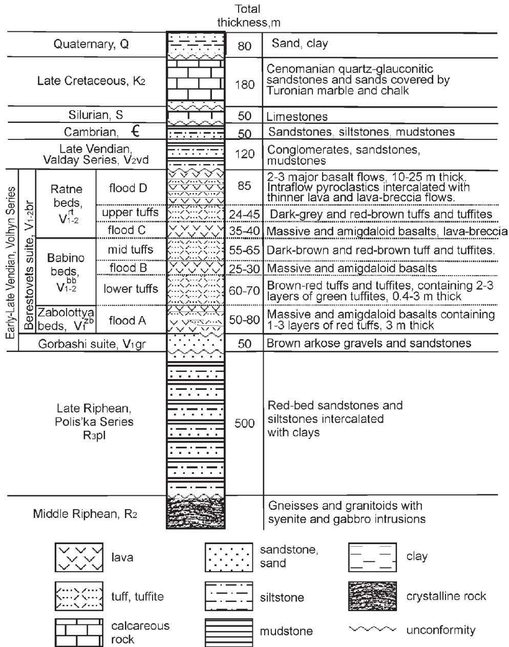
Fig. 5. Stratigraphic column of the Zhyrychi deposit
