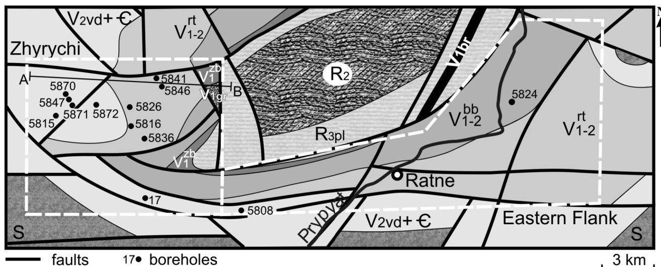
Fig. 3. Sketch geological map of the Zhyrychi deposit without Cainozoic cover (see Fig. 5 for symbol explanation)
