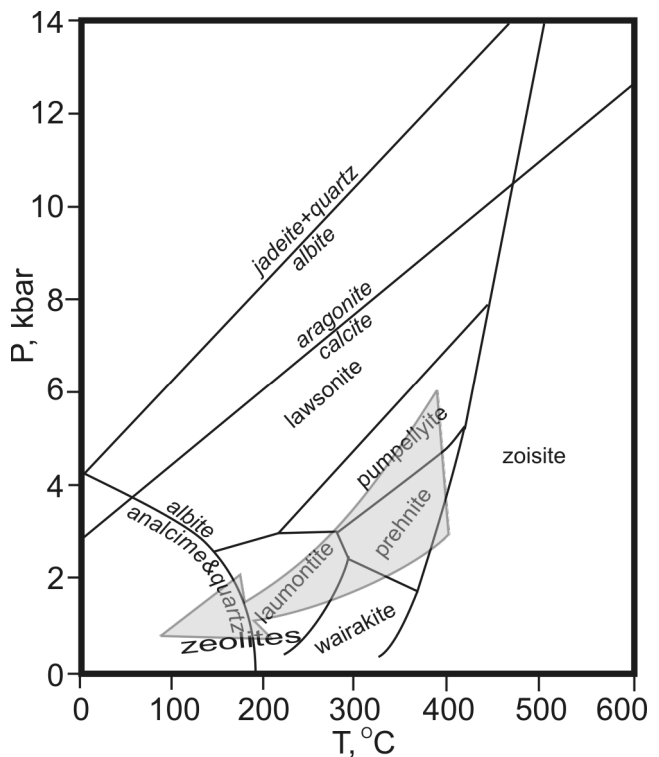
Fig. 13. P-T diagram for numerous critical reactions of the minerals of prehnite-pumpellyite and related metamorphic mineral facies (Liou, 1970, 1971; Phillipotts, 1986). The arrow shows the evolution of the mineral-forming hydrothermal system in the Zhyrychi deposit
