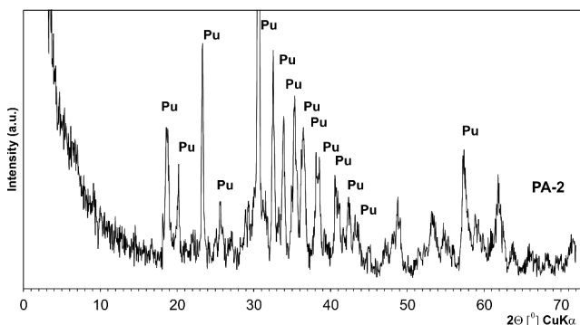
Fig. 8. X-Ray diffraction pattern of pumpellyite from the Zhyrychi deposit
