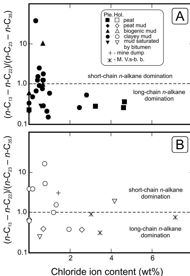
Fig. 4. Short-chain ( n\text{-}C_{13} - n\text{-}C_{22} )/long-chain ( n\text{-}C_{23} - n\text{-}C_{35} ) n -alkanes ratio in bitumen versus chloride ion content in (A) Pleistocene sediments, and (B) Holocene sediments, salt-bearing Miocene Vorotyshcha beds, and mine wastes. Ple. – Pleistocene, Hol. – Holocene, M.V.s.b.b. – Miocene Vorotyshcha salt-bearing beds
