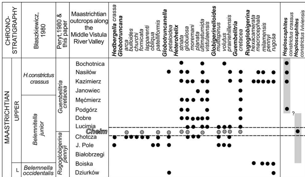
Fig. 9. The occurrence of planktonic foraminifers in the Middle Vistula River Valley section (after Peryt, 1980) and in the Chelm quarry section, plotted against the macrofaunal zonation (after Blaszkiewicz, 1980) and showing the inferred stratigraphical position of the latter section
