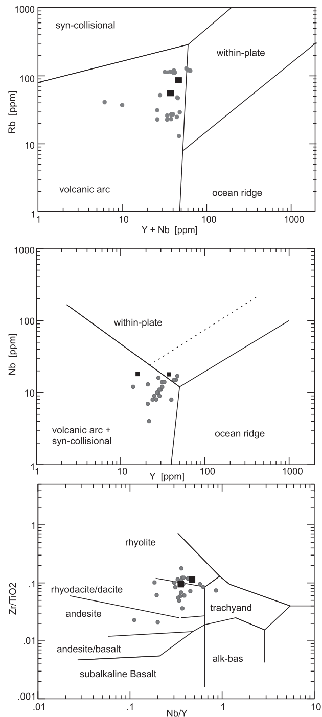
Fig. 8 Trace element discrimination diagrams for the volcanoclastic rocks clearly demonstrating that these are comparable with Early Badenian tephra known from the CF that originate from explosive eruptions of rhyolitic to rhyodacitic magmas
