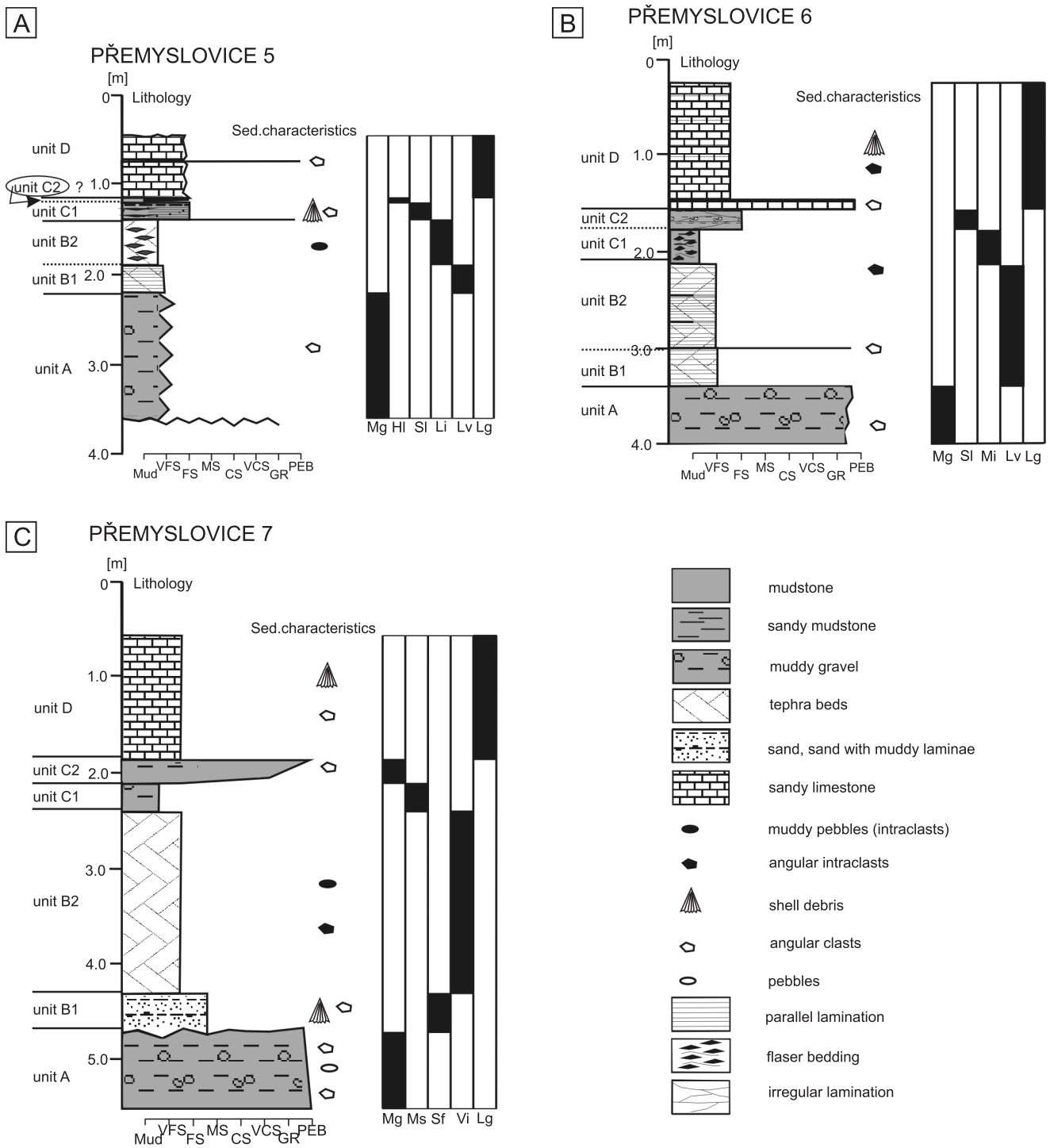
Fig. 4. Subdivision of the sedimentary and palaeontological succession in the boreholes studied in lithostratigraphic logs
