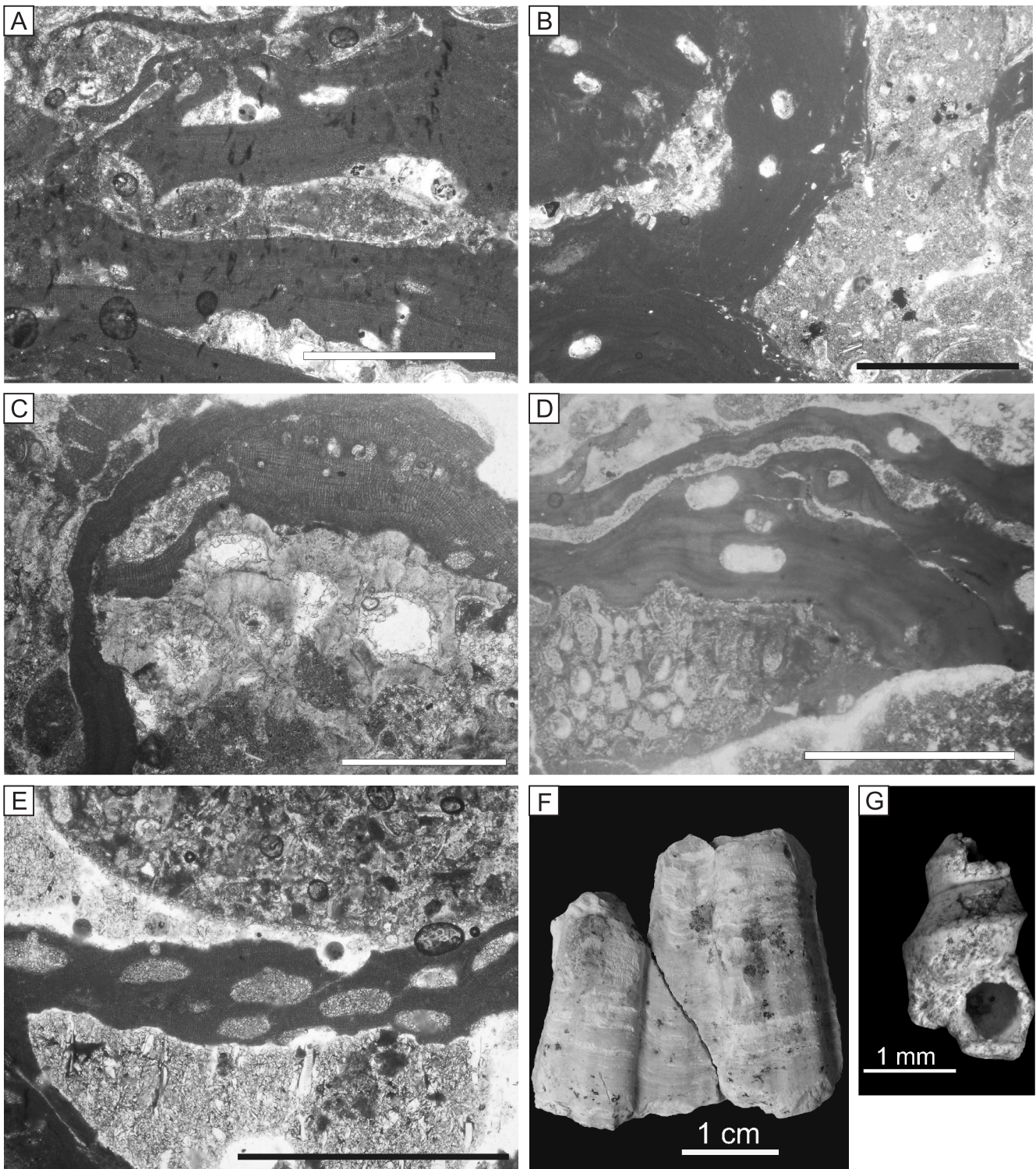
Fig. 7. Examples of algae and molluscs found in the samples studied
