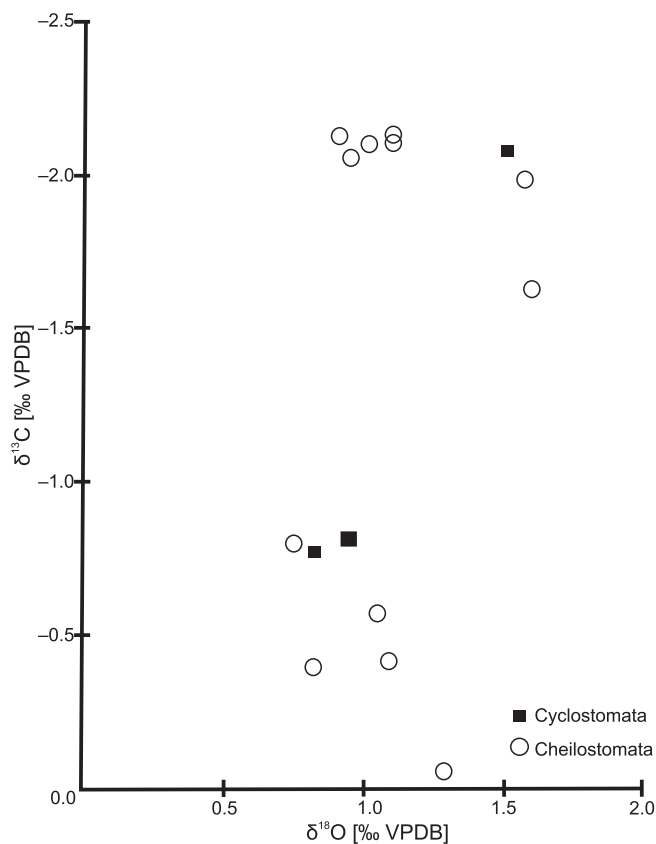
Fig. 5. Results of stable isotope analyses of bryozoan skeletons
