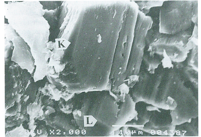
Fig. 14. Two authigenic albite crystals (K and L – points of EDS analyses) growing into pore space from altered detrital feldspar grain. SEM
