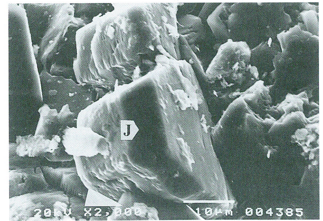
Fig. 15. Authigenic albite crystals parallelly oriented in the pore space (J – point of EDS analysis). Termination of authigenic quartz (arrow) partly engulfed in albite crystal. SEM
