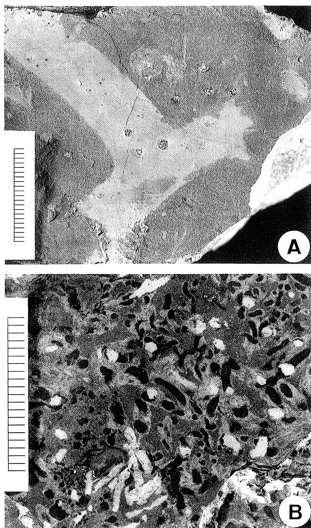
Fig. 9. Examples of ichnofabrics from the Nienadowa Marl Member in horizontal cross-sections. Millimetric scale. A. Thalassinoides suevicus crosscut by small sandy pipes, which are probably shafts of Chondrites . Lower surface of the underbed illustrated in Fig. 8D; marlstone, Zabratówka Wieś, W19. B. Phycosiphon incertum (darker spots in light mantle) crosscut by Chondrites (light spots). The upper part of the same underbed illustrated in Figs. 8D and 9A; marlstone, Zabratówka Wieś, W19
