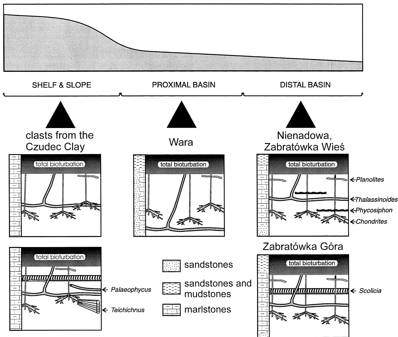
Fig. 12. Tiering patterns from different sections and their palaeoenvironmental location
