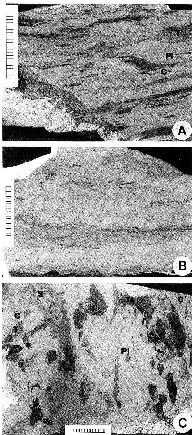
Fig. 10. Examples of ichnofabrics in marlstone clasts from the debris-flow deposits of the Czudec Clay at Wara. Millimetric scale. A. Smeared Thalassinoides (T), Planolites (PI) and Chondrites (C) in totally bioturbated background. B. Vague mottling in totally bioturbated background. C. Thalassinoides (T), Planolites (PI), Chondrites (C), Scolicia (S), Palaeophycus (Pa), ? Teichichnus (Te) and ? Taenidium (Ta) in totally bioturbated background
