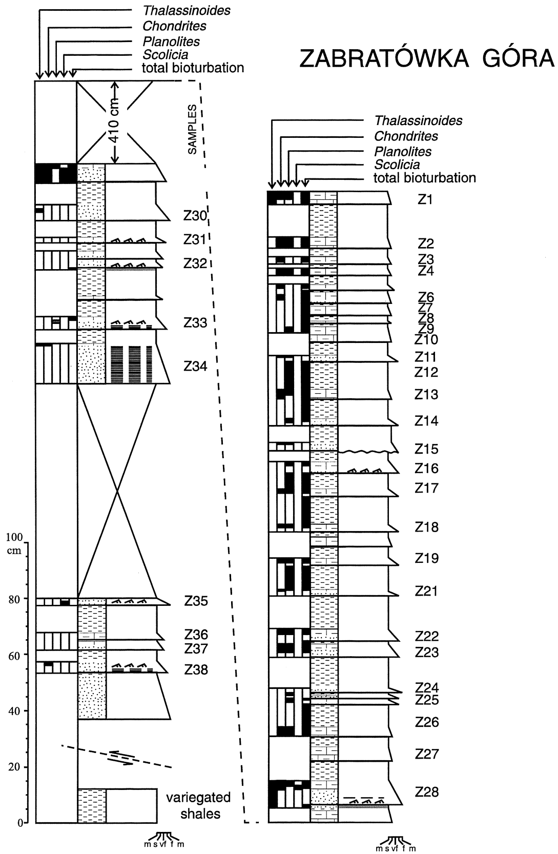
Fig. 6. Lithological column of the Nienadowa Marl Member at Zabratówka Góra with the range chart of trace fossils and bioturbation. For explanations see Fig. 3
