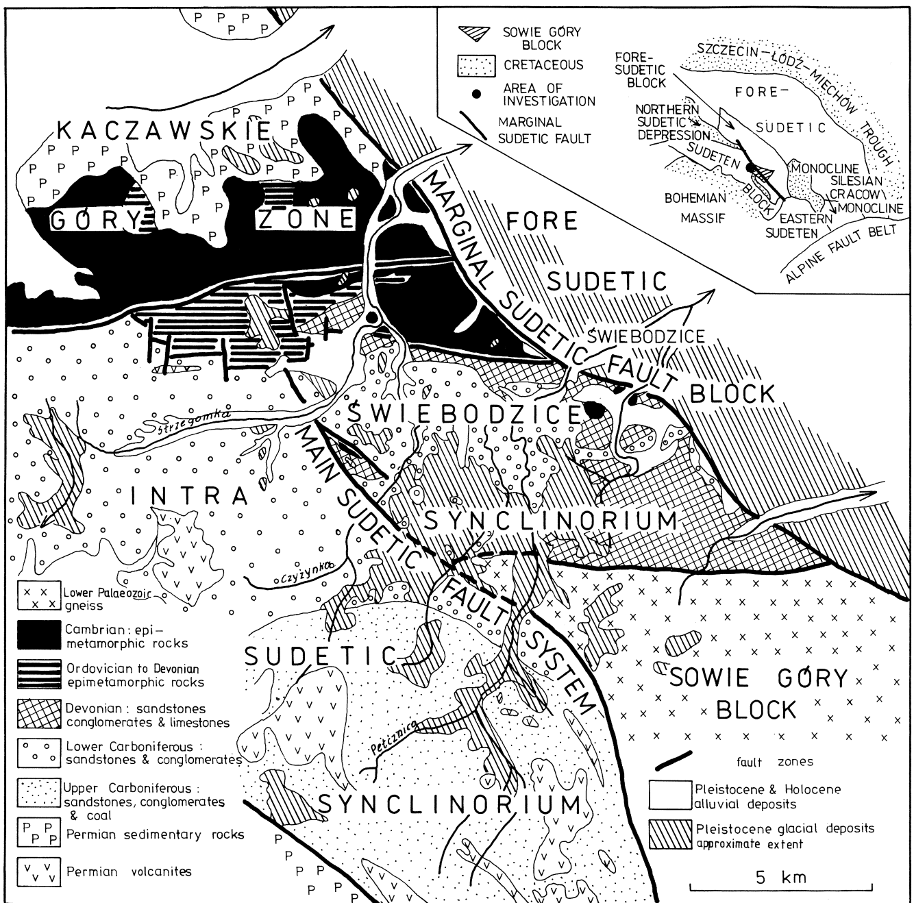
Fig. 2. Simplified geological map of the Walbrzych Upland (after Haydukiewicz et al. , 1982; Teisseyre, 1969; Teisseyre & Gawroński, 1965)
