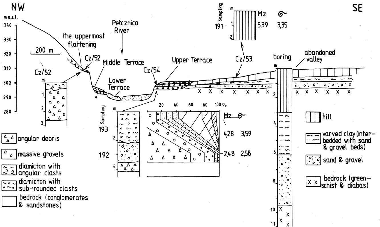
Fig. 23. Geological cross-profiles and description of trenches and borings in the Pelcznica river valley. Location of sites studied in Fig. 21. Grain size ranges are explained in Fig. 18
