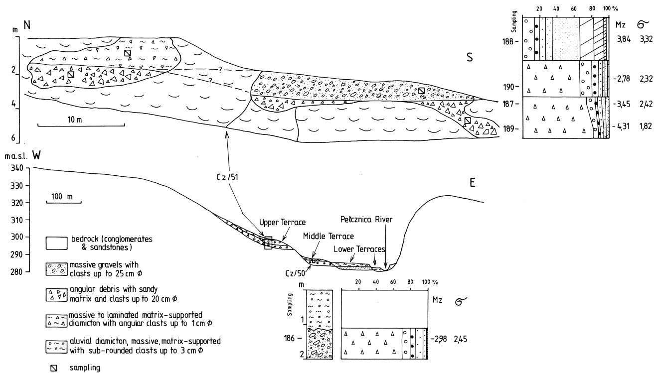
Fig. 24. Geological cross-profiles and description of outcrops and trenches in the Pelcznica river valley. Location of sites studied in Fig. 21. Grain size ranges are explained in Fig. 18
