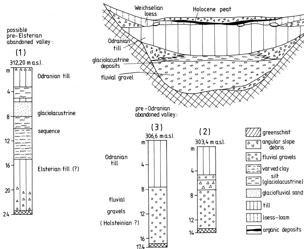
Fig. 16. Geological profiles (boring-logs) of the abandoned valleys near Dobromierz. The section in upper right is based on the data from the outcrop described by A. Jahn ( vide Stachura, 1993a) (location of borings and the outcrop is in Fig. 13)
