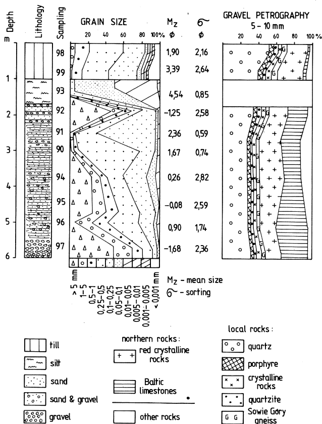
Fig. 32. Sediment stratigraphy and lithological and petrographical properties of deposits at site Czyżynka 70
