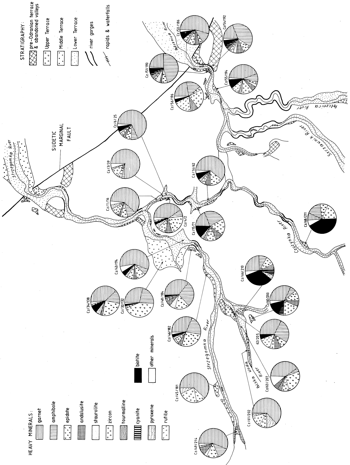
Fig. 29. Heavy mineral content of alluvial deposits of the Waibrzych Upland and its distribution along the river valleys
