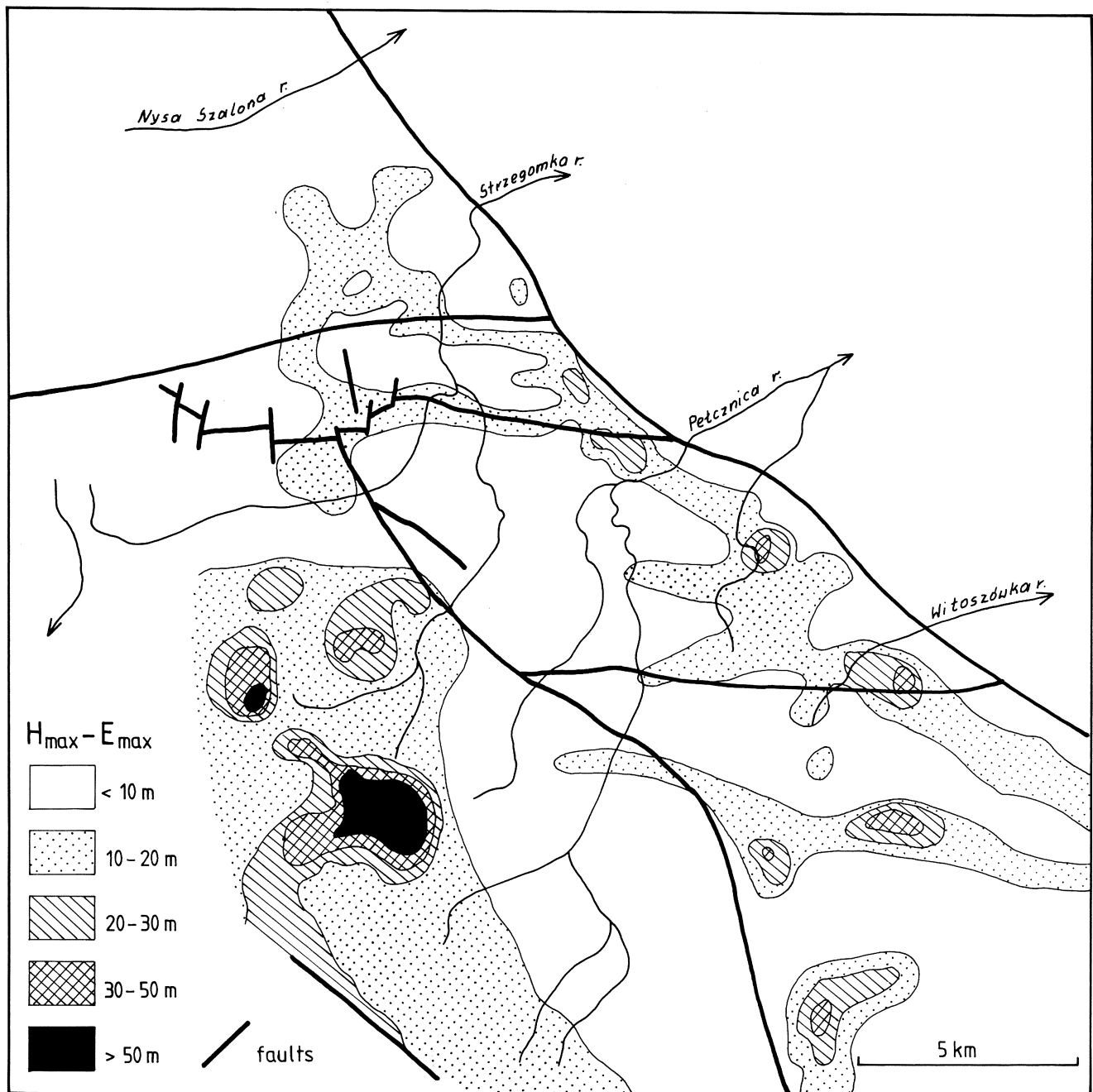
Fig. 6. Map of the relief belt above headstream erosion ( H_{max} - E_{max} – highest elevation in m a.s.l., E_{max} – highest position of erosion). The map has been interpolated on the basis of a topographic map (1:25 000) with a net of squares (area 1 \text{ km}^2 , distance between centres 0.5 km)
