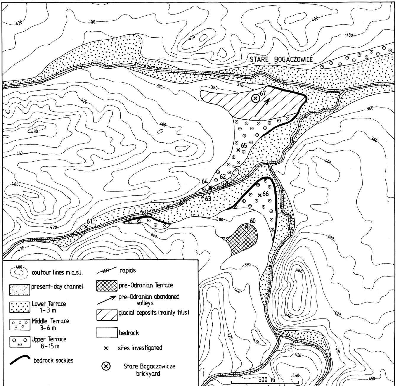
Fig. 19. Quaternary geology and position of alluvial terraces in the Stare Bogaczowice Depression (Strzegomka, Polska Woda and Chwaliszówka river valleys). Location map in Fig. 1
