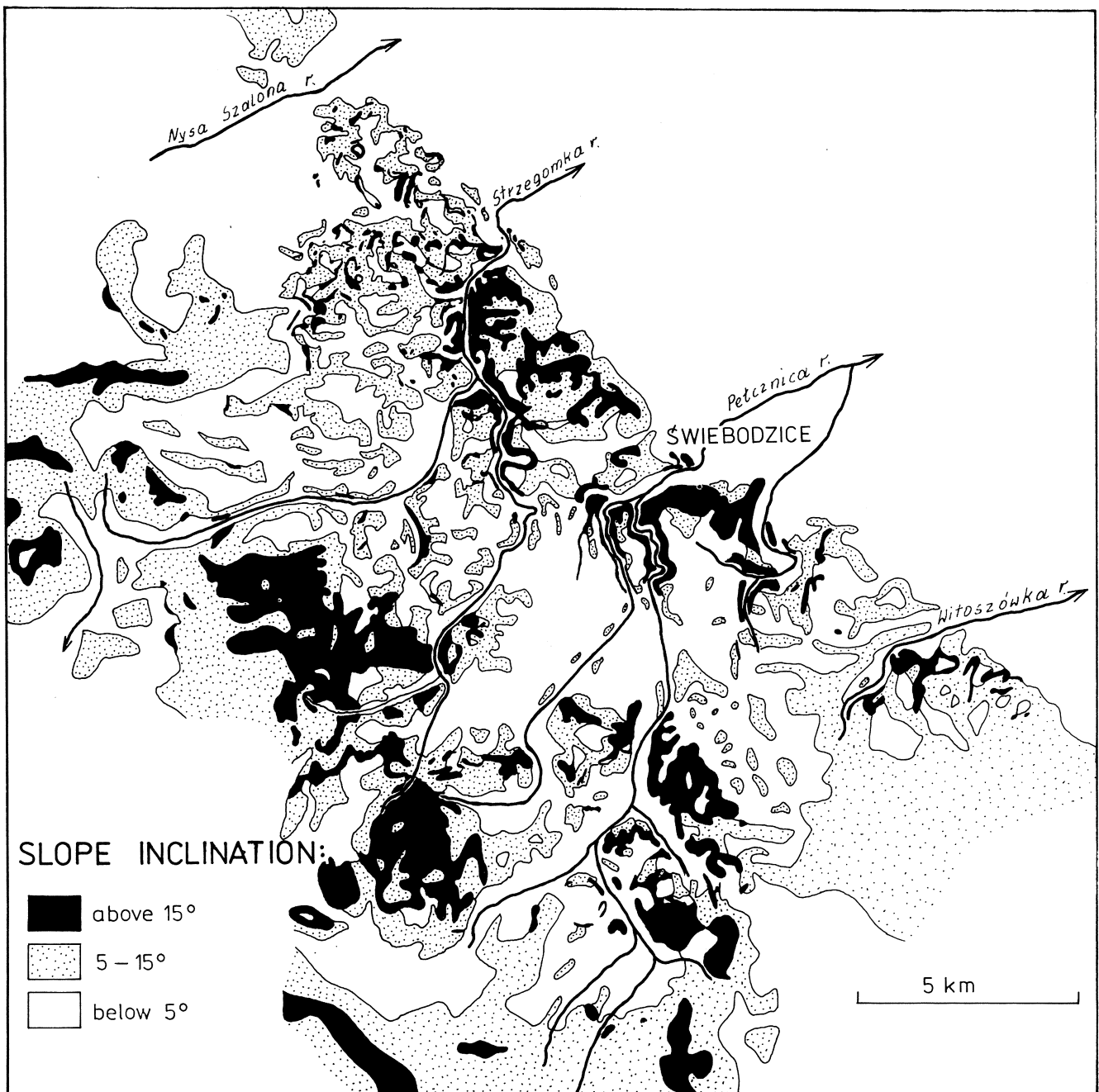
Fig. 4. Map of slope inclination. The map has been compiled on the basis of a topographic map (1:25 000) using the equation \text{tg}\alpha = \text{hd}^{-1} , where \alpha – slope inclination, h – height between contour lines, d – distance between contour lines
