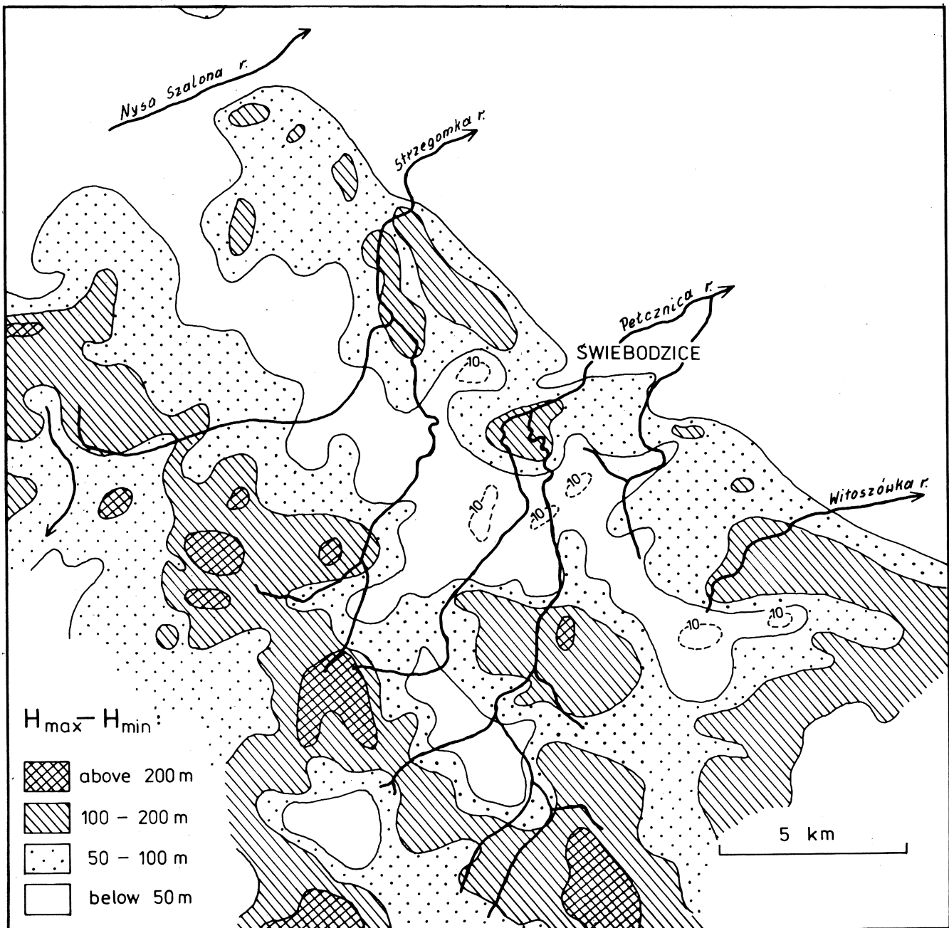
Fig. 5. Map of relief energy ( H_{max} – highest elevation in m a.s.l., H_{min} – lowest elevation in m a.s.l.). The map has been interpolated on the basis of a topographic map (1:25 000) with a net of squares (area 1 \text{ km}^2 , distance between centres 0.5 km)
