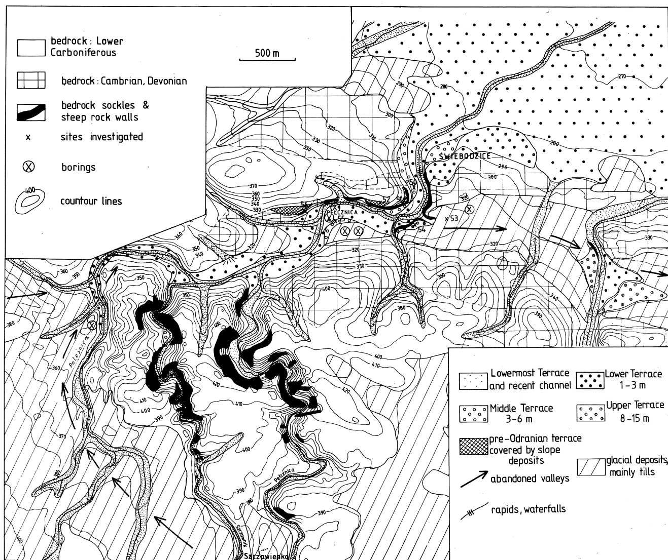
Fig. 21. Quaternary geology and position of alluvial terraces and abandoned valleys in the lower Pelcznica river valley near Świebodzice. Location map in Fig. 1
