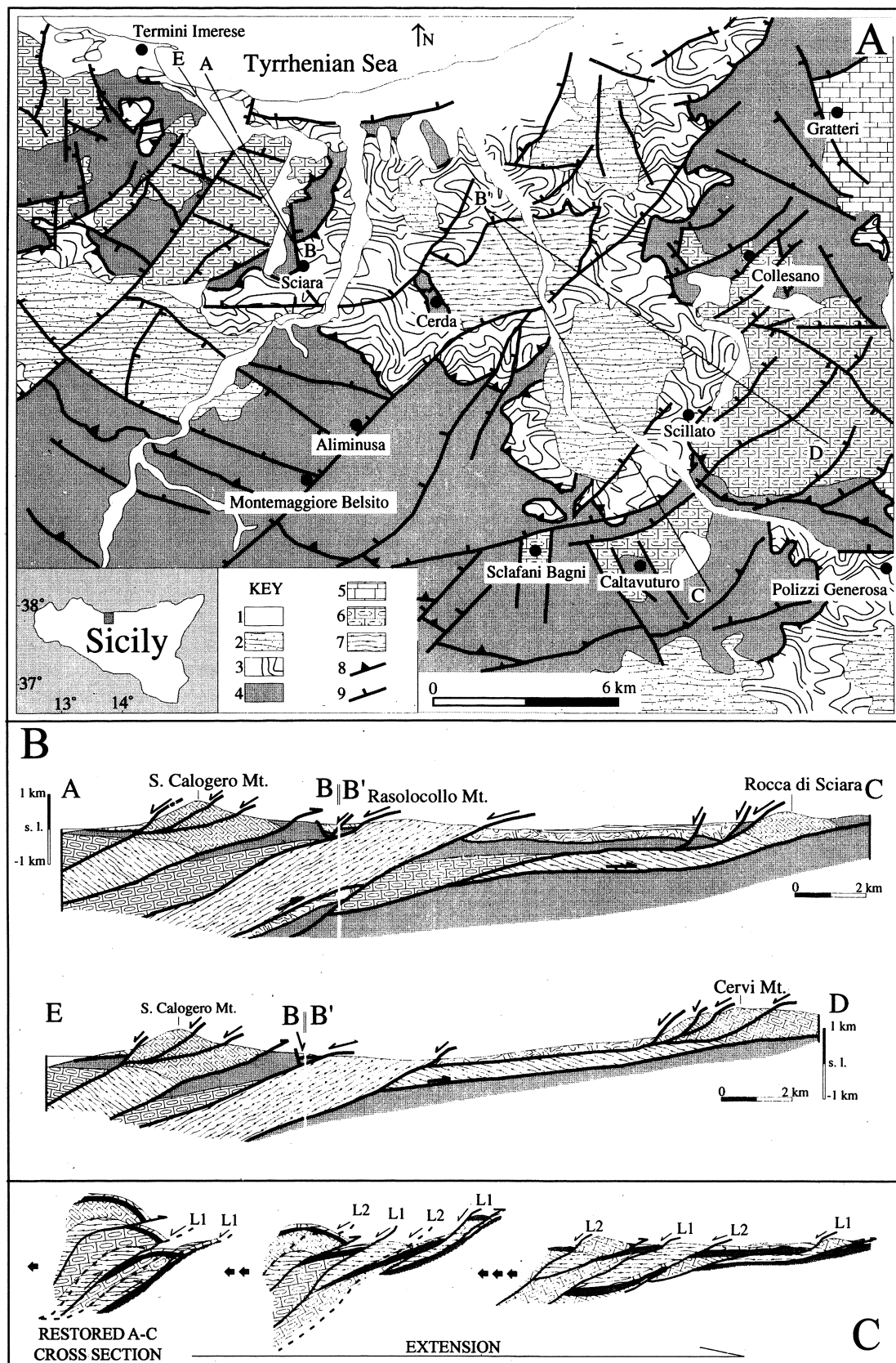
Fig. 11. A. Geological map and sections across the Madonie Mts. tectonic edifice, affected by neotectonic LNF systems. 1 – Pleistocene deposits; 2 – Tortonian–Pliocene sequences; 3 – Cretaceous–Paleogene Sicilidi terranes; 4 – Oligocene–Miocene Numidian Flysch; 5 – Mesozoic carbonates of Panormide Unit; 6 – Mesozoic carbonates of Imerese Unit; 7 – Triassic turbiditic sequences (Lercara Fm.); 8 – main thrusts; 9 – main extensional faults. B. Cross sections. C. Restored A–C cross section in which two main extensional events (L1 and L2) occurred during the Plio-Pleistocene. The key is the same for cross-sections
