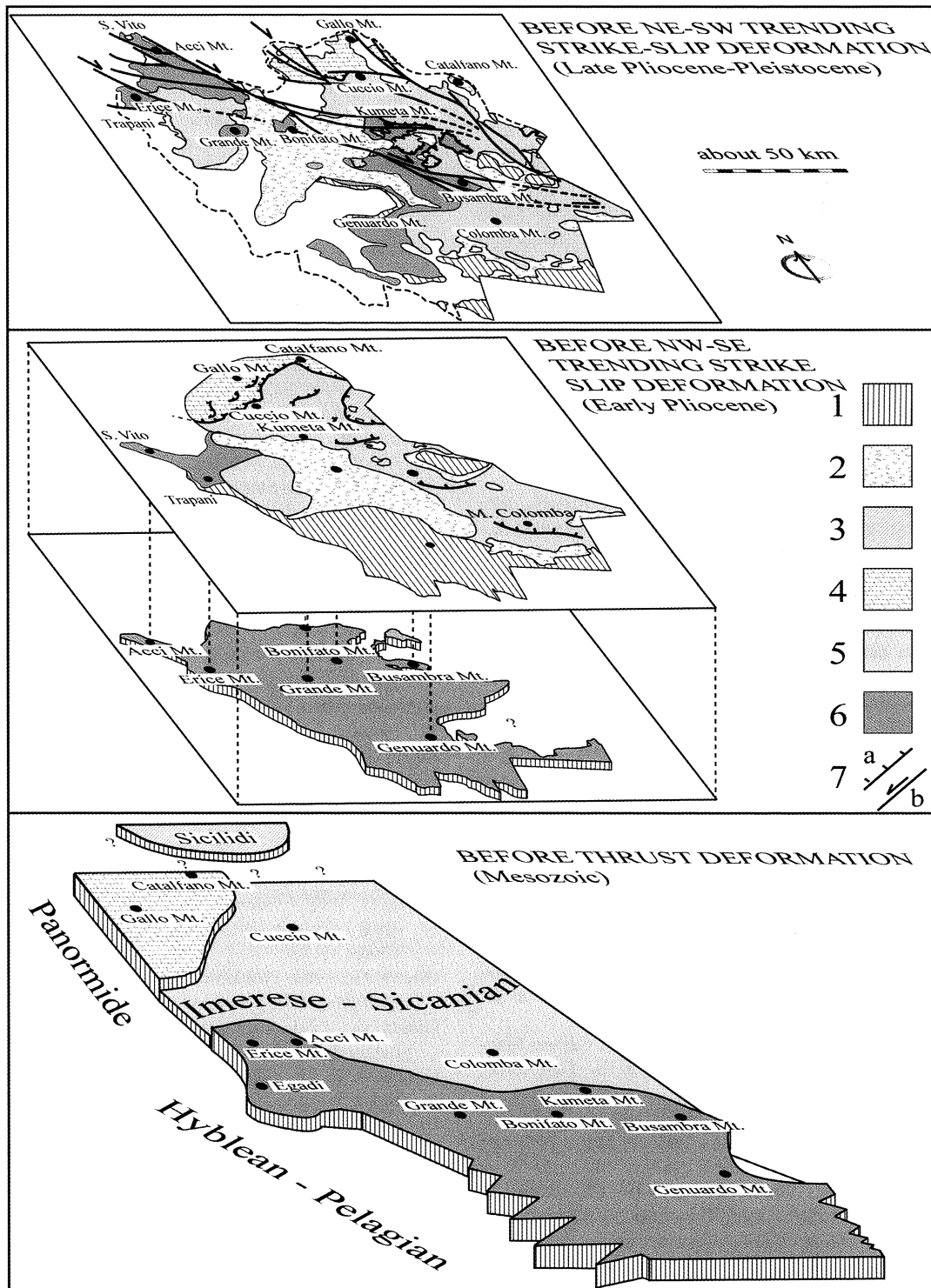
Fig. 8. Semiquantitative restoration of Western Sicily Chain. 1 – Messinian–Pleistocene successions; 2 – Tortonian successions; 3 – Sicilide units; 4 – Panormide units; 5 – Imerese–Sicanian units; 6 – Hyblean–Pelagian successions; 7a – main thrust; 7b – main strike-slip faults
