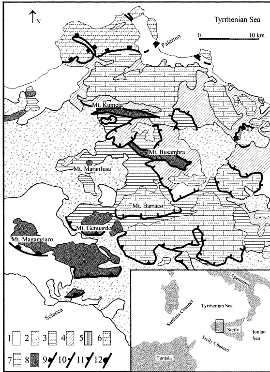
Fig. 2. Schematic structural map of North-Central Sicily. Fore-deep and coeval intramountain basin deposits: 1 – Middle Pliocene–Pleistocene; 2 – Late Tortonian–Early Pliocene; 3 – Serravallian–Middle Tortonian; 4 – Late Oligocene–Langhian. 5 – Sicilide Units (Cretaceous–Oligocene); 6 – Panormide Units (Late Triassic–Oligocene); 7 – Imerese–Sicanian Units (Early Liassic–Oligocene); 8 – Hyblean–Pelagian Units (Late Triassic–Late Miocene). Main thrust fronts: 9 – Early–Middle Miocene; 10 – Late Miocene; 11 – Pliocene; 12 – Pleistocene
