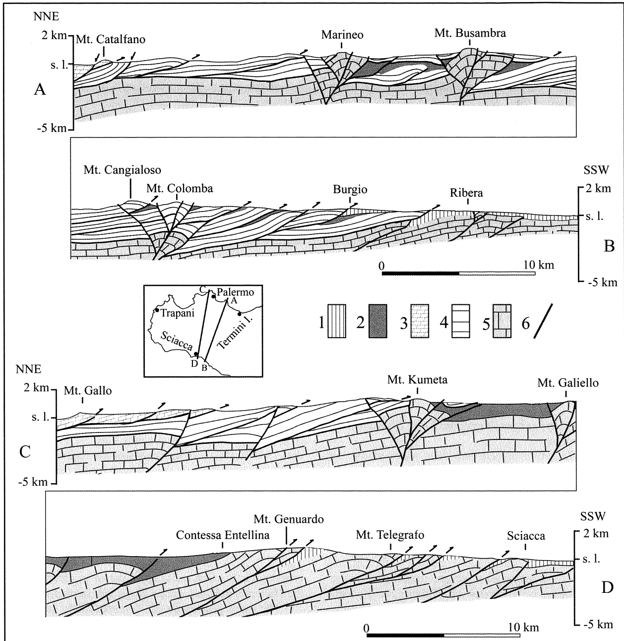
Fig. 6. Schematic structural sections across North-Central Sicily. 1 – Plio-Pleistocene deposits involved in the deformation; 2 – Late Miocene–Early Pliocene deposits involved in the deformation; 3 – Panormide units and their Numidian covers (Late Triassic–Late Langhian); 4 – Imerese–Sicanian units and their Numidian covers (Early Triassic–Middle Tortonian); 5 – Hyblean–Pelagian units (Late Triassic–Late Miocene); 6 – thrust and high-angle reverse faults
