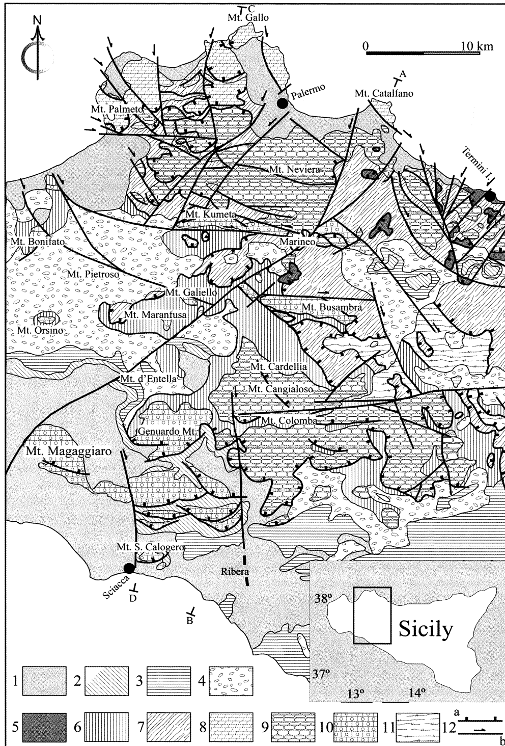
Fig. 5. Schematic geological map of the North-Central Sicily. 1 – marls, sands and arenites (Middle Pliocene–Pleistocene); 2 – Trubi Fm. (Early Pliocene); 3 – diatomitic deposits, evaporitic limestones, gypsum and clays (Messinian); 4 – conglomerates, sands, clays and reef limestones (Late Tortonian–Early Messinian); 5 – Sicilide sequences: varicoloured clays and micritic limestones with planktonic foraminifers (“argille scagliose” and Polizzi Fm., Late Cretaceous–Oligocene). Numidian sequences: 6 – clays, marls, quartz-arenites, carbonatic and/or glauconitic arenites and rudites, clays and marls with planktonic foraminifers (external Numidian sequences, Late Oligocene–Tortonian); 7 – clays, sandy clays and quartz-arenites (Numidian Flysch s. s. , Late Oligocene–Late Langhian); 8 – Panormide Domain-derived sequences: carbonate platform sequences, dolomites, marls and marly limestones (Late Triassic–Oligocene); 9 – Imerese–Sicanian Domain-derived sequences: clays, cherty limestones, dolomites, radiolarites, micritic limestones, marls and carbonatic breccias (Late Triassic–Oligocene); 10 – Hyblean–Pelagian Domain-derived sequences: carbonate platform sequences, marly limestones, marls and micritic limestones, boundstones and carbonatic arenites and rudites with benthonic foraminifers (Late Triassic–Miocene); 11 – “Lercara Basin” sequences: clays, marls and quartz-arenites with inserted carbonatic breccias made of Palaeozoic carbonate platform clasts (Early–Middle Triassic); 12 – main thrust front (a) and high-angle faults (b). Arrows indicate strike-slip movements. A-B and C-D indicate the geological cross sections of Fig. 6
