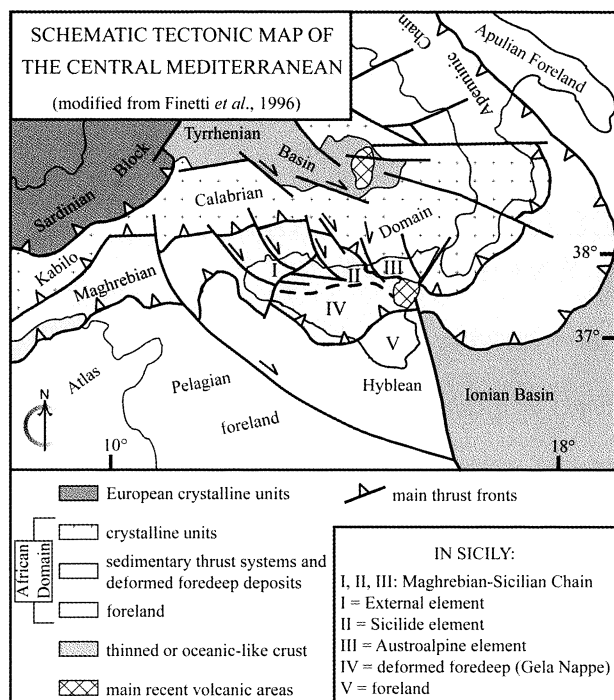
Fig. 1. Studied area in the frame of the Central Mediterranean geodynamic context
