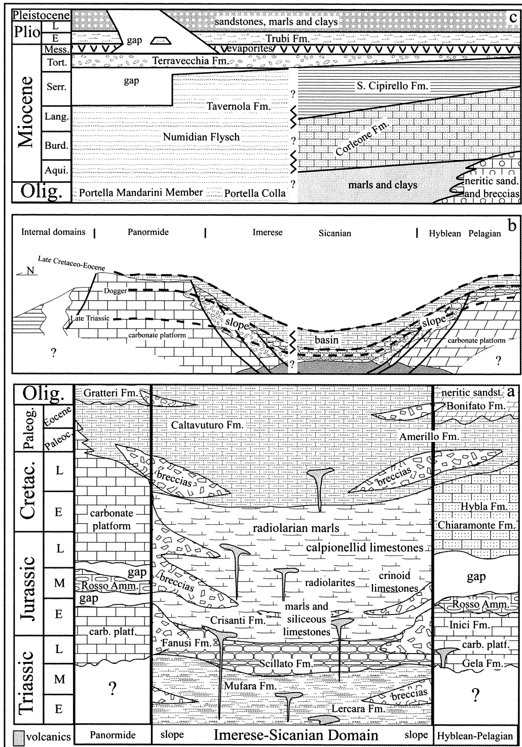
Fig. 4. Stratigraphic scheme and palaeogeographic domains of Western Sicily. a) Stratigraphy and facies distribution during the Triassic–Oligocene time. b) Palaeogeographic scheme during the Mesozoic–Tertiary. c) Stratigraphy and foredeep sequences distribution during the Late Oligocene–Pleistocene
