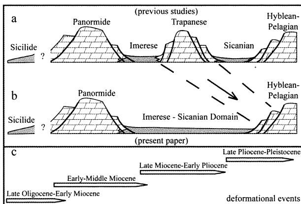
Fig. 3. a–b) Comparison between the palaeogeographic model of the Authors during the Mesozoic and the model proposed in the present paper; c) chronology of deformational events
