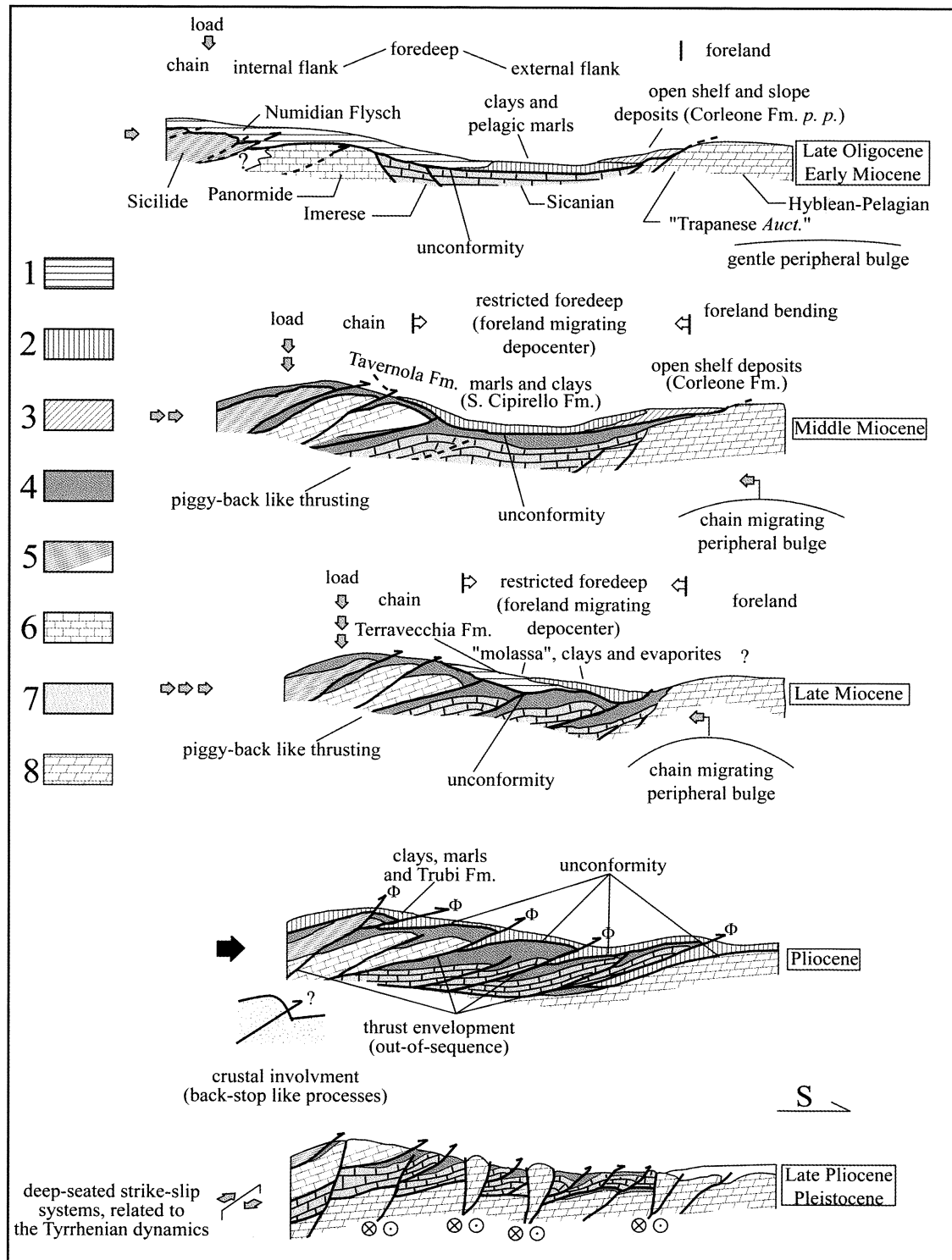
Fig. 7. Kinematic model of the tectono-sedimentary evolution of North-Central Sicily during the Miocene-Pliocene. 1 – internal flank foredeep deposits; 2 – depocentral foredeep deposits; 3 – external flank foredeep and/or foreland deposits; 4 – foredeep deposits progressively incorporated in the chain construction; 5 – internal Sicilide tectonic units; 6 – Panormide tectonic units; 7 – Imerese-Sicilian tectonic units; 8 – Hyblean-Pelagian tectonic units
