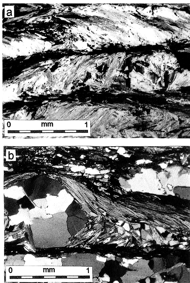
Fig. 12. Foliation S_1 preserved in microlithons between younger foliation planes S_2 : a – foliation S_2 (horizontal on the photo) developed parallel to axial planes of crenulations of foliation S_1 in coarse-grained schist, b – foliation S_1 in fine-grained schist preserved in the hinge of a crenulation micro-fold in foliation S_2 (horizontal on the photo)
