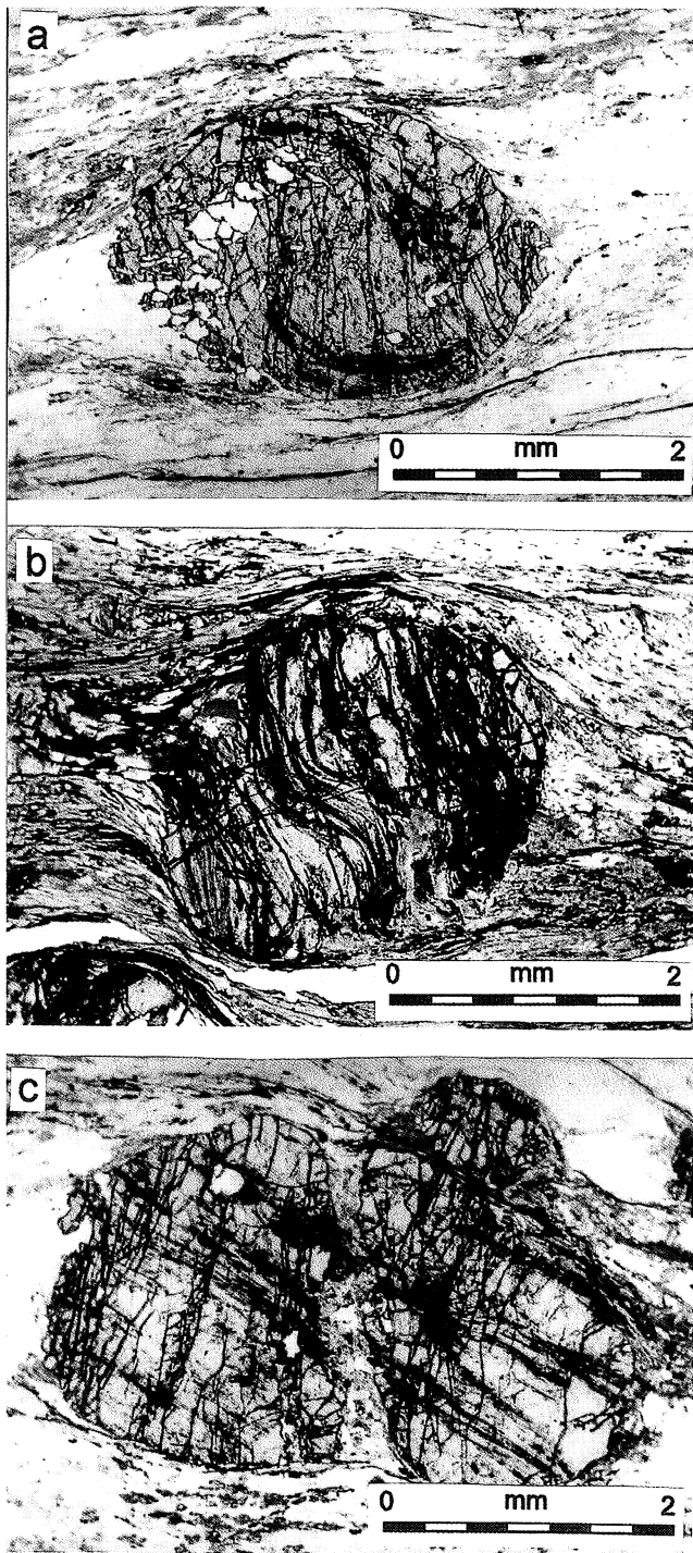
Fig. 9. Shape varieties of inclusion trails in garnet porphyroblasts: a – spiral inclusion trails, b – sigmoidal inclusion trails, c – straight-line inclusion trails
