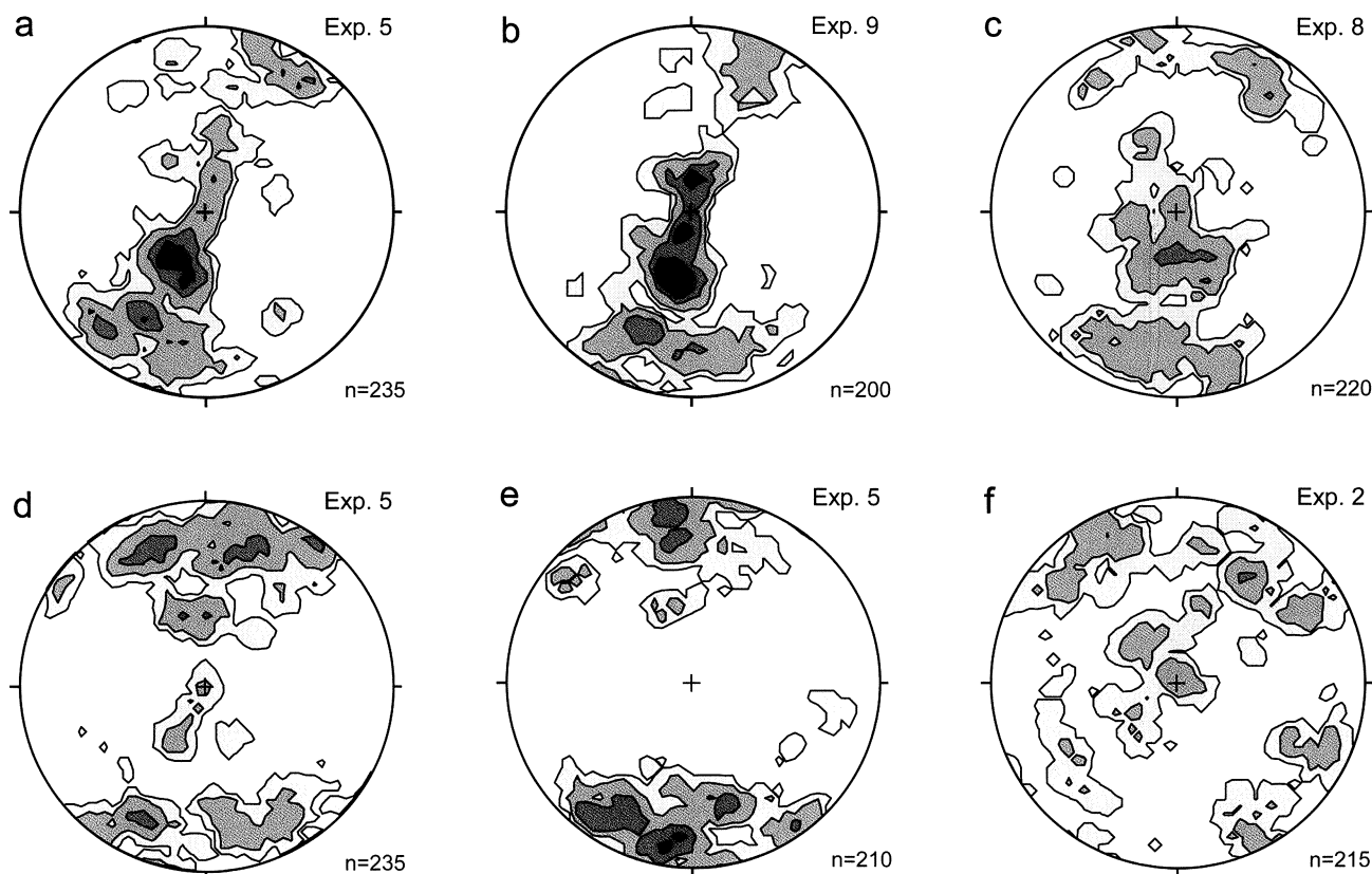
Fig. 18. Representative examples of quartz c-axis patterns in coarse-grained mica schists from vicinities of Kamieniec Ząbkowicki. Equal-area net, lower hemisphere. Density contours at 2% intervals. Projection plane is XZ plane of strain ellipsoid. Attitude of foliation corresponds to a plane perpendicular to the figure. Lineation (parallel to X axis of strain ellipsoid) trends parallel to the figure. a, d, e – exposure 5; b – exposure 9; c – exposure 8; f – exposure 2
