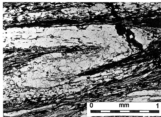
Fig. 13. Intrafolial fold in fine-grained schist. Folded foliation S_1 is preserved between planes of penetrative foliation S_2
