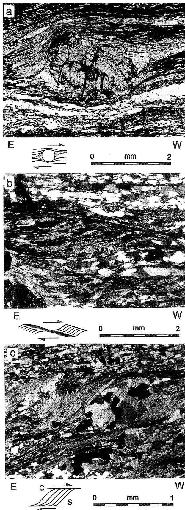
Fig. 16. Examples of kinematic indicators related to the D 3 deformation in the mica schists from the vicinity of Kamieniec Ząbkowicki. In all three cases sense of shear is top-to-SW along the S 2+3 foliation: a – asymmetric pressure shadows around garnet porphyroblast in fine-grained mica schist (Kamieniec unit), b – extensional crenulation cleavage in fine-grained mica schist (Kamieniec unit), c – S-C structure in albite-bearing mica schist (Byczeń unit)
