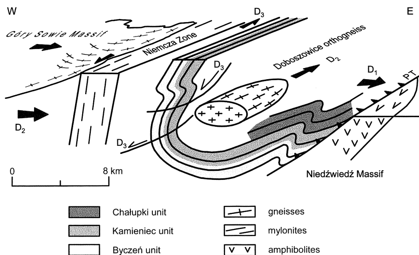
Fig. 23. Schematic block diagram showing the structural geometry of metamorphic complexes between the Góry Sowie Massif and the Niedźwiedź Massif. Chałupki, Kamieniec and Byczeń units are separated by overthrusts (here omitted for sake of simplicity). PT – Paczków overthrust
