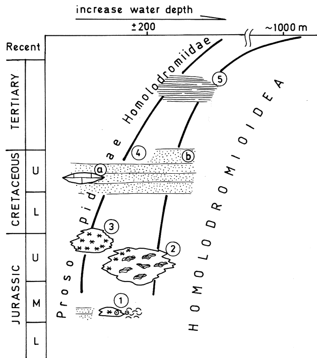
Fig. 33. Trend of environmental displacement of Homolodromioidea crabs from Jurassic to Recent based on palaeo- and ecological preferences of fossil and extant taxa. 1 – Middle Jurassic environments: shallow-water siliciclastic and carbonate (coral reefs, crinoid limestones, brachiopod shell beds) deposits; 2 – Oxfordian cyanobacteria-sponge and sponge-coral buildups; 3 – Tithonian Štramberk coral reefs; 4 – Upper Cretaceous shallow water siliciclastic (a – with limestone lenses) and outer shelf (b) environments; 5 – Tertiary outer shelf deposits
