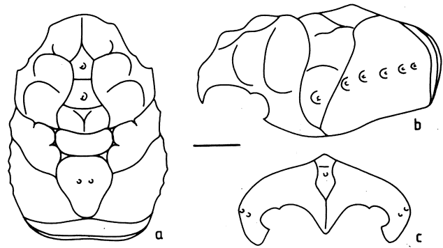
Fig. 8. Vectis wrighti Withers. Lower Aptian, Isle of Wight, England (after Glaessner, 1969); a – dorsal view; b – lateral view; c – frontal view. Length of scale bar – 1 mm
