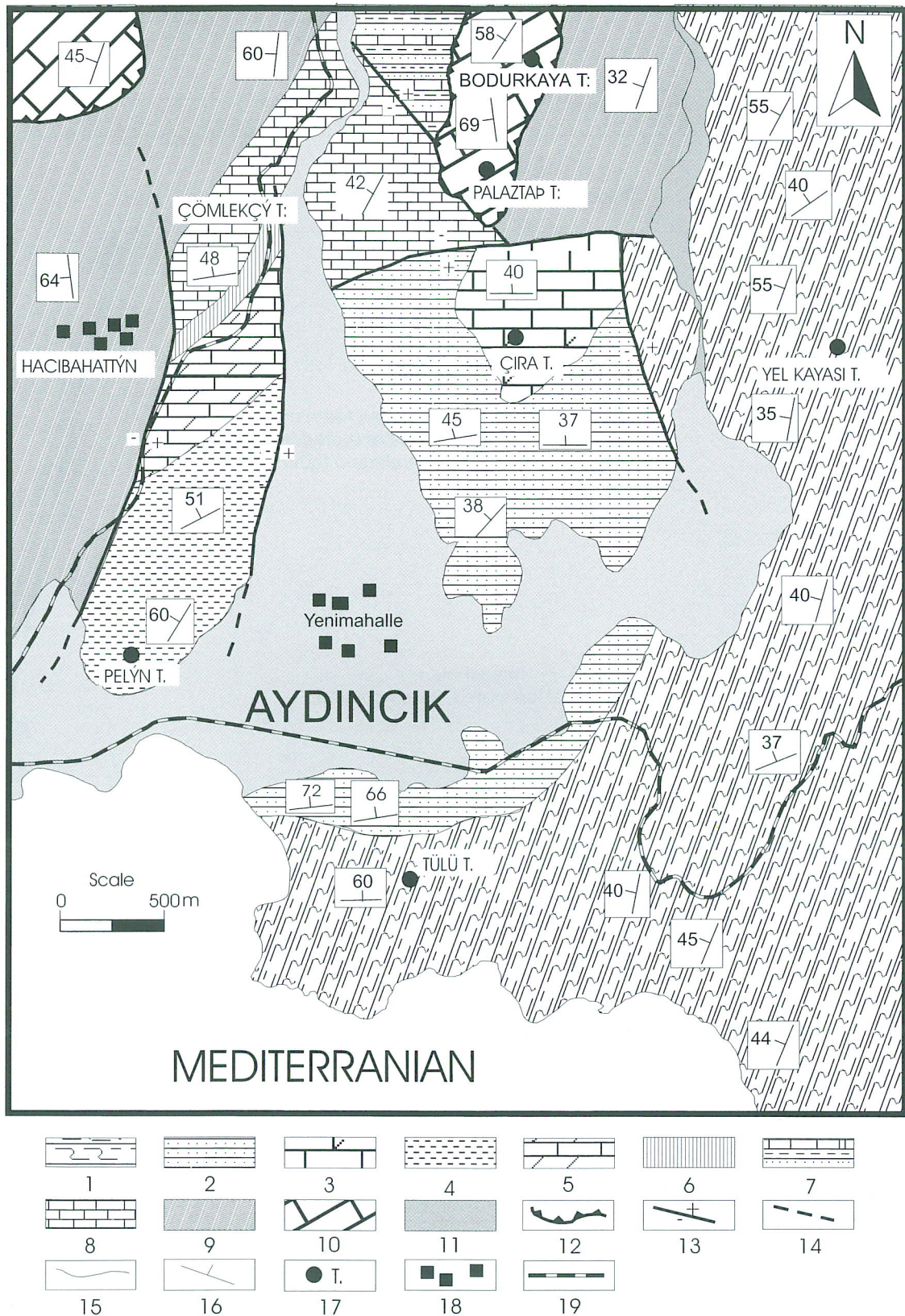
Fig. 3. Geological map of the study area (Modified from Koç, 1996). 1 – Sipahili Formation (Infra-Cambrian); 2 – Hüdai Formation (Early Cambrian); 3 – Çaltepe Formation (Early to Middle Cambrian); 4 – Seyditehir Formation (Late Cambrian to Ordovician); 5 – Büyükeceli Formation (Middle Ordovician); 6 – Akdere Formation (Late Devonian); 7 – Korucuk Formation (Early Carboniferous); 8 – Kirtıldağı Formation (Late Permian); 9 – Murtçukuru Formation (Late Triassic); 10 – Cehennemdere Formation (Jurassic to Early Cretaceous); 11 – alluvium; 12 – thrust fault; 13 – fault; 14 – probable fault; 15 – formation boundary; 16 – strike and dip of bedding; 17 – hill; 18 – district; 19 – main road
