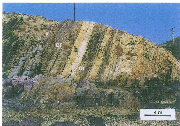
Fig. 2. An excellent exposure of the Hüdai Formation at the coastal area showing a rhythmic bedding. The beds are facing to the north. The sequence comprises cream colored, horizontal laminated sandstone (h), ripple cross-laminated sandstone (cr) predominantly red in color, and green colored mixed sandstone-shale (m) and rarely shale
