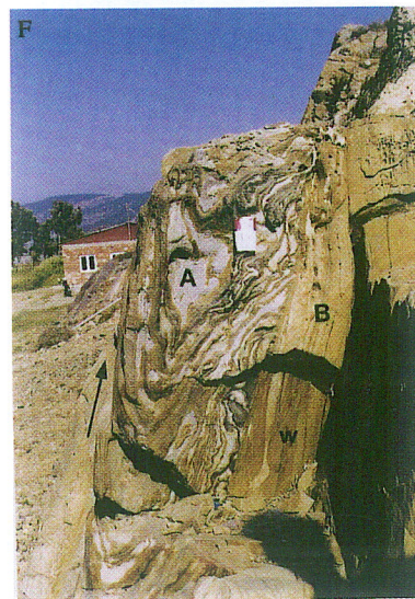
Fig. 5. Sedimentary structures in the Hüdai Formation. A. Horizontal laminated sandstone. Dark laminae indicate clay rich intervals. B. Typical ripple cross-laminated sandstone (R). Arrow indicates reactivation surface. M – Alternating laminae of sandstone shale in the mixed sandstone-shale. C. General view of ripple-marks on the bedding surface in the cross-laminated sandstone facies. The pitch of ripple-crest is measured as 40^\circ . D. Symmetrical, flat-topped ripples in the cross-laminated sandstone facies. E. Interference ripples in the cross-laminated sandstone facies. F. Large scaled overturned lamination (A) in the cross-laminated sandstone facies. Arrow indicates current flow direction. The right-hand part of the photograph (B) show wavy and lenticular bedding (w) in the mixed sandstone-shale facies. Dark areas indicate clay-rich intervals (w). G. Convolute lamination in the cross-laminated sandstone facies showing syn-depositional deformation
