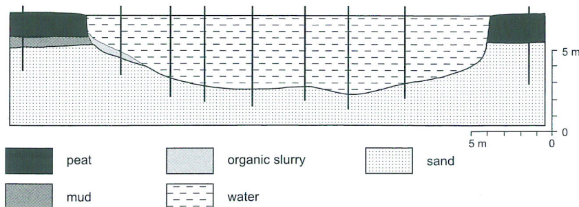
Fig. 8. Cross-section through a canal-like channel, boreholes marked with vertical lines
