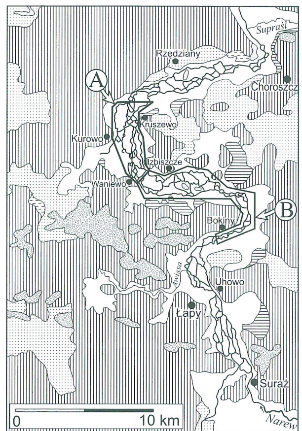
Fig. 1. The upper Narew river between Suraz and Tykocin. The channel network in the section downstream from Rzędziany is shown as before drainage works
