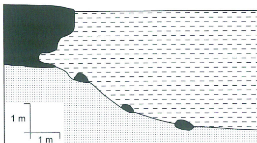
Fig. 14. An example of eroded peat bank
