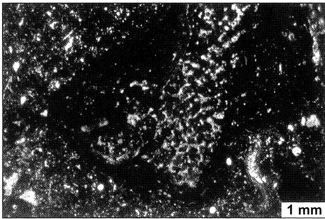
Fig. 7. Boundstone. Siliceous sponge overgrown with microbolites; chalky limestones, Jasna Cave
