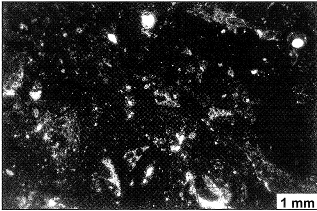
Fig. 6. Thrombolitic boundstone; chalky limestones, Jasna Cave
