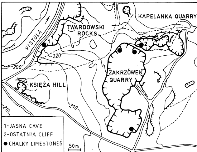
Fig. 2. Location sketch of the study area (names of exposures after Szelerewicz & Górny, 1986 and Król & Barabasz, 1997)
