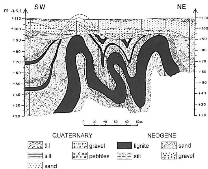
Fig. 7. Geological cross-section of the Sieniawa deposit (after Ciuk, 1968) — an example of glacioteclonic deposits
