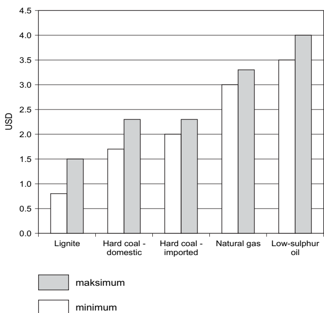
Fig. 10. Cost of 1 GJ of energy; comparison of the different energy sources (after Bielikowski et al. , 1999)
