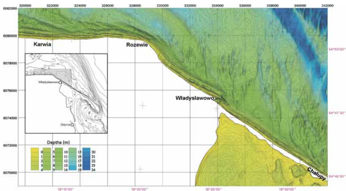
Fig. 1. Bathymetric digital map of the sea bottom at the Władysławowo region (scale 1:25,000) with isobaths every 0.25 m. Location of the study area is presented on the inset bathymetric map “Sea Bottom Relief”, Plate I (Mojski, 1995)
