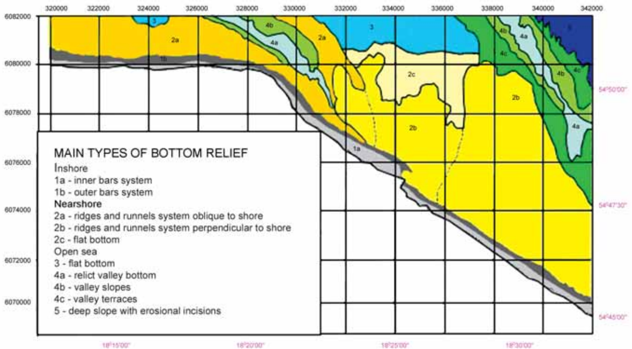
Fig. 2. Main types of sea bottom relief
