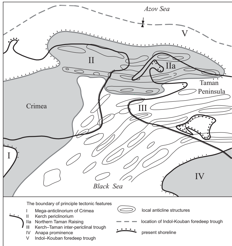
Fig. 4. General features of geological structure of Kerch–Taman region
