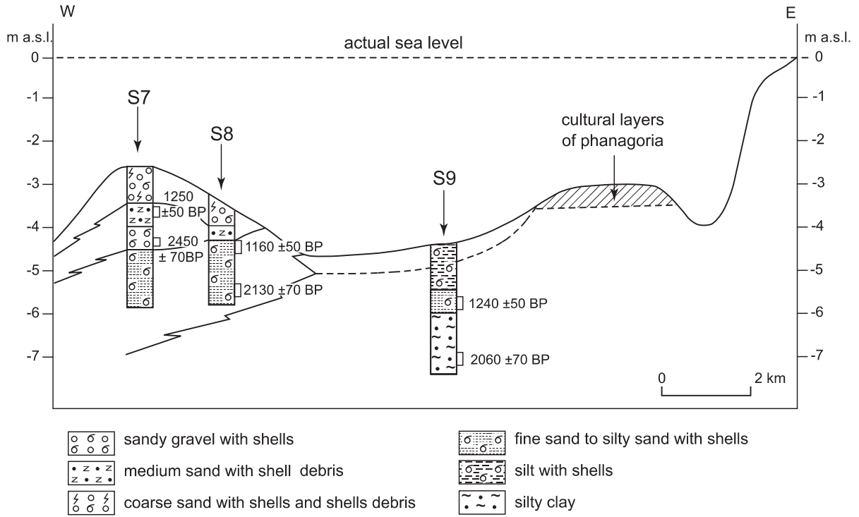
Fig. 9. Gulf of Taman
