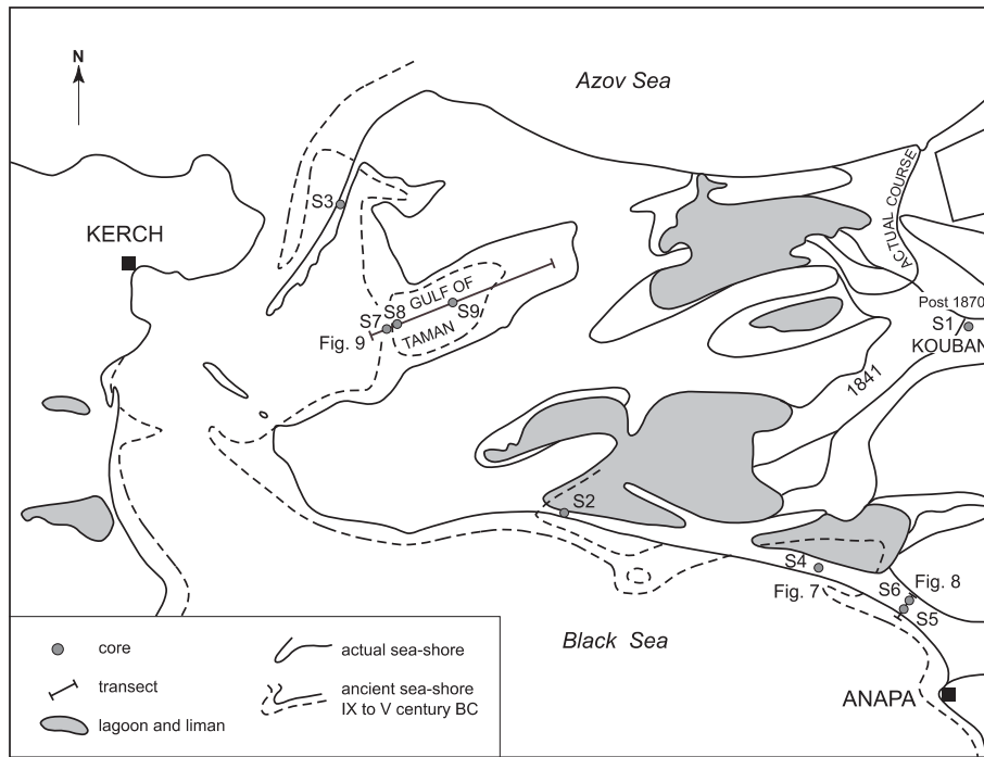
Fig. 3. Possible reconstruction of sea-shore IX to V century BC (adapted from Nevesky, 1958)
