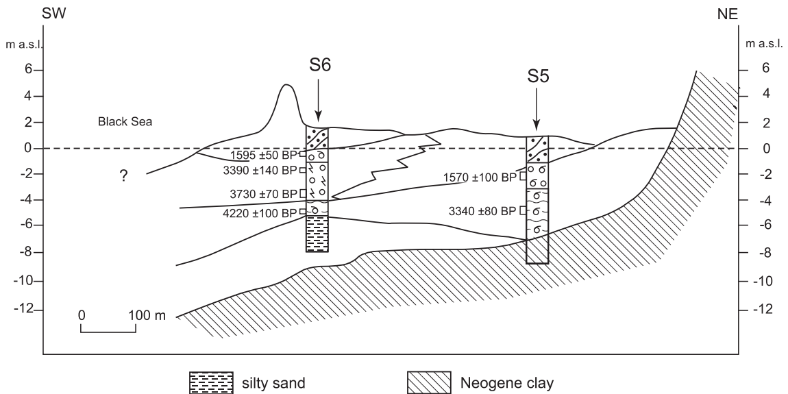
Fig. 8. Eastern part of Anapa Spit
