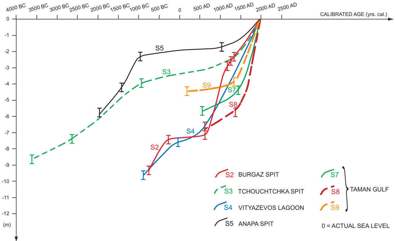
Fig. 10. Relative regional sea level fluctuations in Taman Peninsula
