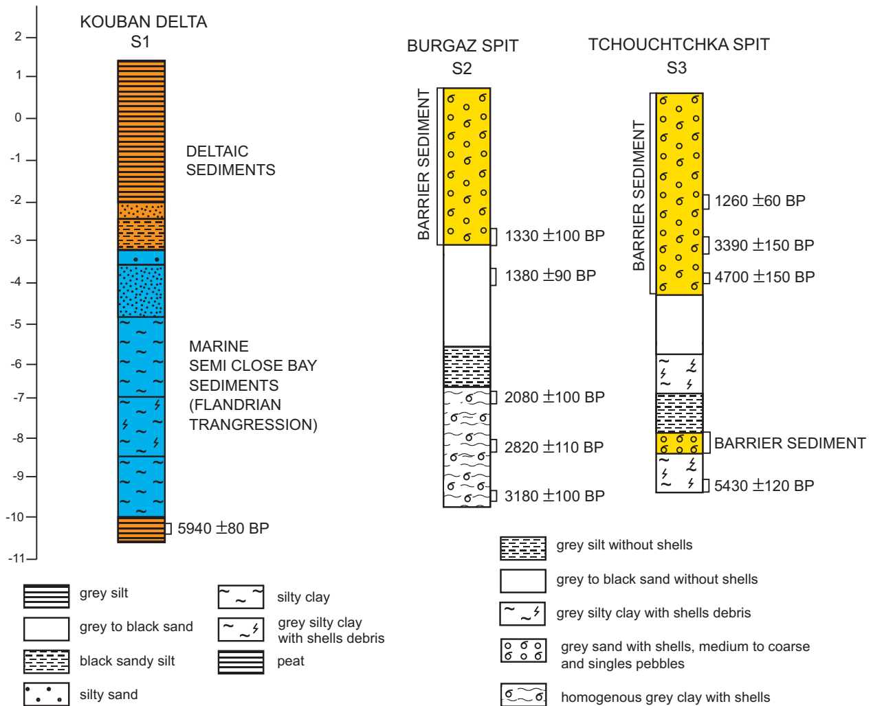
Fig. 6. Cores S1, S2, S3
