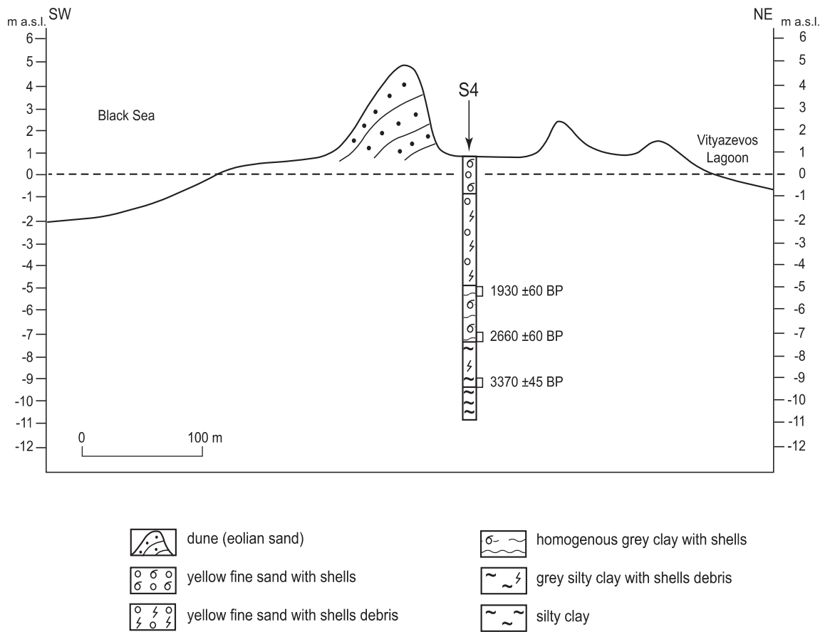
Fig. 7. Anapa Spit
