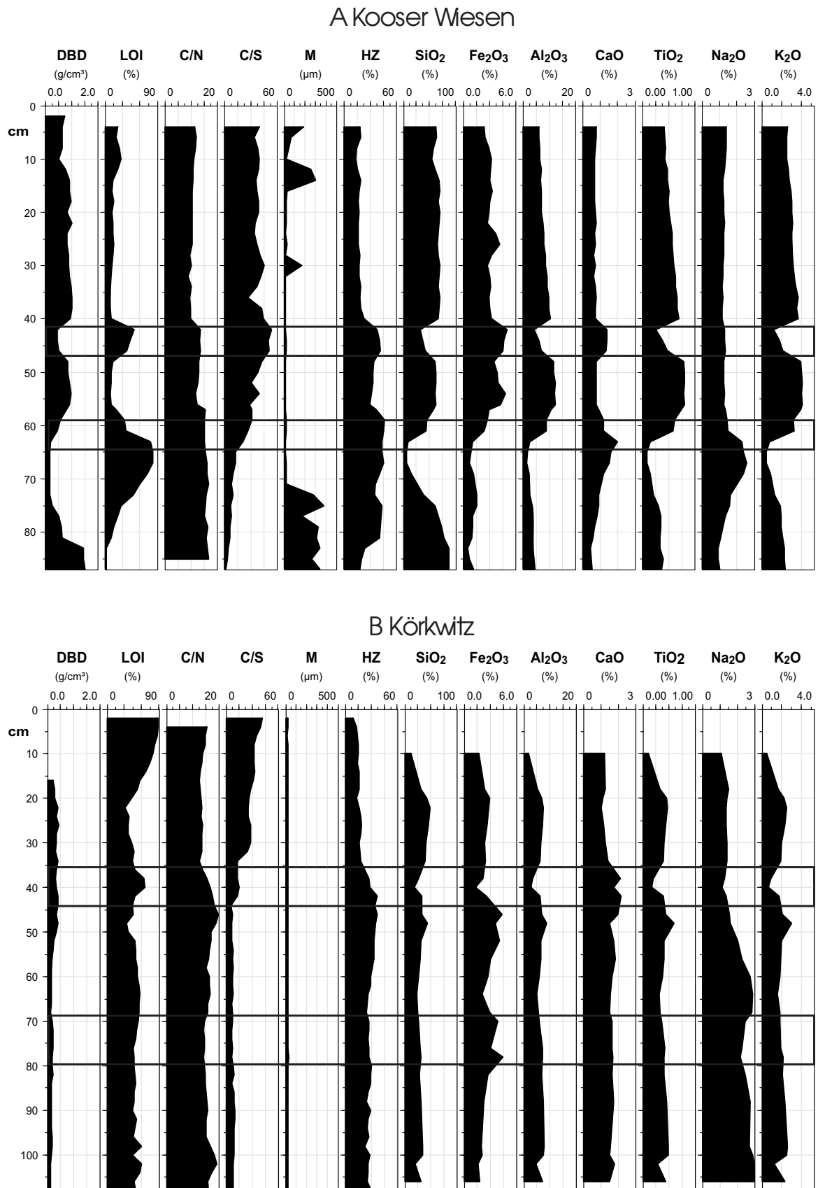
Fig. 3. Distribution of geochemical parameters: Kooser Wiesen site (A) and Körkwitz site (B)
