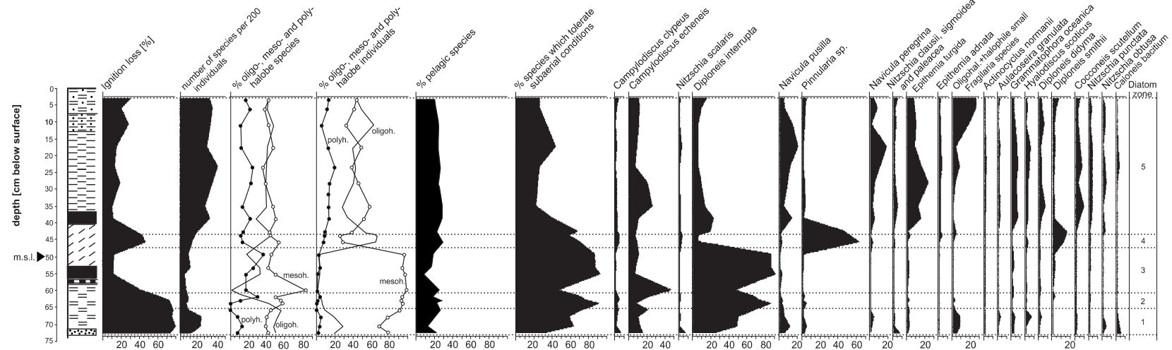
Fig. 2. Pollen and diatom diagram, Kooser Wiesen site, near Greifswald
