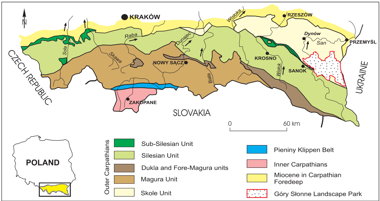
Fig. 1. Localisation of the Góry Słonne Landscape Park against the background of the geological structure of the Carpathians
