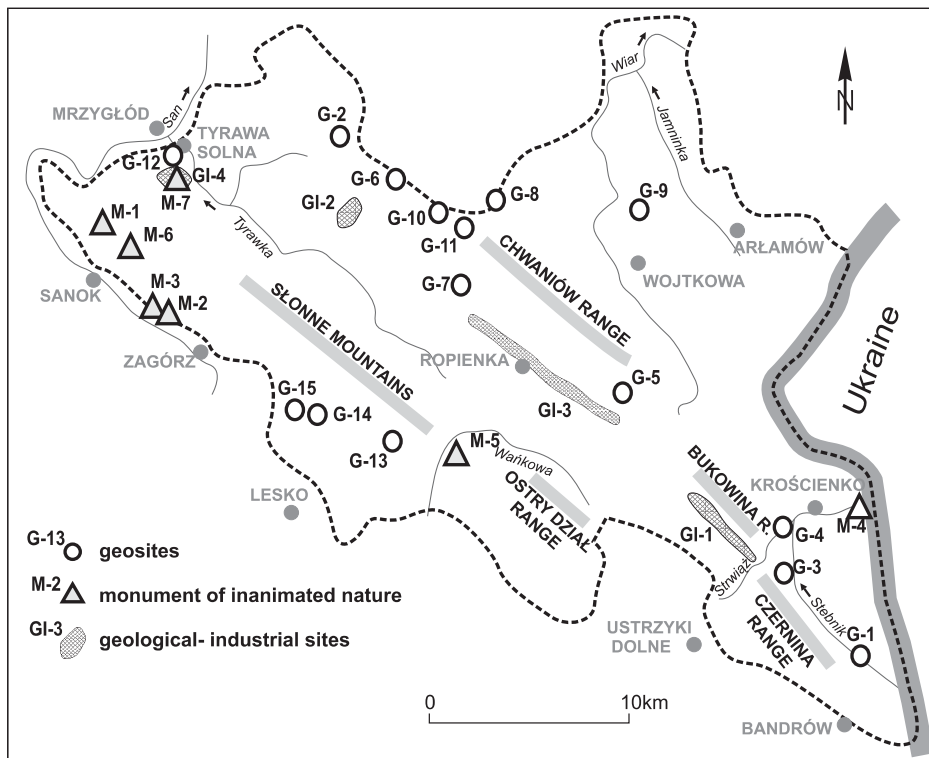
Fig. 2. The Góry Słonne Landscape Park with the localisation of the proposed for protection documentary sites, monuments of the inanimate nature and geological-industrial sites against the background of morphological structures and drainage pattern
