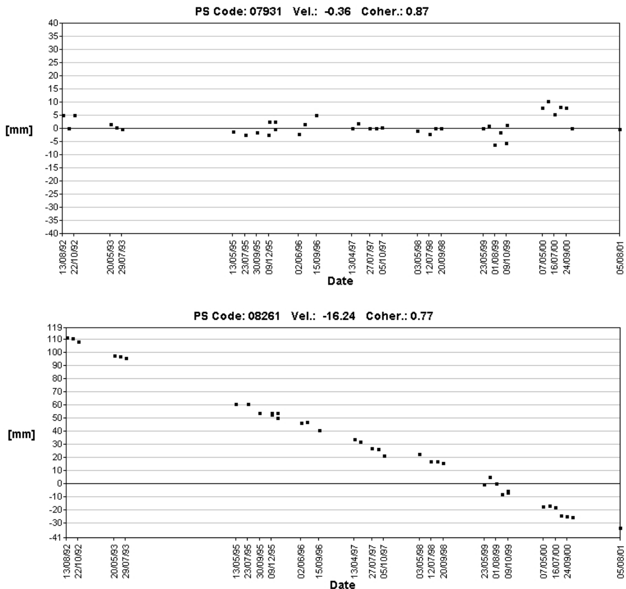
Fig. 4. LOS displacement time series of PS 1 (upper graph) and PS 2 (lower graph) situated, respectively, outside and within the Triesenberg–Triesen landslide (see Figure 3 for location)
