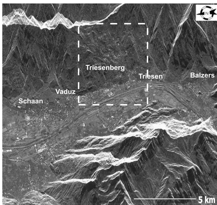
Fig. 2. Multi-image SAR reflectivity map of the Triesenberg–Triesen landslide area located in Rhine river valley Liechtenstein (after Colesanti, Wasowski, 2004, modified)
