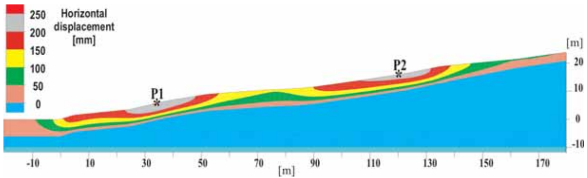
Fig. 12. Predicted five-years horizontal displacement of the slope
