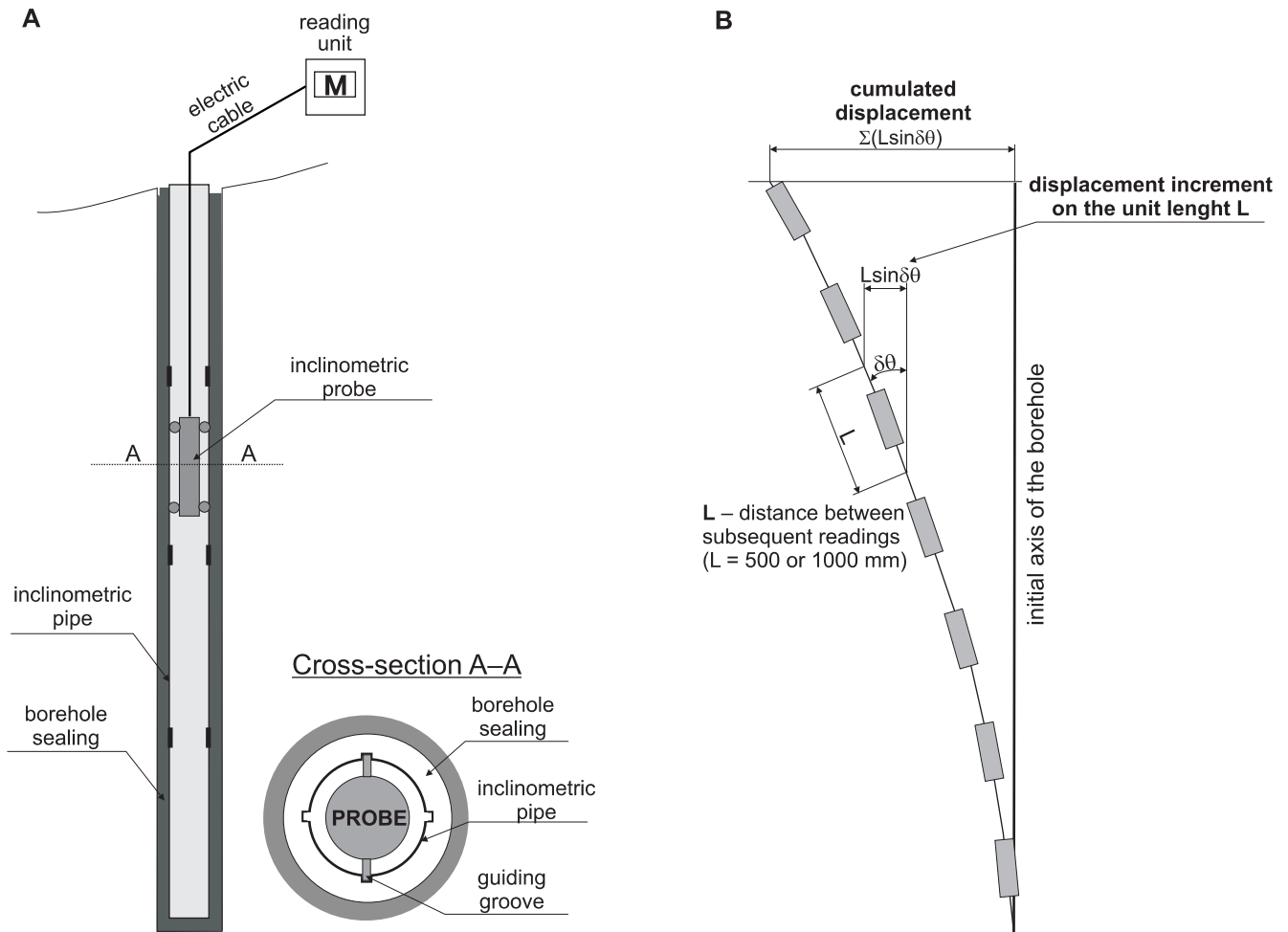
Fig. 4. Principles of inclinometric measurements
