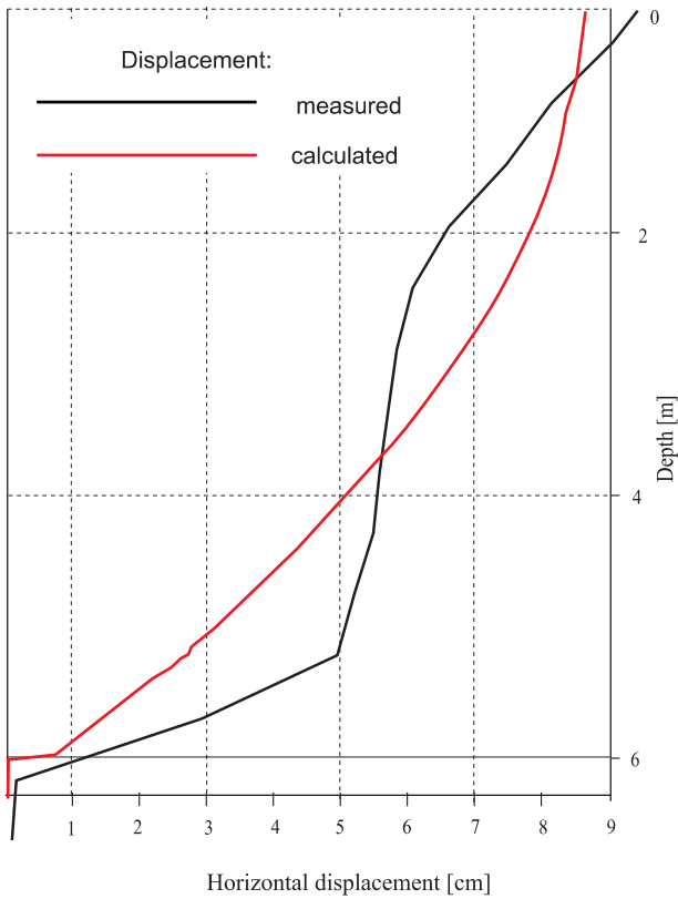
Fig. 11. Two-years horizontal displacement measured and calculated in K3 borehole
