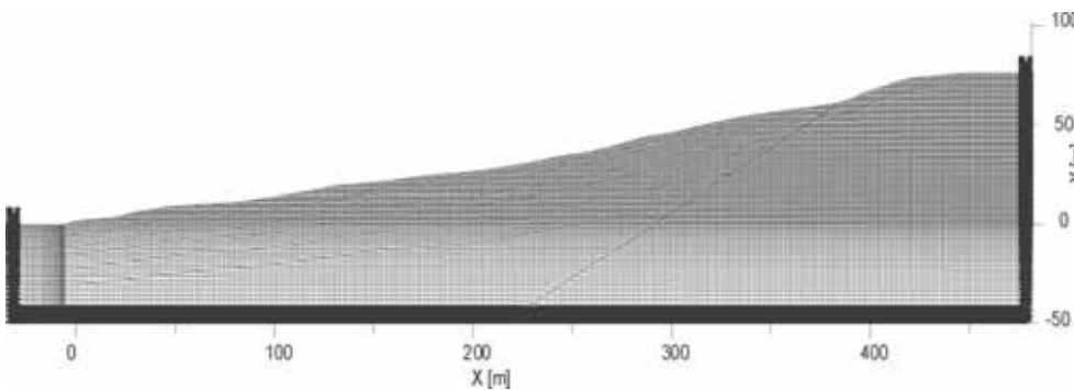
Fig. 7. Kawiry landslide — finite difference grid
