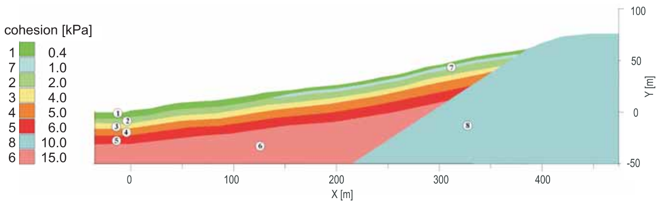
Fig. 9. Cohesion of geomechanical zones (layers) in the slope
