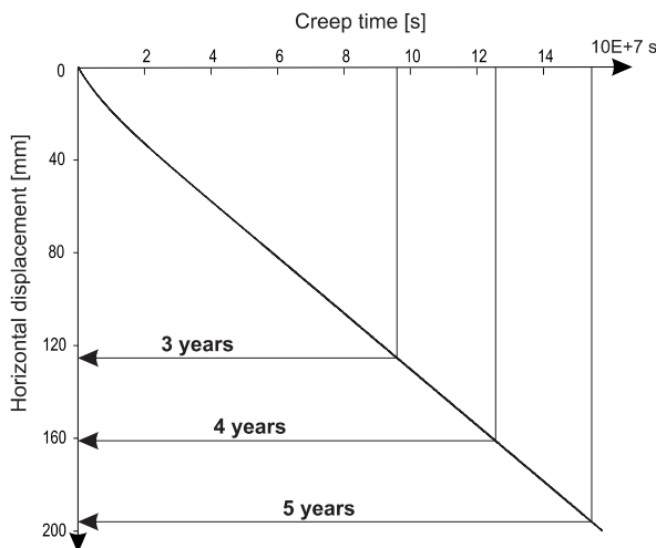
Fig. 12. Predicted five-years horizontal displacement of the slope
