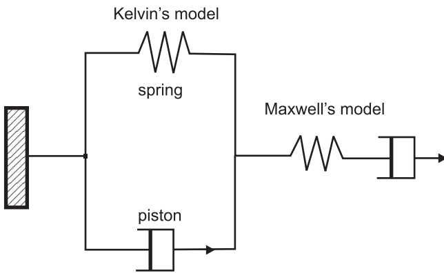
Fig. 8. Scheme of Burger's model
