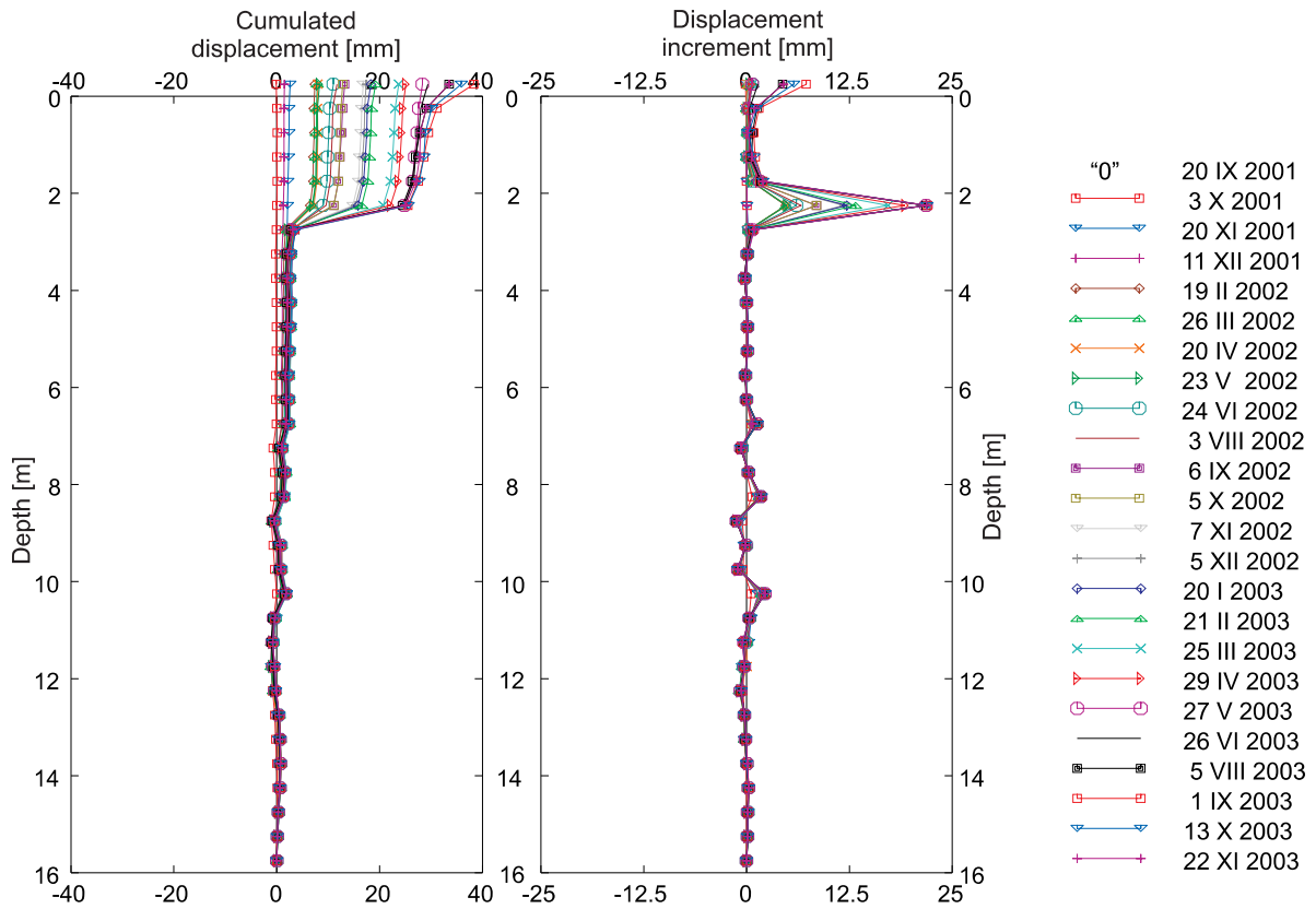
Fig. 5. Displacement curves of K1 borehole
