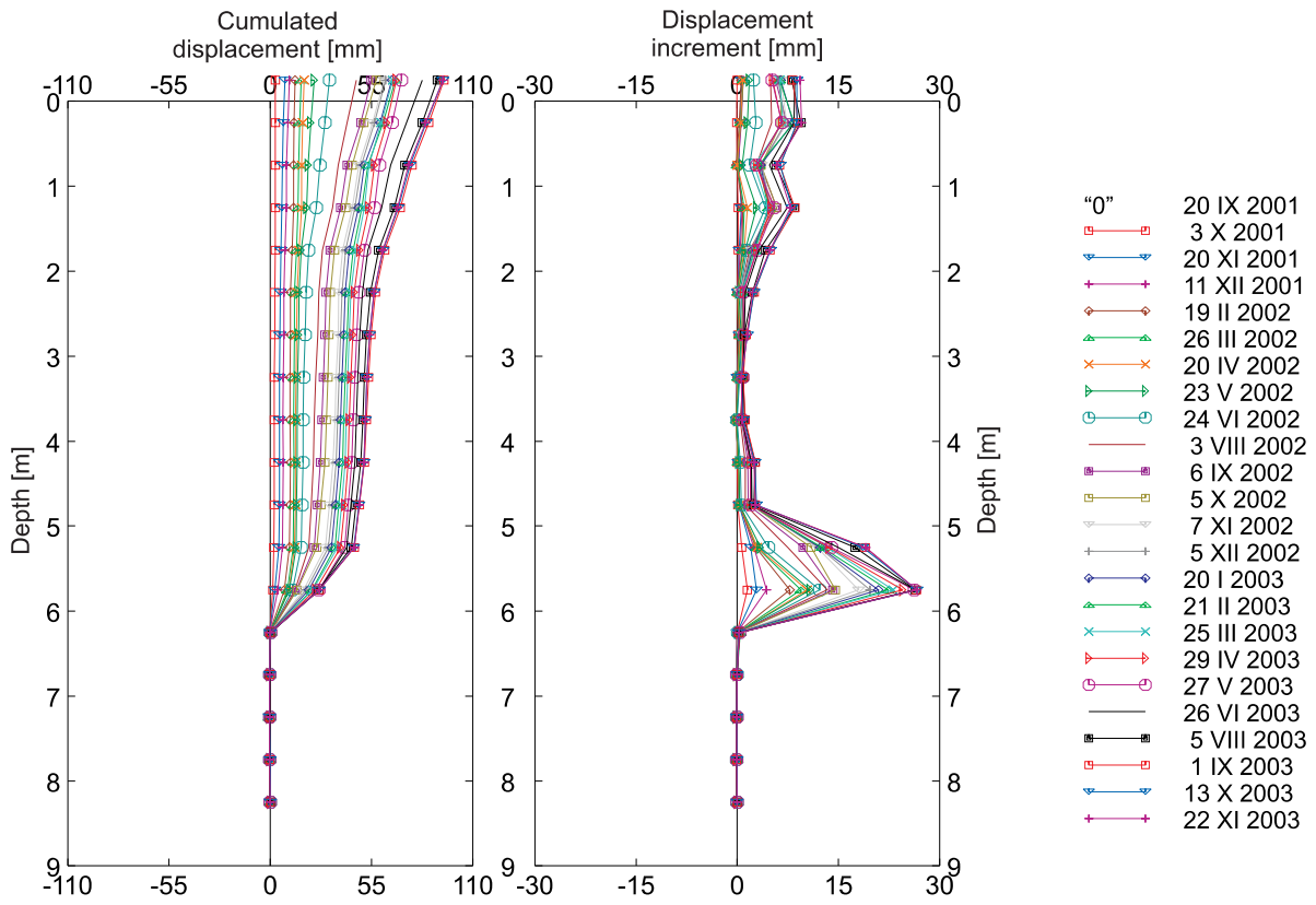
Fig. 6. Displacement curves of K3 borehole
