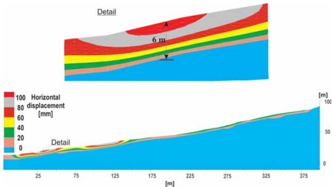
Fig. 10. Horizontal displacement of the slope, as an effect of two-years creep
