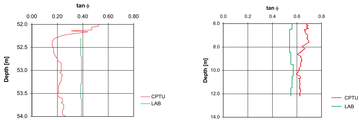
Fig. 9. Prediction of friction angle tangent for Polish and Norwegian clays from CPTU and laboratory tests
