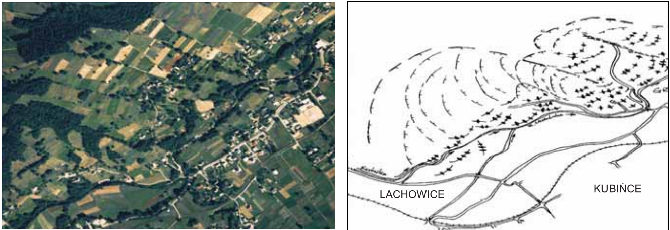
Fig. 13. Lachowice landslide aerial photo (1998) before the main slide occurred (2001) with sliding area interpretation
