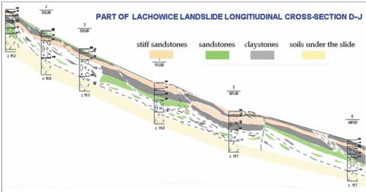
Fig. 11. Ground penetration radar interpretation, Lachowice landslide
