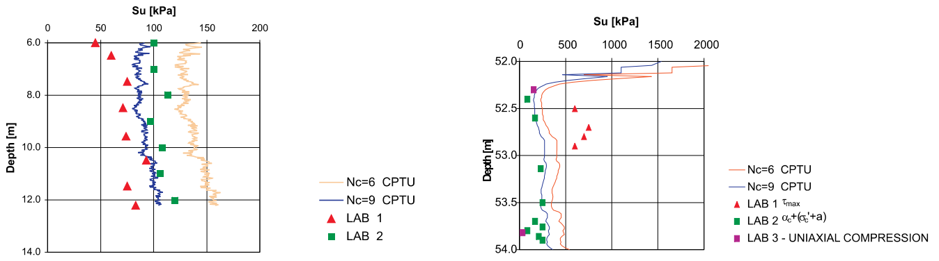
Fig. 6. Prediction of undrained shear strength for Polish and Norwegian clays using bearing capacity theory ( N_c = 6-9 ).
