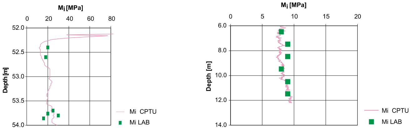
Fig. 8. Prediction of compression moduli in overconsolidated stress range for Polish and Norwegian clays from CPTU and laboratory tests
