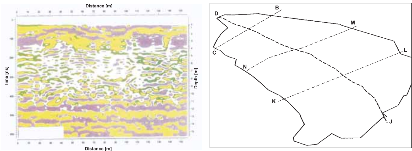
Fig. 10. GPR measurements, Lachowice, Carpathian Mountains
