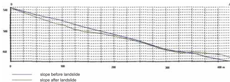
Fig. 14. GPS measurements on Lachowice landslide, comparison of slope profile before and after the main slide
