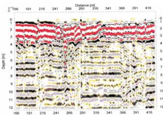
Fig. 12. Landslide in Wapienne, results of ground penetration scanning
