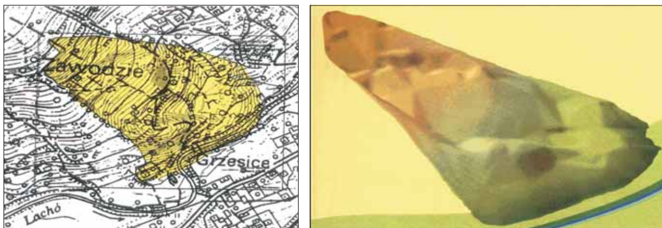
Fig. 15. GPS measurements on Lachowice landslide, 3D slide model
