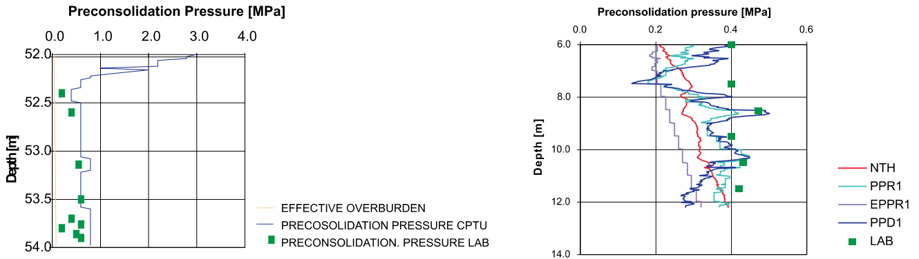
Fig. 7. Prediction of preconsolidation pressure for Polish and Norwegian clays from CPTU using different approaches and laboratory tests
