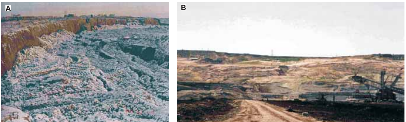
Fig. 2. Landslides in Polish open-cast mines
