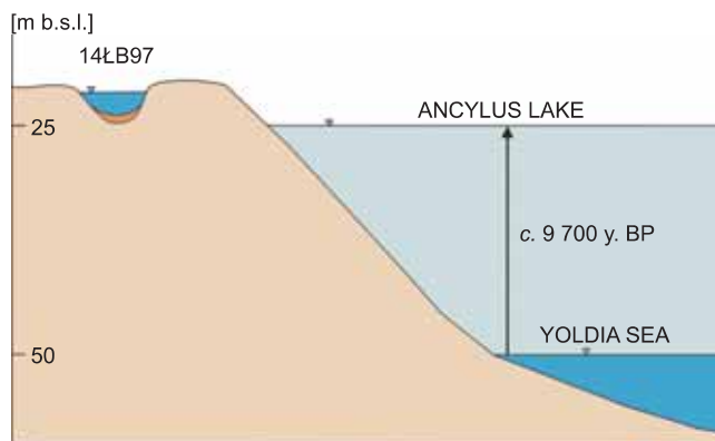
Fig. 10. Sketch of the discussed site and its vicinity during transgression of the Ancylus Lake
