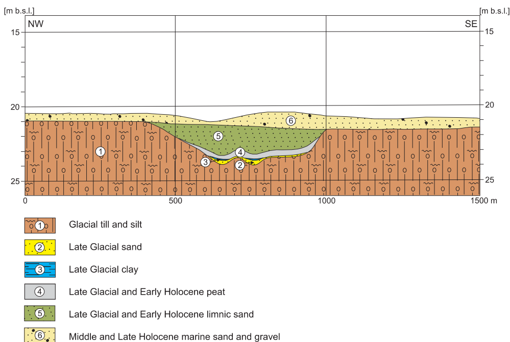
Fig. 6. Schematic geological cross-section along the investigated site
