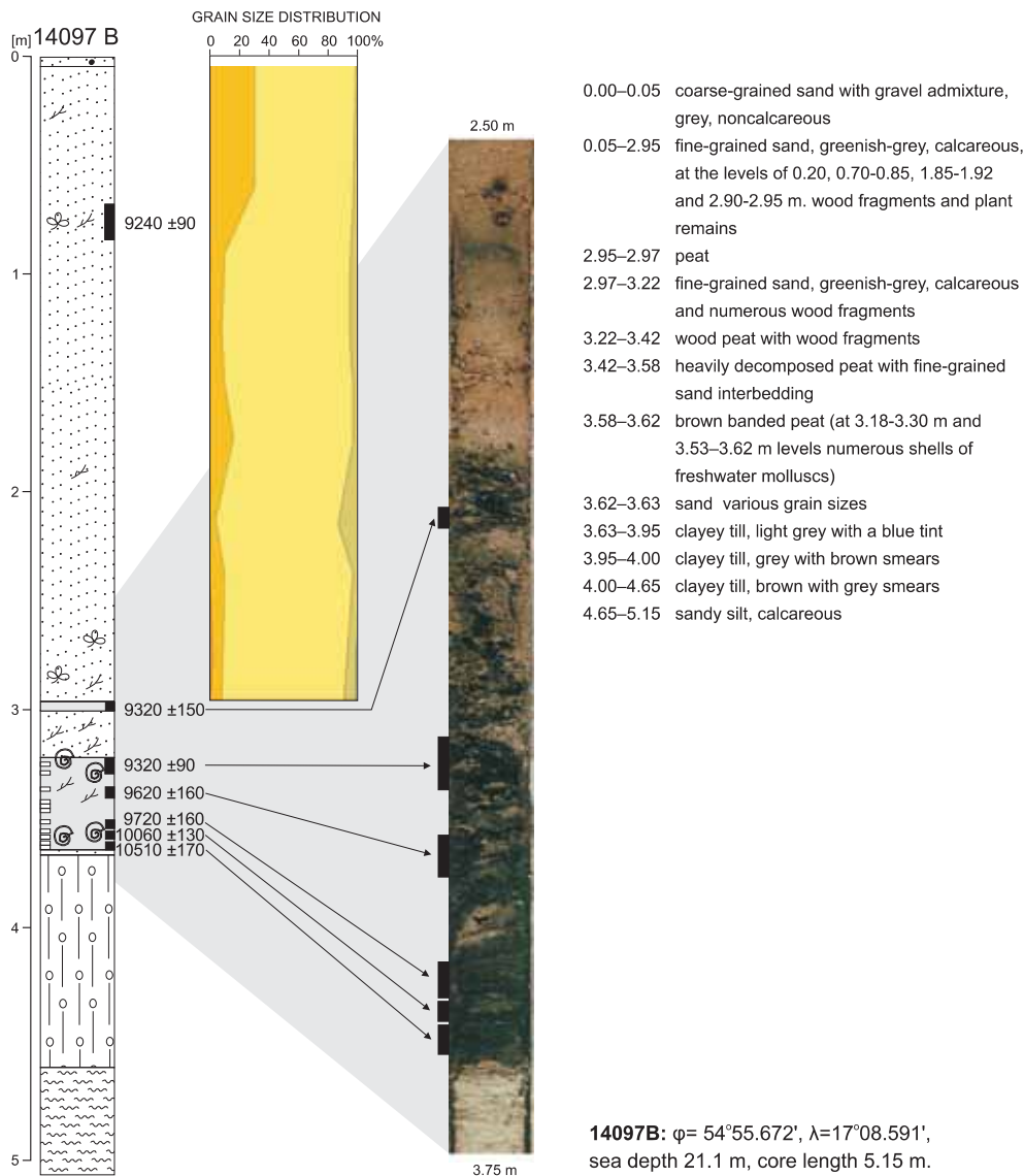
Fig. 5. Grain size distribution of sedimentary core 14097 B For explanation see Fig. 3
