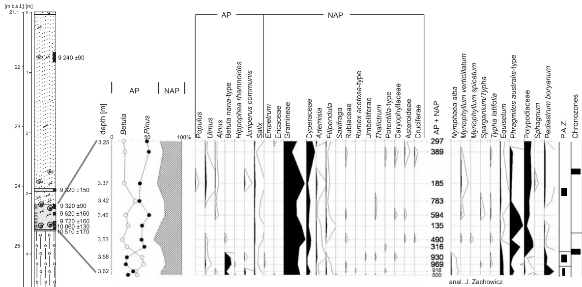
Fig. 7. Pollen diagram of sediments from core 14097 B (for explanation see Fig. 3)
