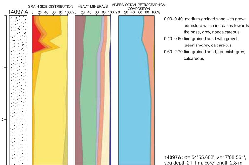
Fig. 4. Grain size distribution and mineralogical composition of sedimentary core 14097 A
