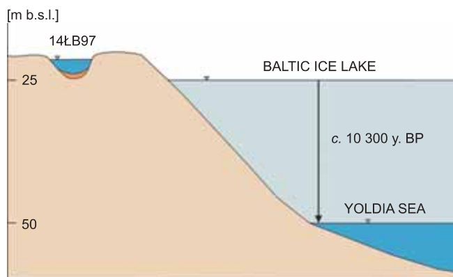
Fig. 9. Sketch of the discussed site and its vicinity during regression of the Baltic Ice Lake
