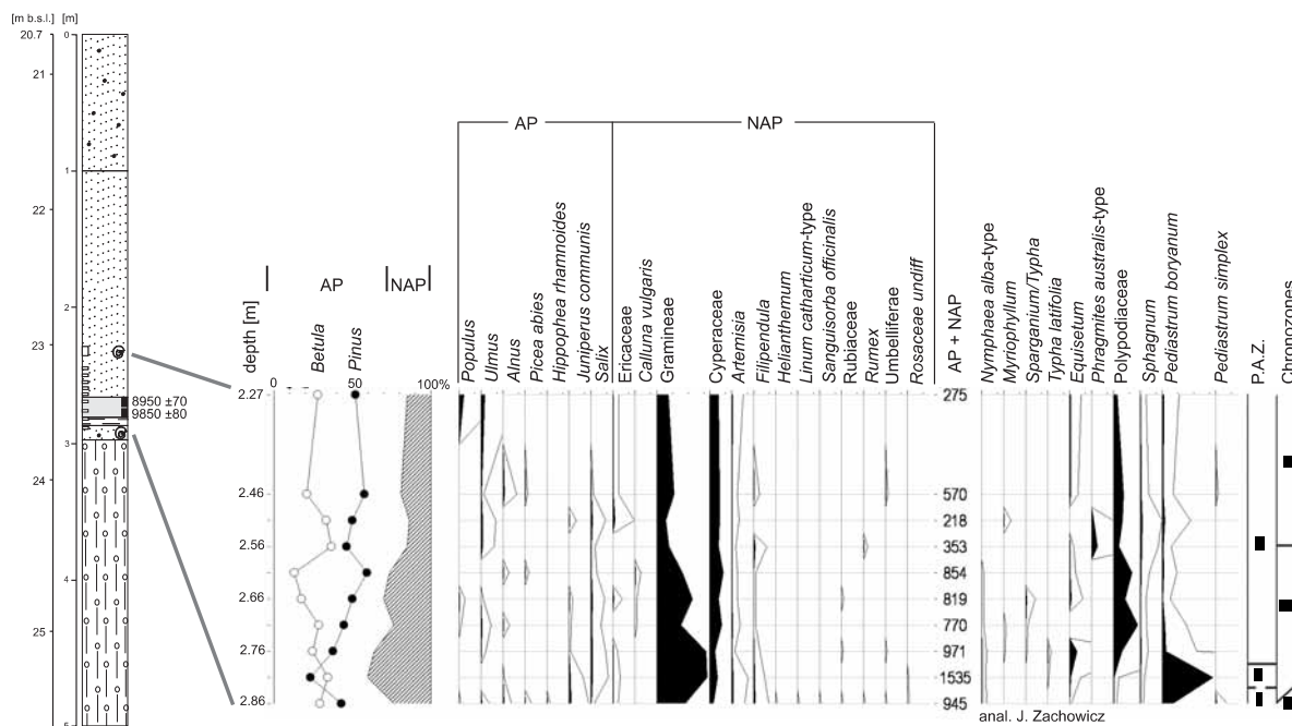
Fig. 8. Pollen diagram of sediments from core 14097 (for explanation see Fig. 3)
