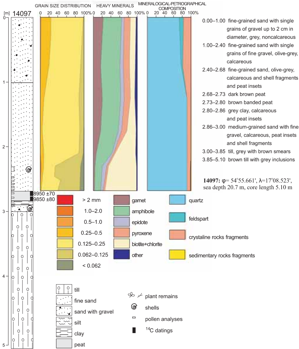
Fig. 3. Grain size distribution and mineralogical composition of sedimentary core 14097
