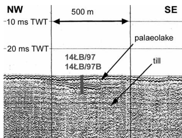
Fig. 2. Seismoacoustic profile (boomer record) across the investigated site
