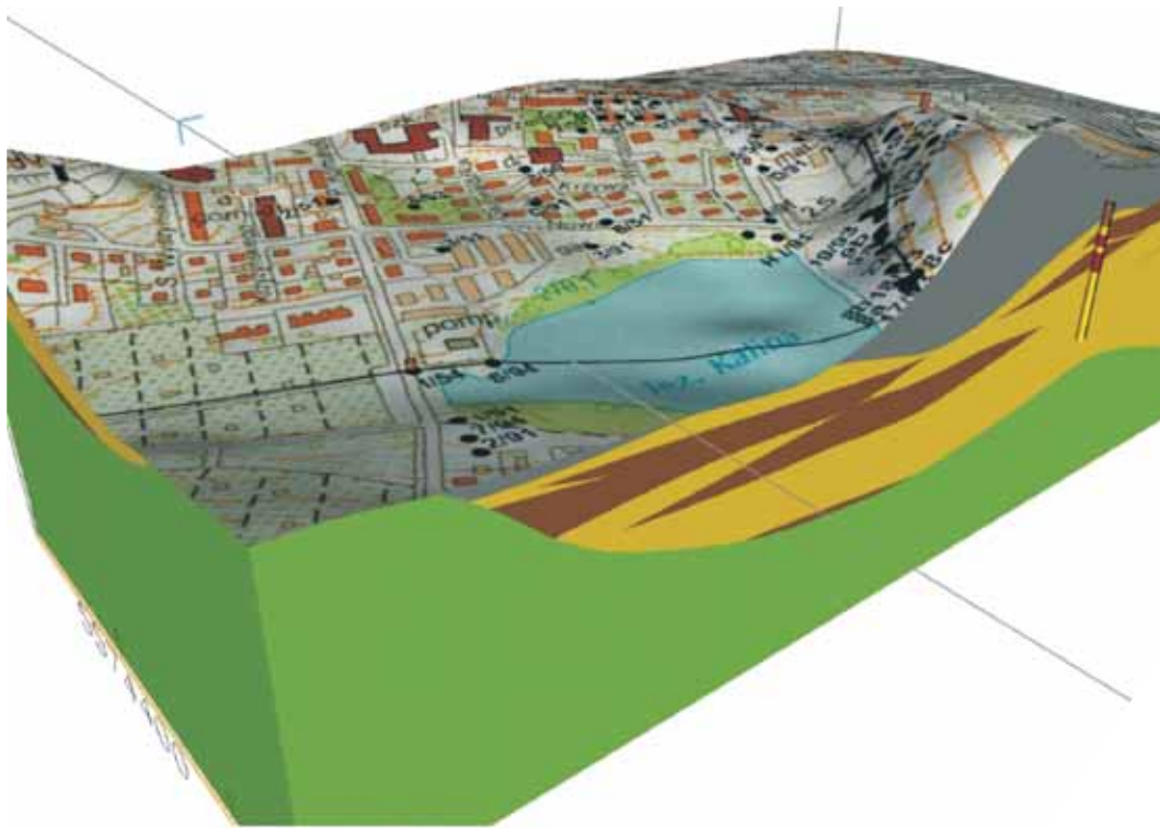
Fig. 4. Model geological cross-section (WE direction)
