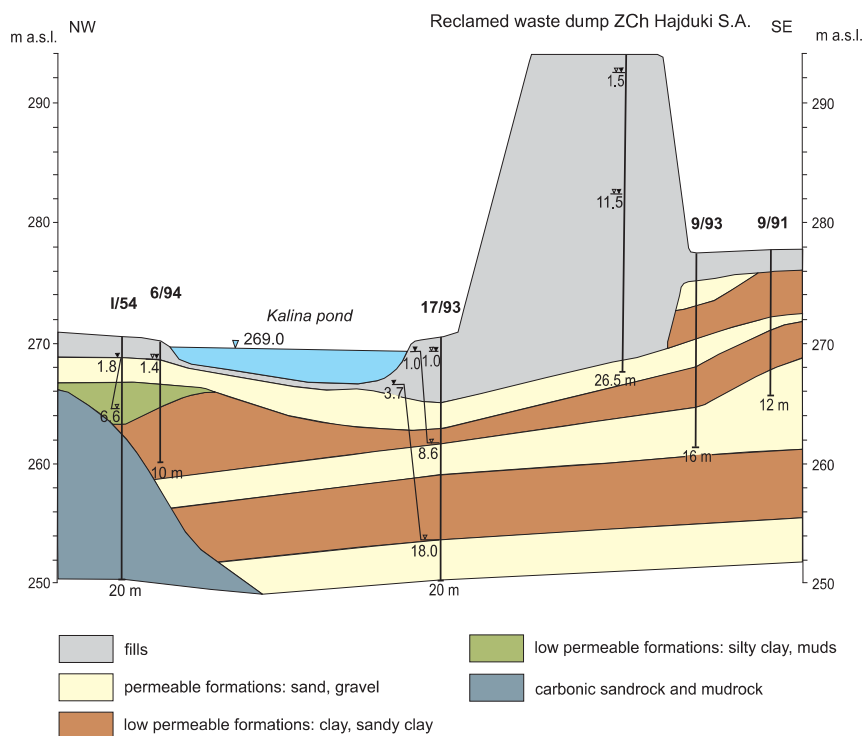
Fig. 1. General cross-section of the Kalina pond and waste dump
