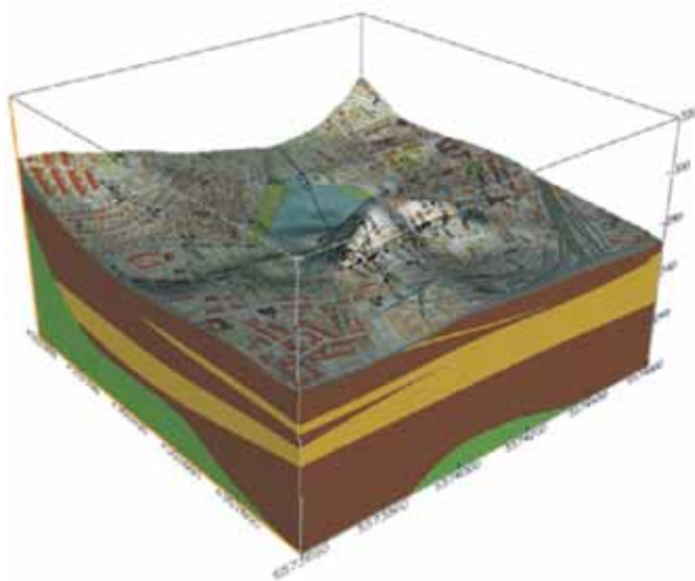
Fig. 3. General view of geological structure model with the terrain map overlain
