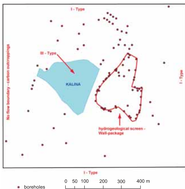
Fig. 6. Boundary conditions for groundwater flow simulations
