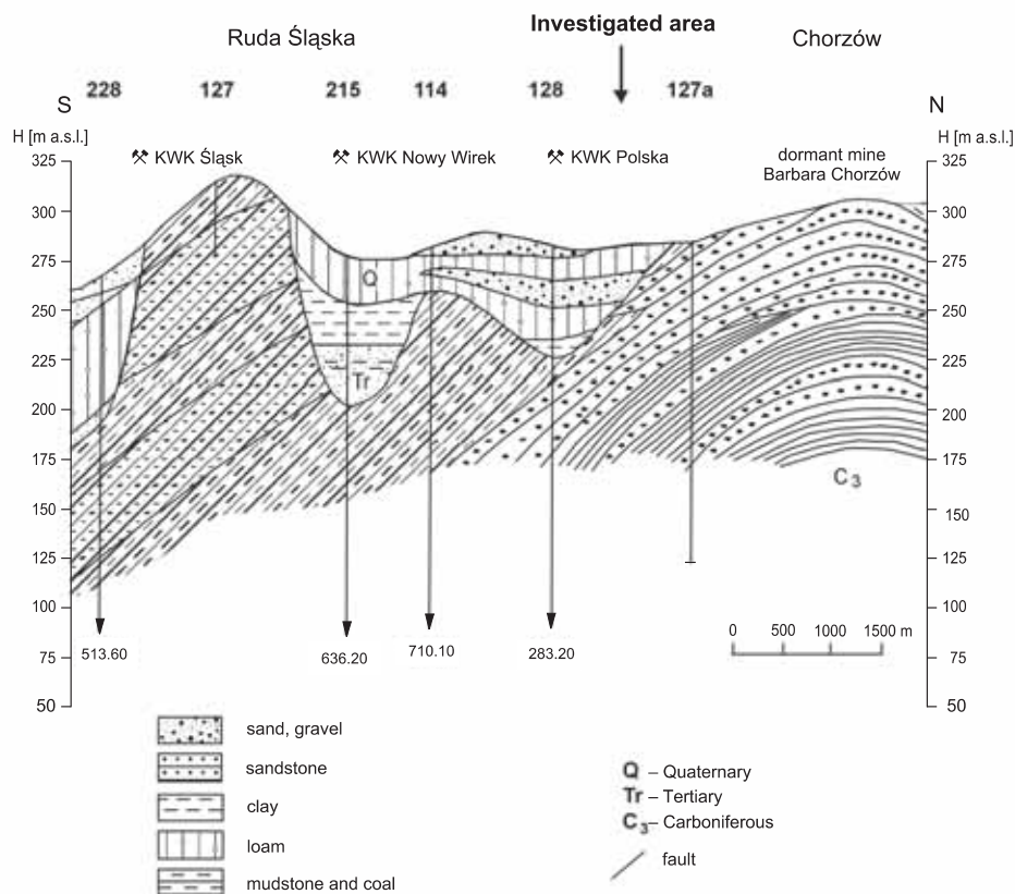
Fig. 2. Regional hydrogeological cross-section (Chmura, Wagner, 1997)
