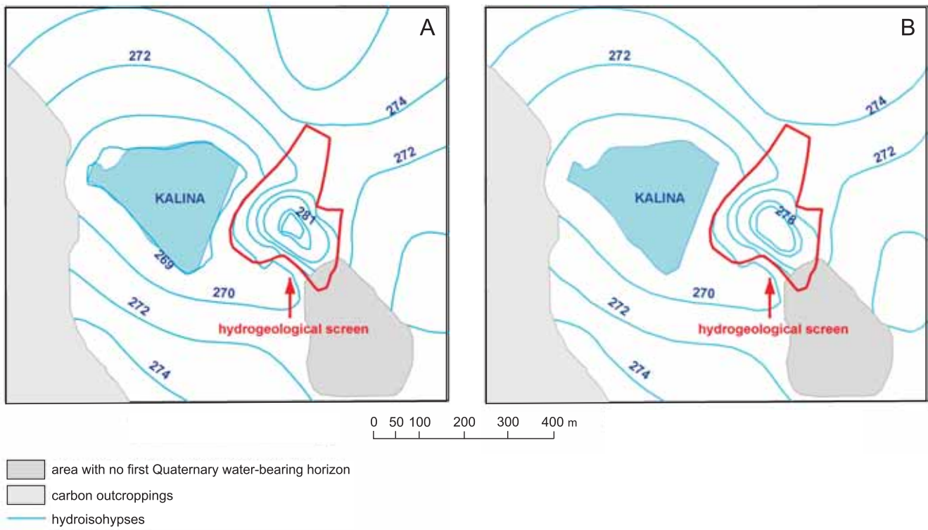
Fig. 5. A — Interpreted surface of water table of the first water-bearing layer; B — Surface of the first water-bearing horizon water table – simulation results
