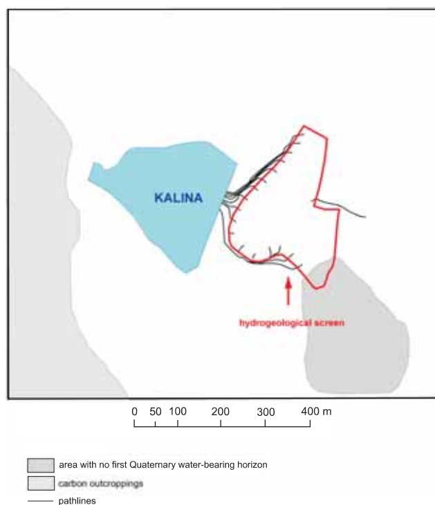
Fig. 7. Water pathlines — the distance between the arrows represents 1 year
