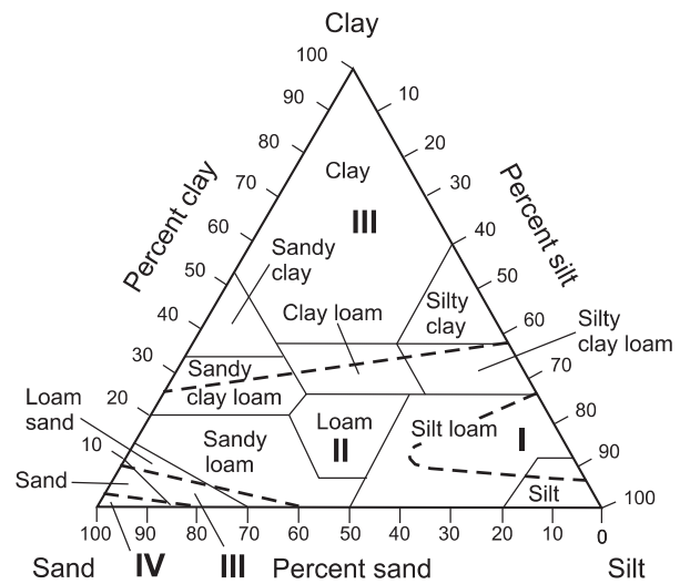
Fig. 15. Reclamation suitability categories of grounds I–IV (Chwastek, Żuławski, 1981) against USDA soil science classification (Sara, 2003)
