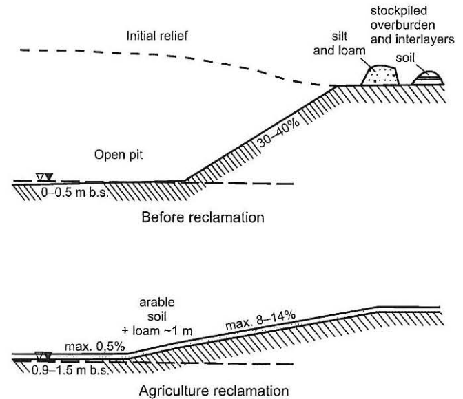
Fig. 10. Scheme of ground balance during technical reclamation of a pit for agriculture use
