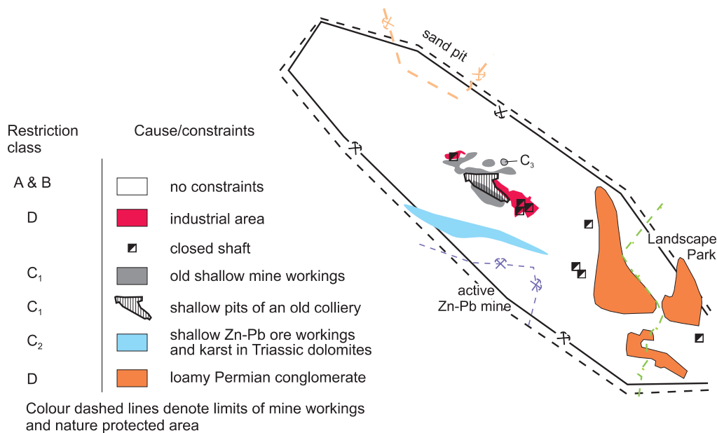
Fig. 16. Example of construction ground categorisation of an old mining area, Siersza, Poland (Popiolek, Ostrowski, 2001)
