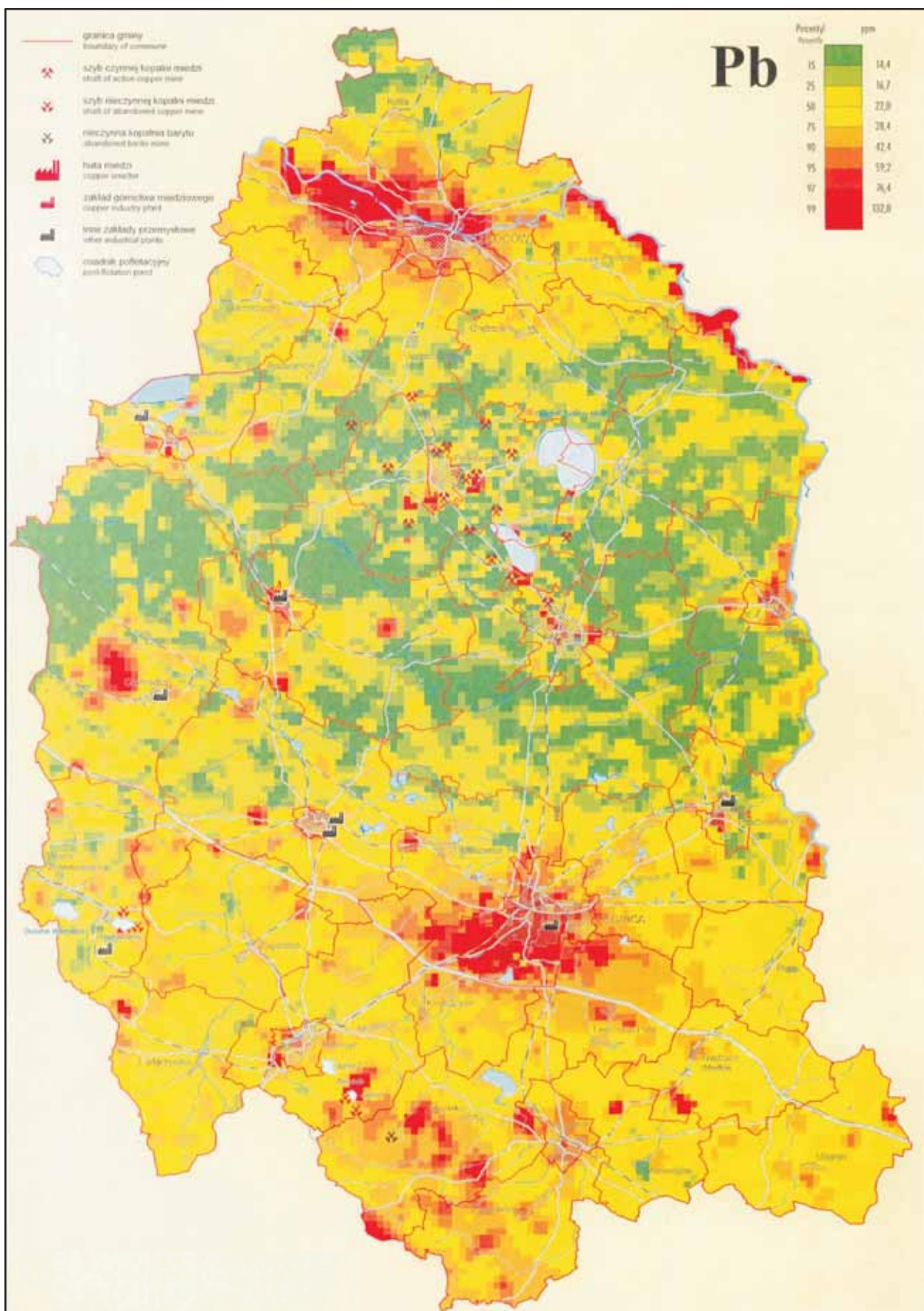
Fig. 2. Lead content in soils (after Lis et al. , 1999)
