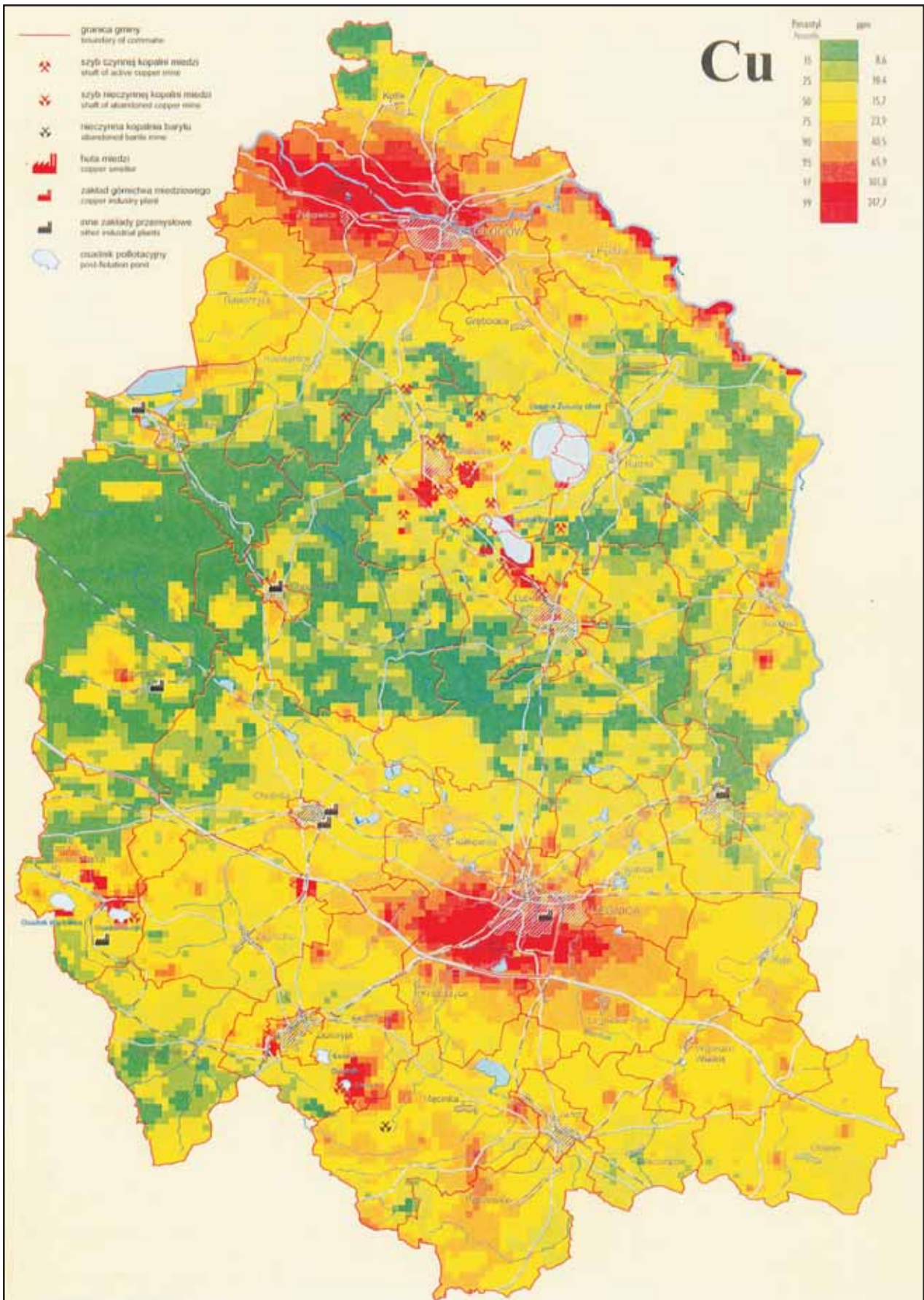
Fig. 1. Copper content in soils (after Lis et al. , 1999)
