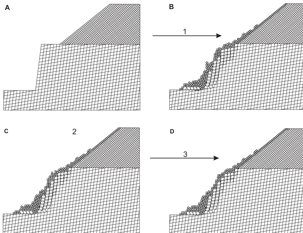
Fig. 6. Selected stages of the landslide development
