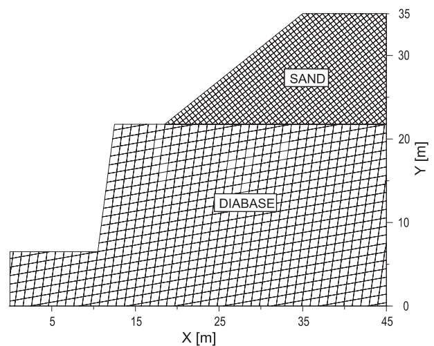
Fig. 5. Cross-section for the numerical simulation of the landslide movement
