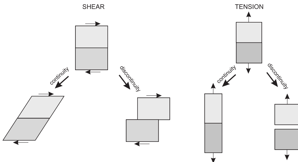
Fig. 3. Comparison between the behaviour of continuous and discontinuous models
