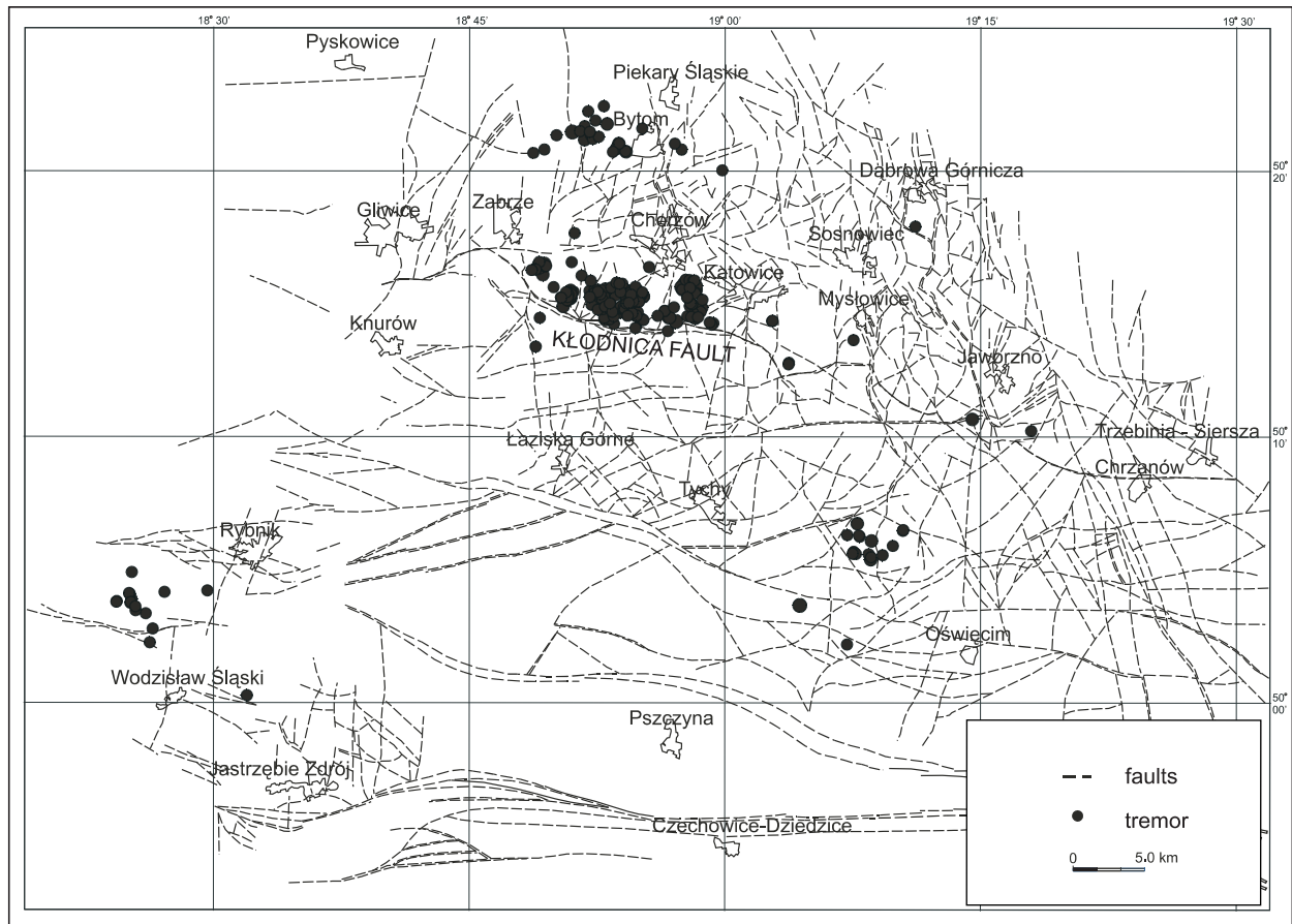
Fig. 3. The USCB tectonics and epicentres of high-energy tremors ( >10^7 J) during the 1985–2004 period
