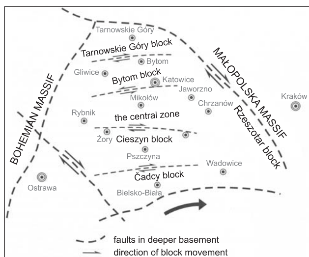
Fig. 2. The USCB and faults in the deep Precambrian bedrock Kotas, 1985)
