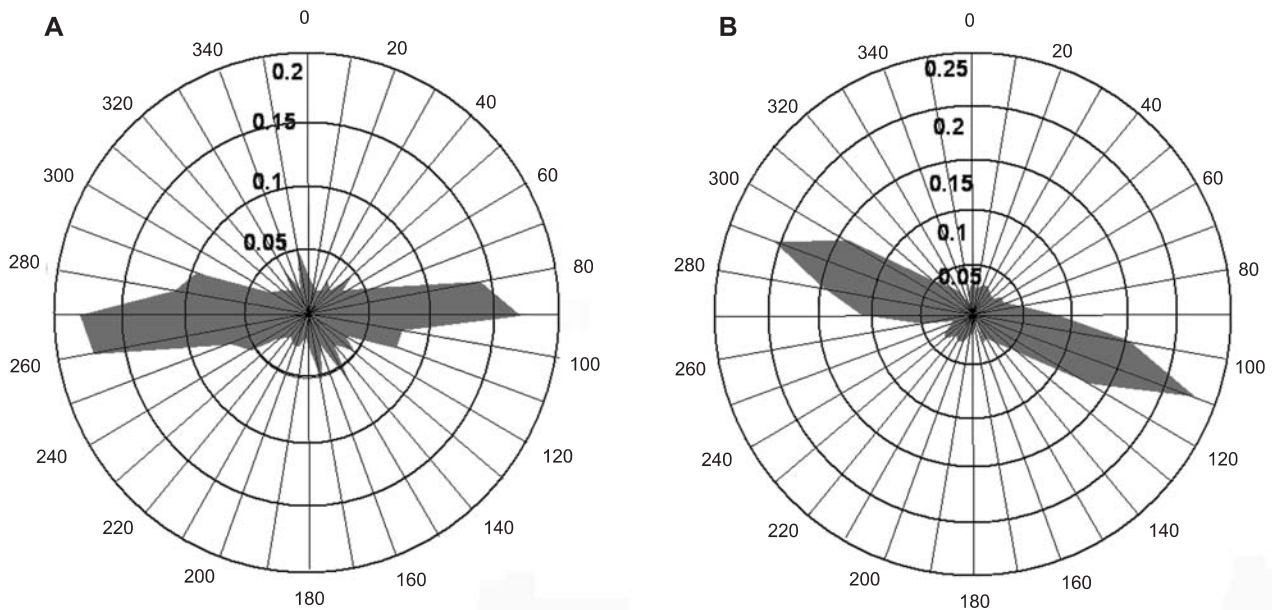
Fig. 1. Distribution of vectors directions, connecting two tremors occurring in the same regions
