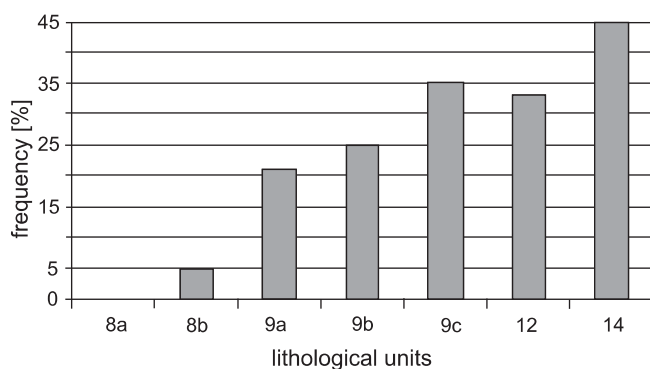
Fig. 3. Area frequency statistics of landsliding for different lithological units
