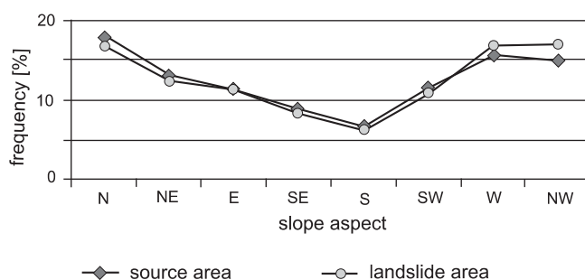
Fig. 5. Area frequency statistics for landslides distribution (source area and total area) caused by slope factor
