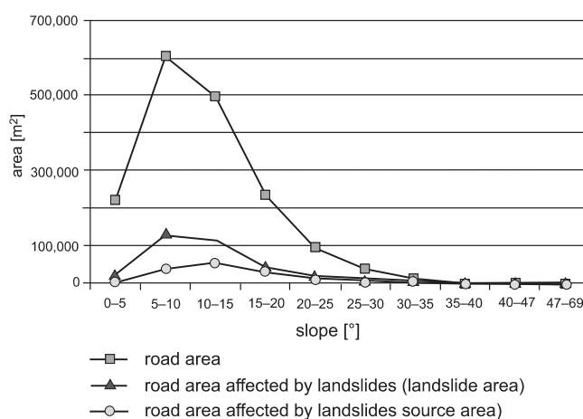
Fig. 7. Extent of roads area affected by landslides source areas (circles) and by landslides total areas (triangles), versus slopes angle. Total extent of roads area versus slopes angle (squares) is also shown
