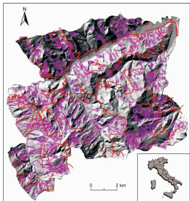
Fig. 1. Landslides distribution (in violet) and roads network (red) superimposed over a shaded digital elevation model (DEM)
