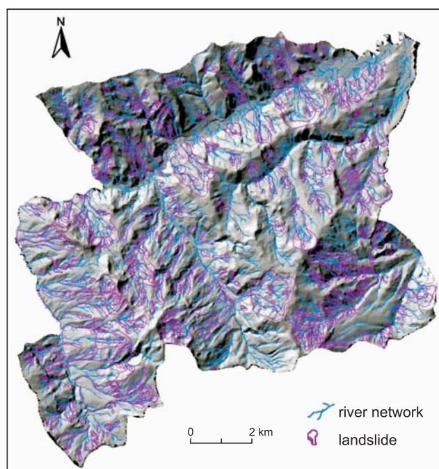
Fig. 6. Landslides distribution and watercourse network data superimposed on a shaded digital elevation model
