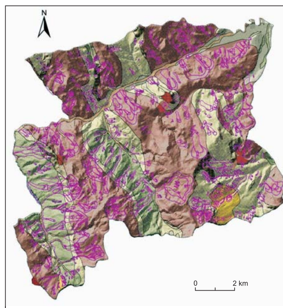
Lithological units:
