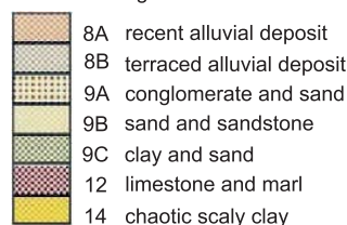
Lithological units:
